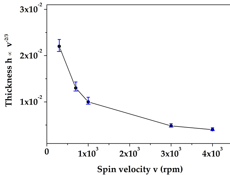
Figure 2.5: Spin curve showing the variation of the film thickness as a function of spin velocity.
