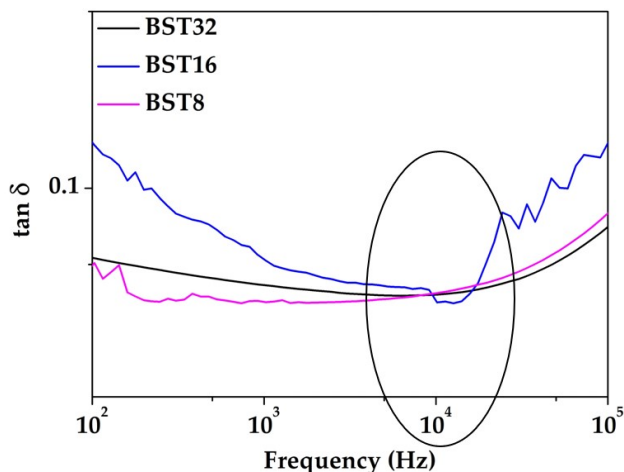
Figure 5.12: Dissipation curve for the three BST diluted samples.
