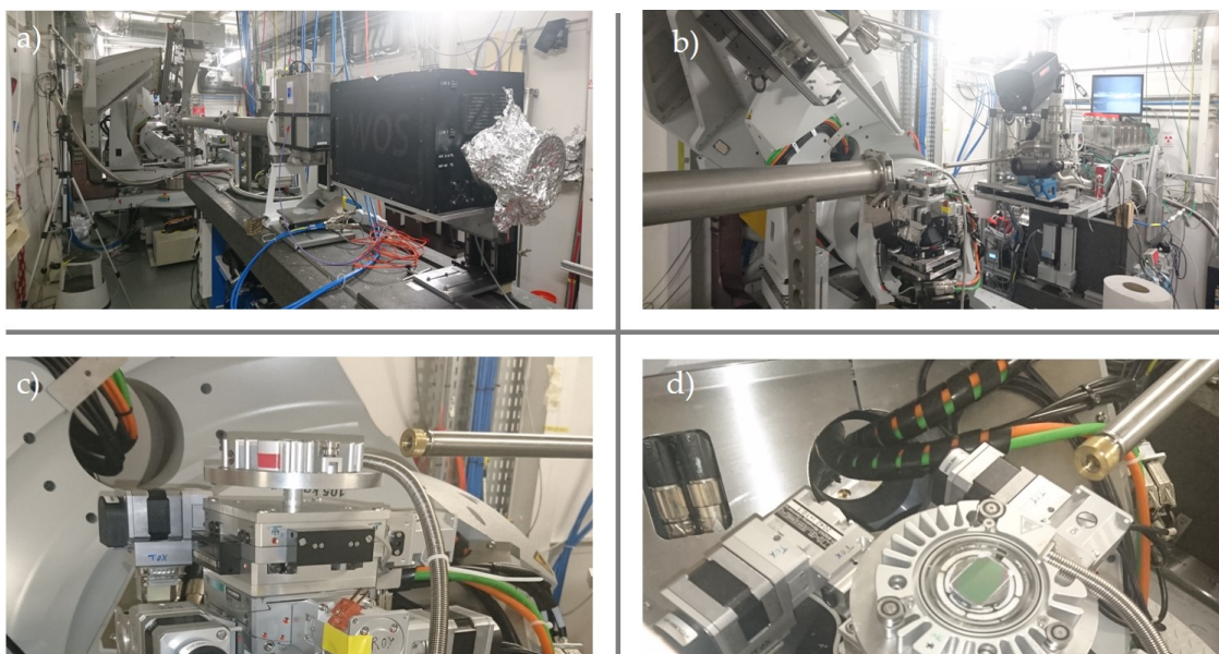
Figure C.1: GISAXS setup images : (a) Overview on the whole setup, (b) detectors and cameras, (c) close-up on the sample holder and (d) close-up on the sample.
