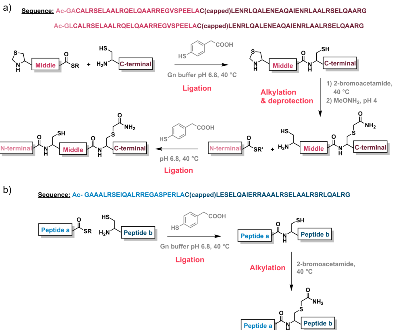
Scheme 4.1. Reaction pathways for the synthesis of 'strand +14' and 'strand +7'. a) Synthesis of both 'strand +14, GAC' and 'strand +14, GLC' using a one-pot three-segment ligation strategy. b) Synthesis of 'strand +7' common to both analogues by NCL. The shown sequence corresponds to the sequence in which Asn residues were replaced by either arginine or serine due to synthetic issues.
