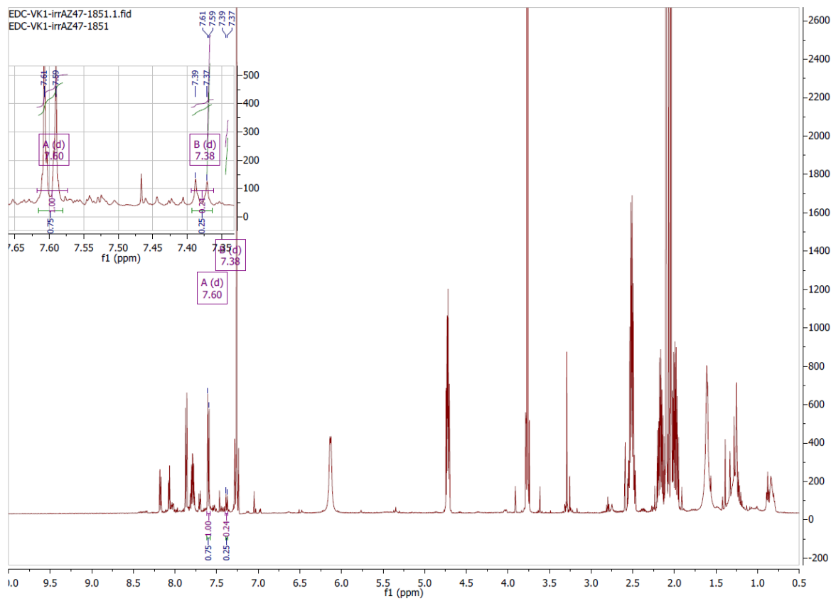
Figure S.3. 3. NMR spectra for photoreaction between nMet and probe 7
