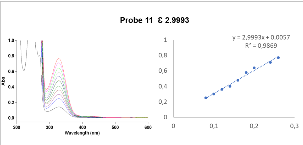
Figure S.3. 6. US-Vis spectrometry indicating \epsilon_{\text{max}} and \lambda_{\text{max}} of probe 9 (a), probe 10 (b) and probe 11 (c) in 20% ACN
