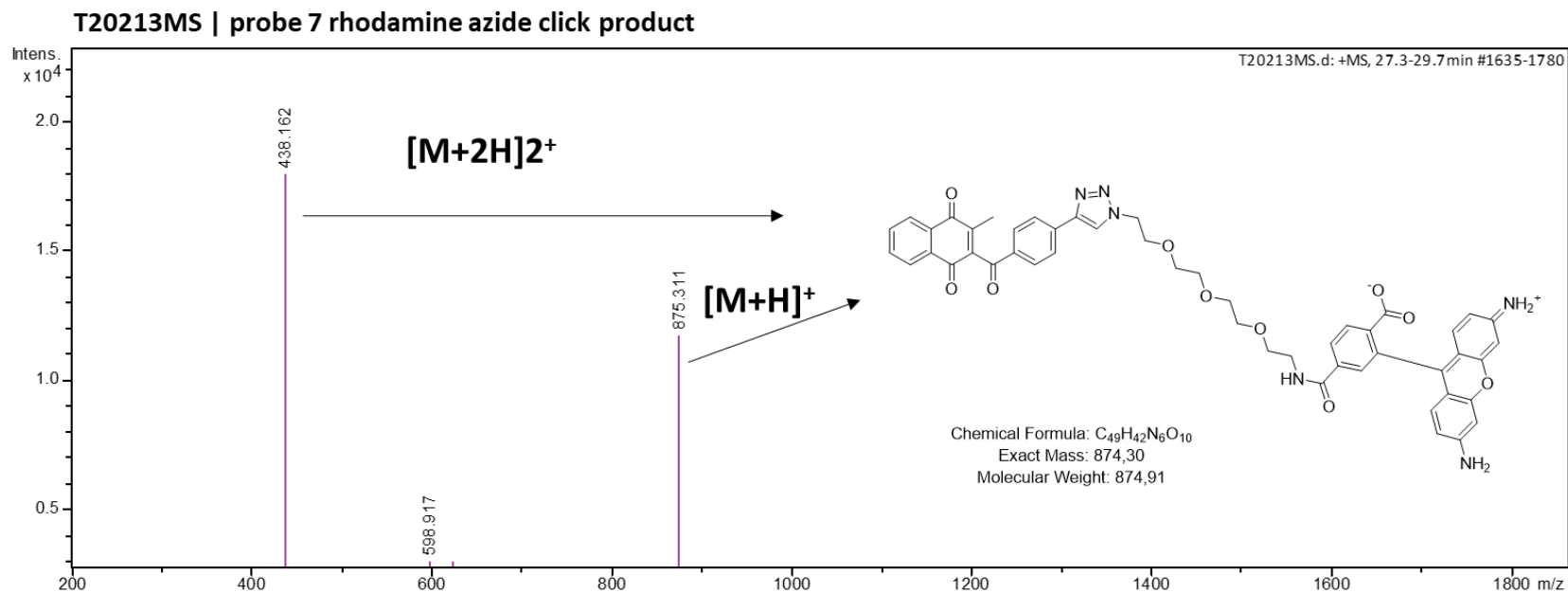
Figure S.3. 18. HPLC-MS analysis of probe 7-RA click product. For probe 7 click reaction, calculated mass of click product is 874.30 and we observed it's hydrated form with mass 875.311 and m/z = 1/2 with mass 438.162 at Rt 27.6 and 29.1 minutes for 2 isomers. RA with 575.22 was observed at Rt.27.6 and 29.1 for two isomers.
