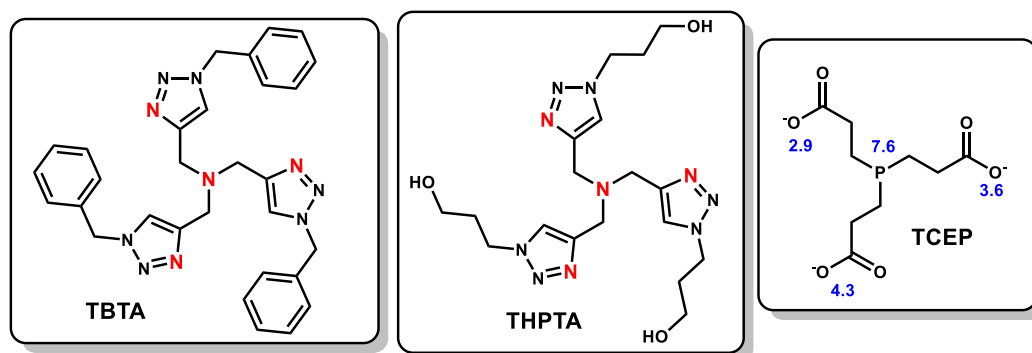
Figure 4. 8. Chemical structures of TBTA/THPTA (the red colour indicates the Cu(I) binding units) and of TCEP ( pK_a values are given in blue).
