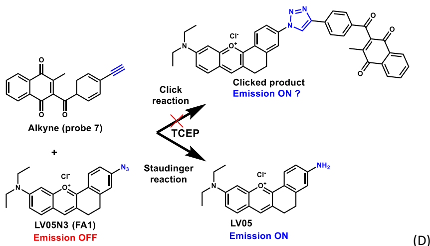
Figure 4. 9. Feasibility of ligand TBTA and reductant NaASc for flavylum azide click reaction. (A) Effect of ligand TBTA and NaASc reductant used in excess on FA1 in aqueous conditions with ~ 3% DMF. 1.
