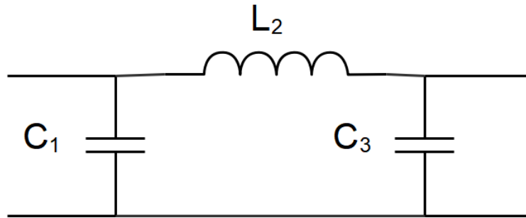
Figure 4.4 – Single port ladder type network-third-order ladder type low-pass network
