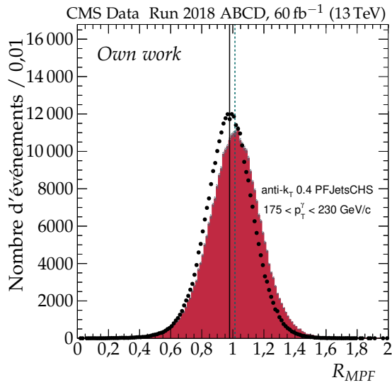
(a) Avant correction (figure 3.18c).
