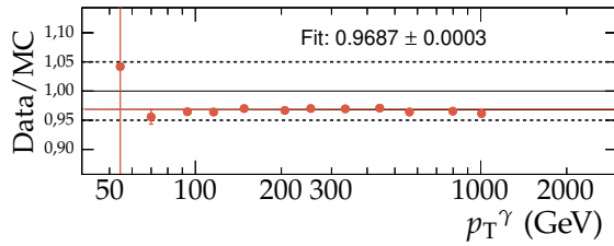
(a) |\eta^{jet}| < 1,3 .
