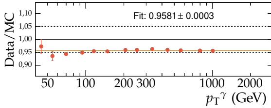
(a) |\eta^{jet}| < 1,3 .
