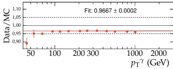
(a) |\eta^{jet}| < 1,3 .
