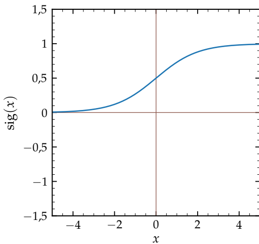
(c) Sigmoide.
