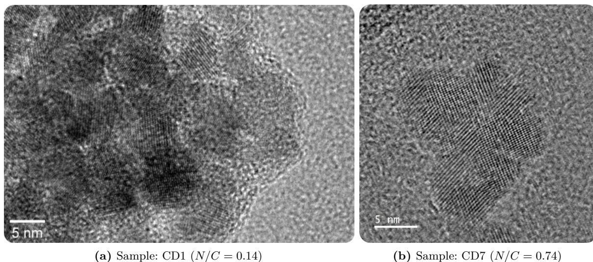
Figure 34 – High-resolution transmission electron microscopy of the studied samples, evidencing the shape and internal crystalline structure of the dots.
