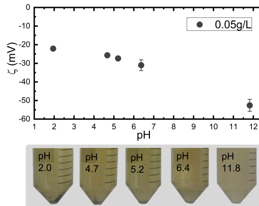
Figure 5. Top: Zeta potential as a function of the pH for the investigated N-CD sample in a concentration of 0.05 g/L. Bottom: Picture of the samples after two weeks in each pH, showing the reduction of precipitate amount with increasing pH.
