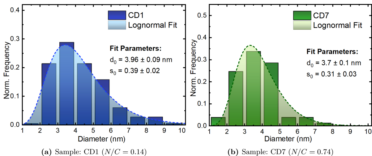
Figure 35 – Particle size histograms deduced from transmission electron microscopy images. The adjustment of the data was performed using the lognormal distribution presented in Equation 1.1 .
