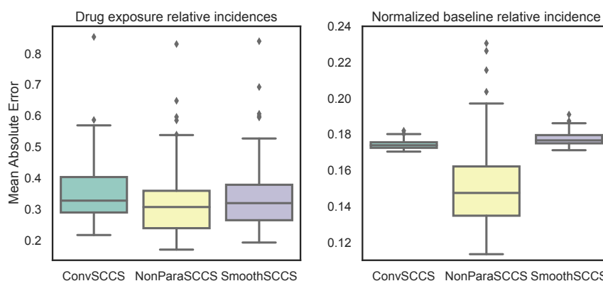
Figure II.4.1 – Simulations results using Set 1 or risk profiles (see Figure II.E.2) with m = 4000 . The boxplots represent the distribution of mean absolute error as defined in Section II.4.1, computed over 100 simulated populations. Left: MAE distribution of the drug exposure relative incidences. Right: MAE distribution of the baseline relative incidences, constrained so that their integral is equal to one.
