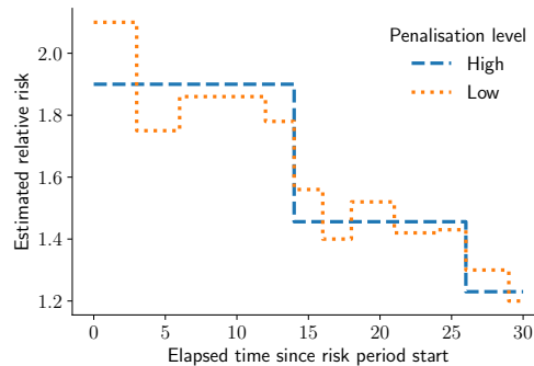
Figure III.2.2 – Illustration of the Total Variation penalisation effect. Assuming a risk period starting at 0 and lasting for 30 days, ConvSCCS will estimate a 30-day piece-wise constant relative risk curve. The total size of the jumps is controlled by the level of Total Variation penalisation. A low (resp. high) level of penalisation results in more (resp. less) detailed relative risk curves, illustrated by the orange small dashes (resp. blue long dashes) curve. The aim of the model fitting algorithm is to reach a good balance between the detail level and the smoothness of the estimated relative risk curves.
