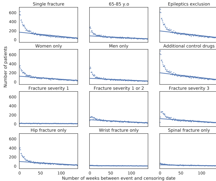
Figure III.C.1 – Robust regression (Huber) of censoring times versus event times. The horizontal axis represents the number of weeks between event date and censoring date, and the vertical axis the corresponding number of patients. Markers represent the patient counts corresponding to each week bucket, and the solid line represents the robust regression line. The closer the points are to the regression lines, the more likely the assumption of independence between event dates and observation dates is. Patients above the regression line are susceptible to have a death event correlated with a fracture event. In the all-fracture (reference) study featured in this paper, 9300 patients (7.35%) death event might be considered to be correlated to their fracture times. Note that the negative gradient of the regression line is explained by the events repartition in the study: if events are assumed to be uniformly distributed across the four years, there are fewer chances to observe events separated by 200 weeks than 25 weeks.
