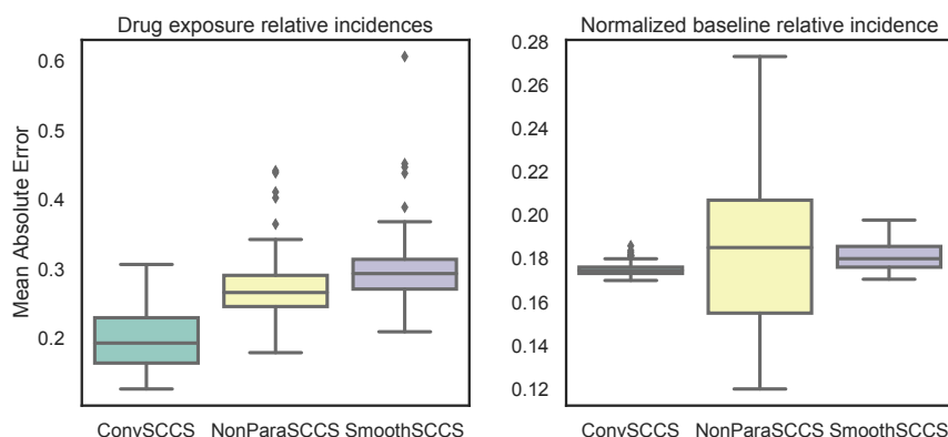
Figure 7 – Results on synthetic data using risk profiles illustrated in Figure 7) with m = 4000 cases. The boxplots represent the distribution of mean absolute error, computed over 100 simulated populations. Left : MAE distribution of the drug exposure relative incidences \theta . Right : MAE distribution of the baseline relative incidences \phi , constrained so that their integral is equal to one.
