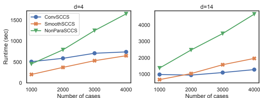
Figure 8 – Run times of ConvSCCS, SmoothSCCS and NonParaSCCS for 1000, 2000, 3000, 4000 cases. Left : run times on 4 features. Right : run times on 14 features. As SmoothSCCS and NonParaSCCS can only handle one feature at a time, we report the time required to fit them on each studied feature while ConvSCCS is fitted on all the features simultaneously. For each model, a fit includes cross-validation of the hyperparameters and estimation of confidence bands (see Chapter II for more details).
