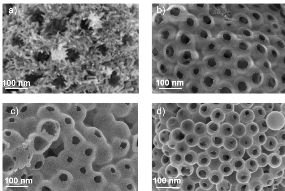
Figure 2.6 Comparison of SEM micrographs at 550° C between a) \text{IrO}_2^{10} , b) 10-Mo, c) 30-Mo and d) 50-Mo.
