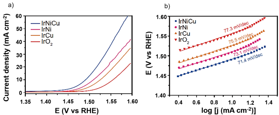
Figure 3.7 a) LSV curves for OER performance and b) Tafel plots of different iridium-based multimetallic alloy (taken and modified from 26 ).
