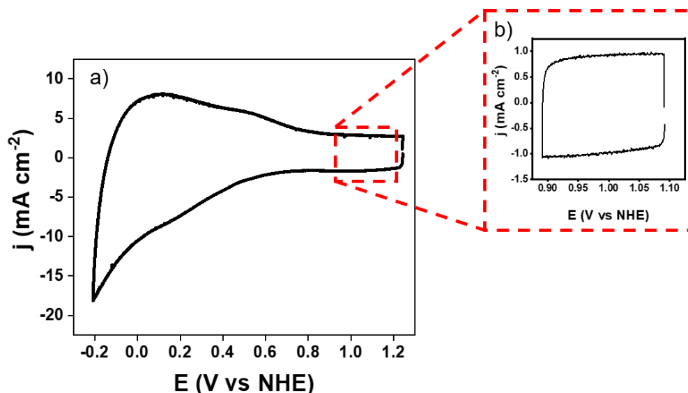
Figure 4.9 a) Cyclic voltammogram of 50-Mo@550 recorded at a scan rate of 25 mV s -1 in 0.1 M HClO 4 and b) zoom in non-Faradaic.
