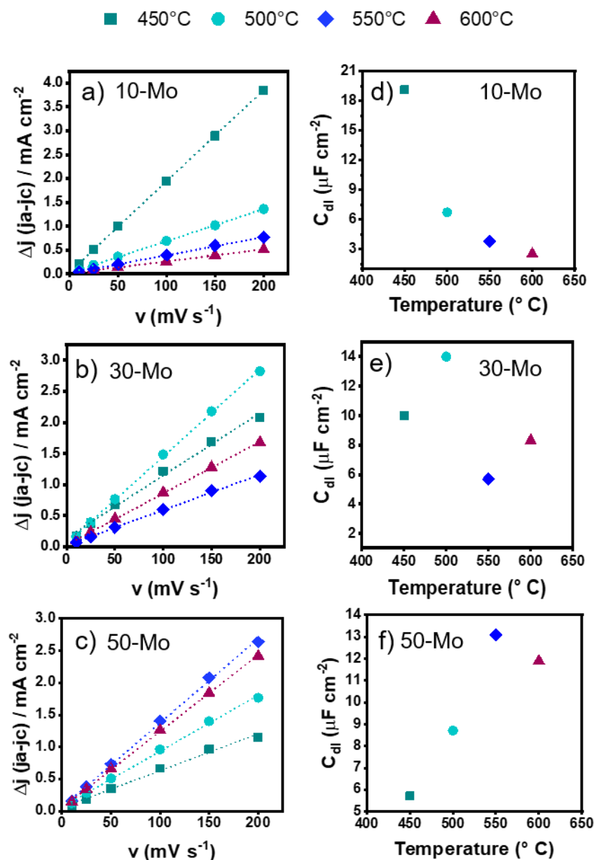
Figure 4.11 a, b, c) The difference between anodic and cathodic charging current density measured at 1.0 V vs NHE plotted as function of scan rate, and d,e,f) the evolution of the differential capacitance ( C_{dl} ) estimated from cyclic voltammograms experiments in the non-Faradaic region in 0.1 M \text{HClO}_4 ;
