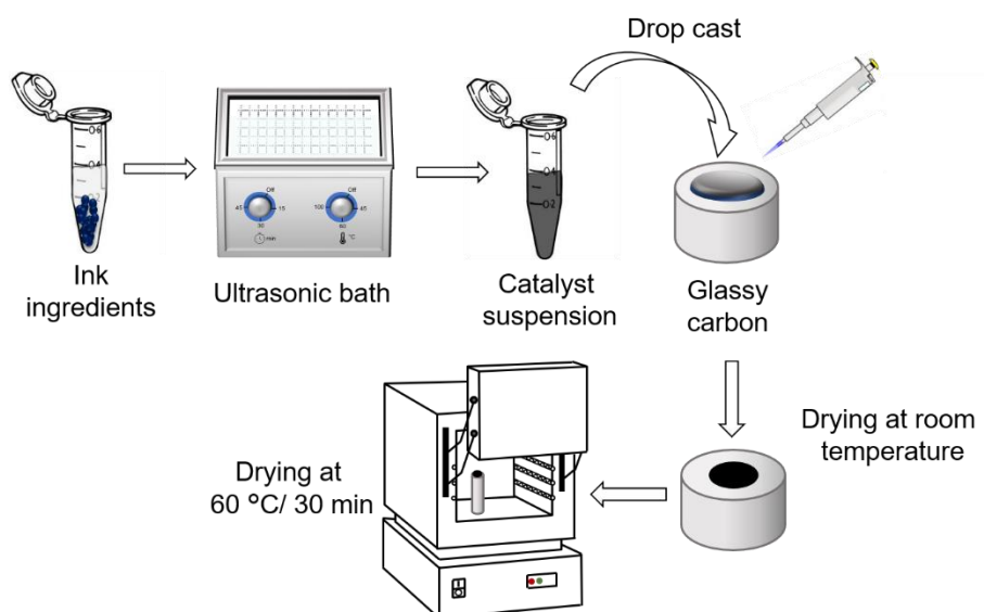
Figure 6.7 Schematic representation of the catalyst ink formation and drying
