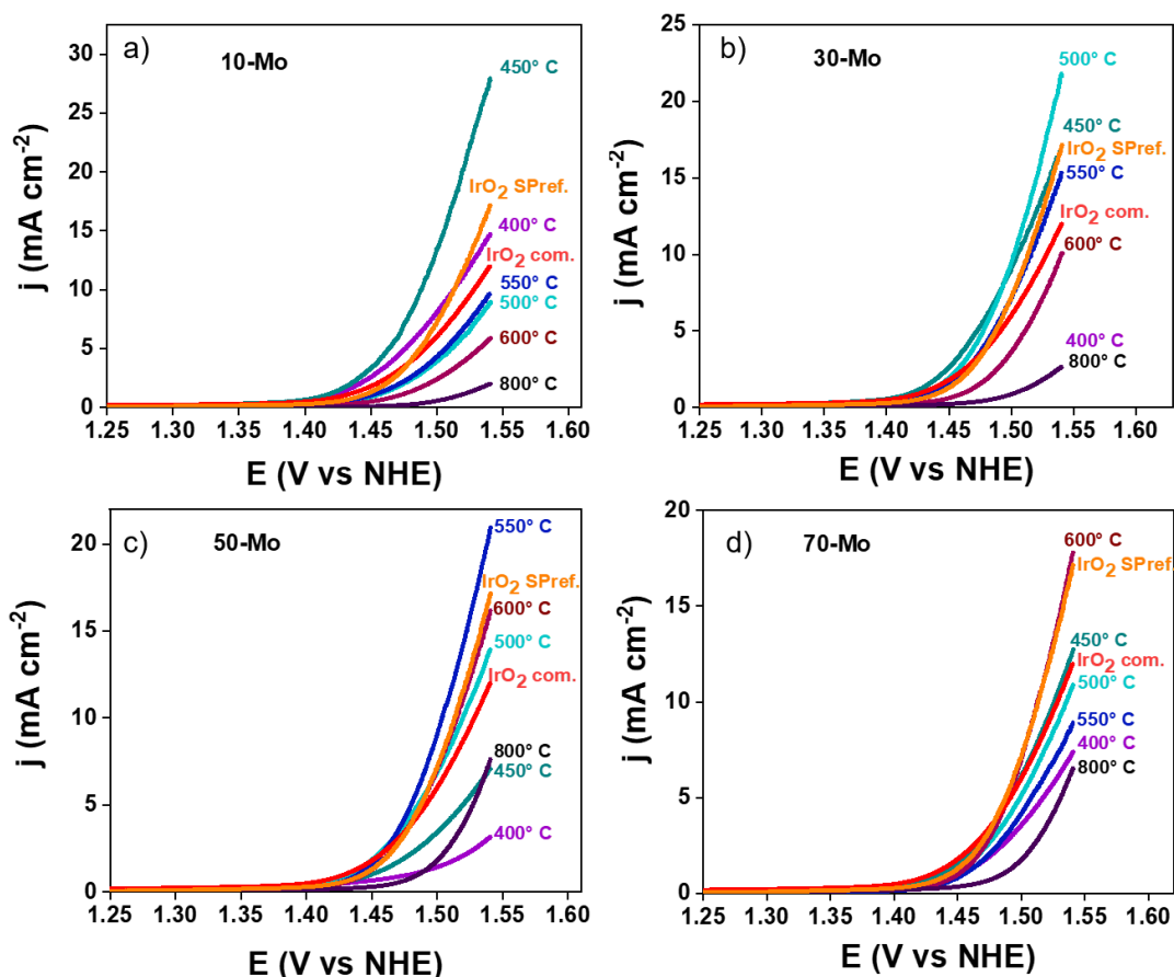
Figure 3.13 Cyclic voltammograms forward scan recorded at 10\text{ mV s}^{-1} of \text{Ir}_{1-x}\text{Mo}_x\text{O}_2 samples obtained after calcination in air at different temperatures.
