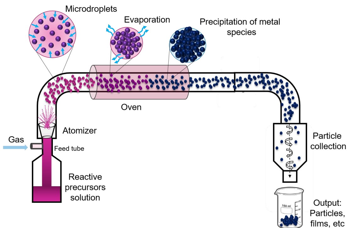
Figure 6.1 General schematic representation of spray-drying process
