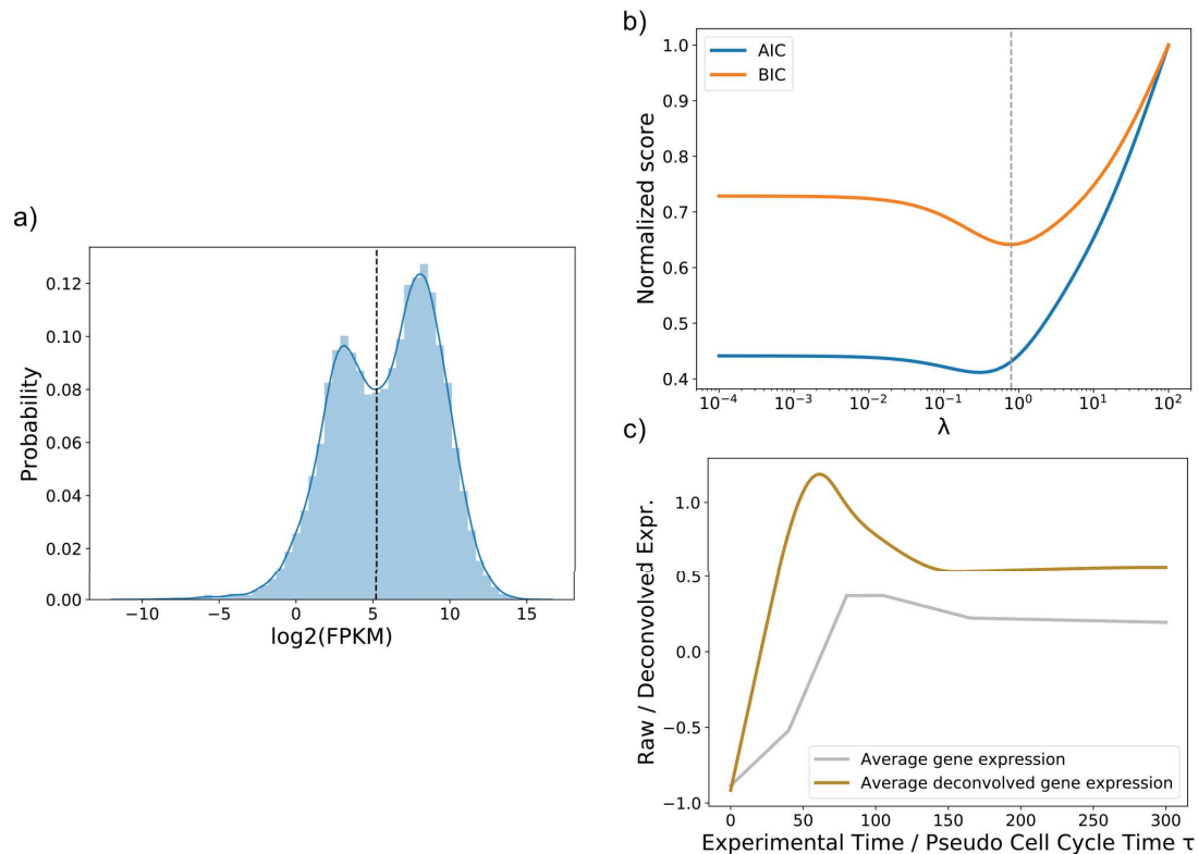
Figure 3.S1. Data processing for deconvolution. a: Log 2 histogram of FPKM reads at gene level for asynchronous data. The dashed vertical line represents the threshold we considered to process our data: genes with asynchronous FPKM < 36.76 were excluded. On the vertical axis, kernel density estimation is indicated. b: AIC and BIC scores were calculated in order to establish the best \lambda parameter for the regularization of the deconvolution process (see Methods). Both AIC and BIC showed a minimum, and we choose \lambda = 0.79 , corresponding to the BIC minimum (dashed vertical line). c: Average gene expression of convolved (grey line) and deconvolved (yellowish line) data were represented on the same plot.
