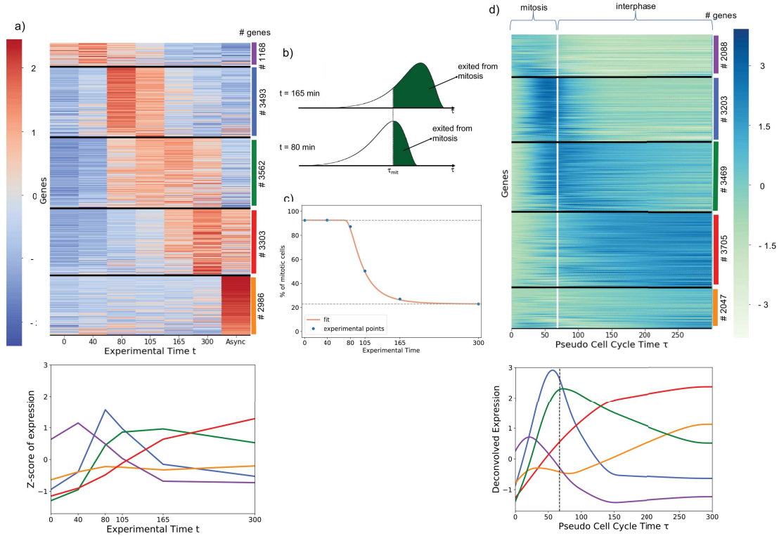
Figure 3.1. Deconvolution of gene expression data of synchronized cell population leads to dynamic expression profile respect to cell-cycle average profile. a: Genes can be divided in groups according to their dynamic expression profiles over time. Each row corresponds to a gene. Black horizontal lines divide the different clusters of genes. The color scale represents the level of the z-score of expression of each gene, as shown by the colorbar on the left. On the right, the number of genes for each cluster is indicated as well as the color corresponding to the cluster expression average shown on the bottom panel. b: We assume that cells have to wait a stochastic, log-normally distributed lag time to start again the cell-cycle progression after the release of the chemical cell-cycle arrest by nocodazole. Here, a pictorial representation of lag time distribution, where the green part of area represents the fraction of cells that already exited mitosis at two different experimental time points. The dashed line indicates time \tau_{\text{mit}} that cells need to complete mitosis. c: Blue dots: quantification of cells showing condensed (mitotic) and decondensed (non-mitotic) chromatin after synchronization release (data from [28]); Orange line: model fitting used to infer \tau_{\text{mit}} and the parameters of the log-normal distribution, \sigma and \mu . d: After the deconvolution, genes were divided in groups according to their dynamic expression profile over the internal pseudo cell cycle time \tau . The vertical white line represents \tau_{\text{mit}} and separates ideally mitosis from interphase in early G1 phase. The color scale represents the level of the z-score of expression of each gene, as shown by the colorbar on the right. On the right, the number of genes for every cluster is indicated as well as the color corresponding to the cluster expression average shown on the bottom to one of the curves on the bottom.
