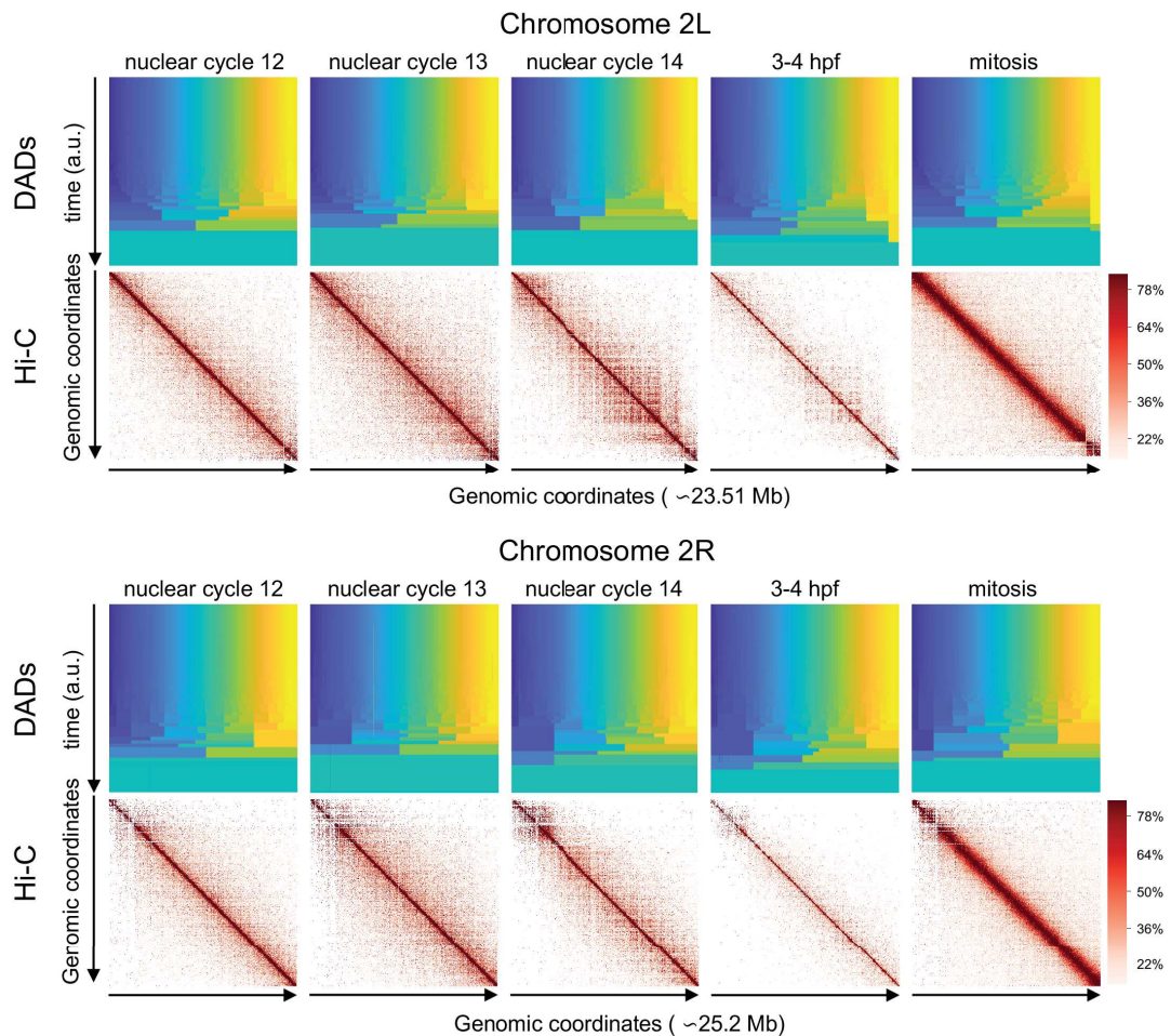
Figure 2.1. Diffusion associate domains (DADs) and Hi-C maps for Dmel Chromosome 2L (left arm, top) and 2R (right arm, bottom). DADs were represented assigning different colours to different communities detected over the genomic coordinates (horizontal axis), over the simulation timesteps progression of the algorithm (vertical axis). For the first timesteps, each region corresponds to a community. Then, as the timesteps increase, coarser communities are detected by the stability algorithm, until a saturation is reached, i.e. the entire network becomes one single community, represented by one single color. Hi-C heatmaps are reported as a reference, with the colorbar on the bottom right providing the percentage with respect to the maximum value of the Hi-C matrix.
