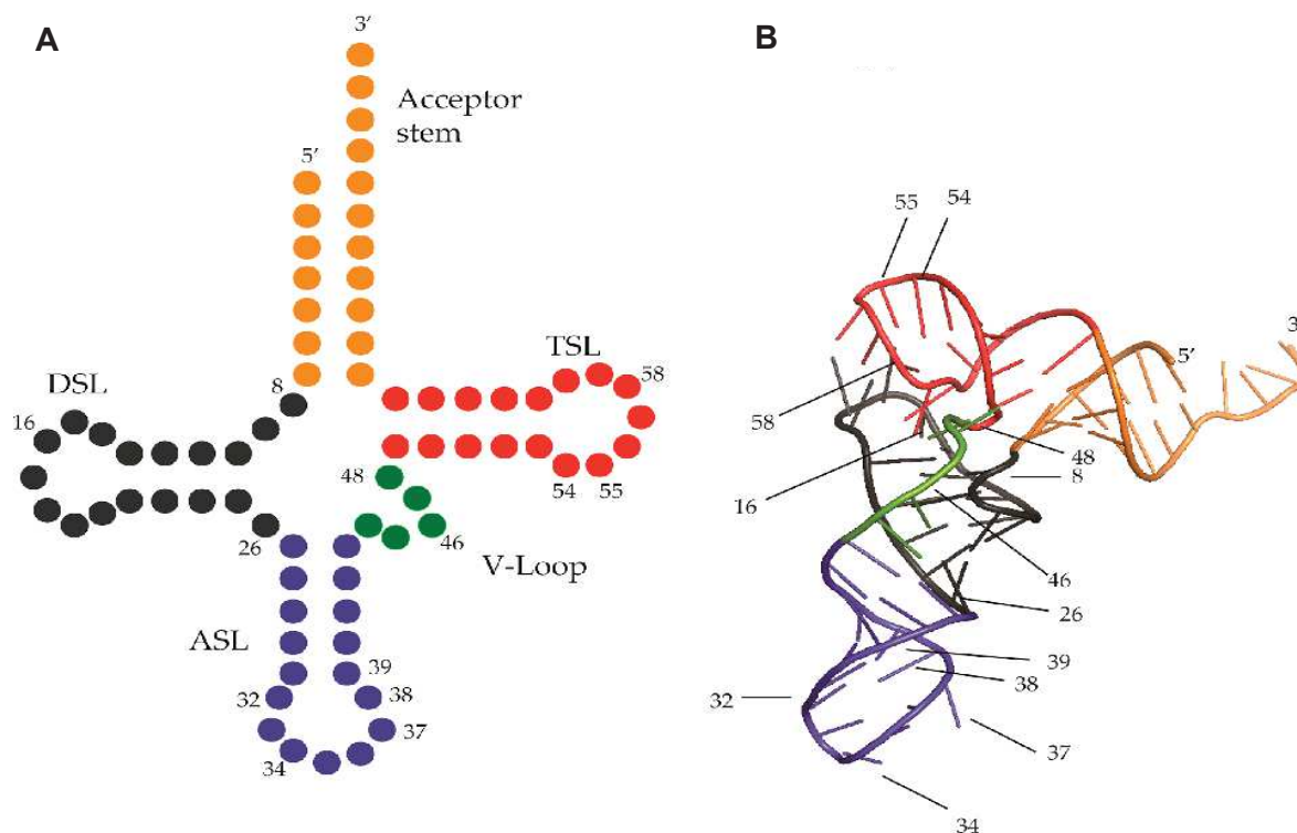
FIG. 32 tRNA ARCHITECTURE
