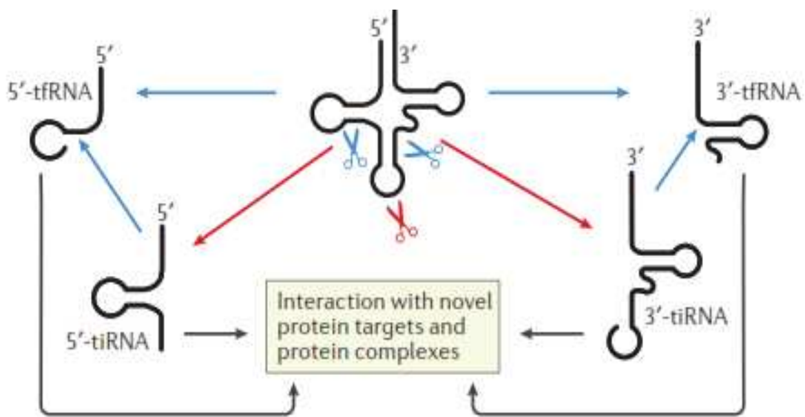
FIG. 37 tRNA FRAGMENTS
