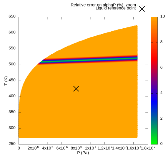
Figure 2.43 – Relative error on \alpha_P compared with IAPWS-97, optimized liquid SRK, with error saturation at 10%.
