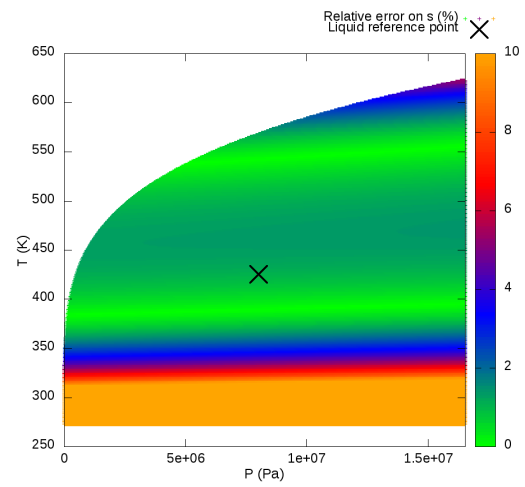
Figure 2.21 – Relative error on s compared with IAPWS-97, optimized liquid NASG, with error saturation at 10%.
