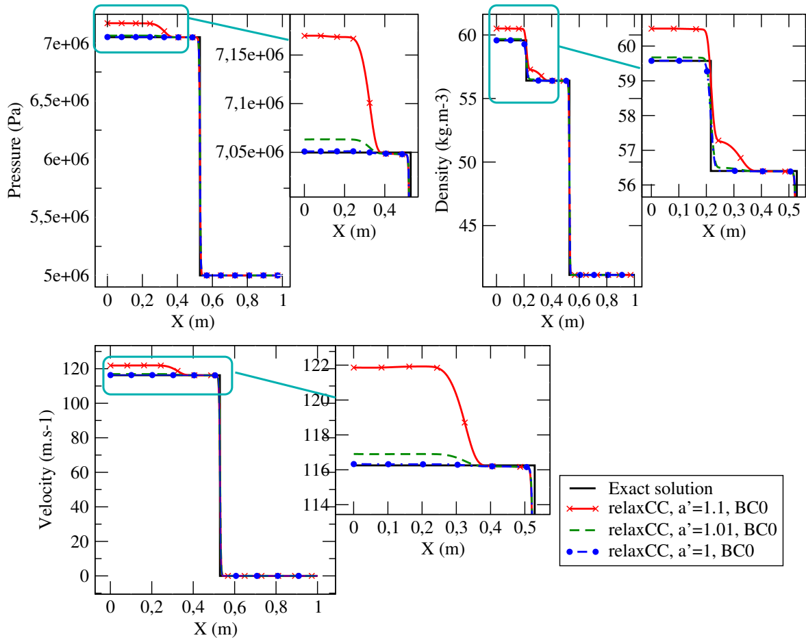
Figure 5.13 – Case 1 with relaxCC scheme and BC_0 . Pressure (Pa), density ( \text{kg}\cdot\text{m}^{-3} ) and velocity ( \text{m}\cdot\text{s}^{-1} ) as a function of X (m) at the final time t_{\text{end}} = 10^{-3}\text{s} . The little windows show zoom on the area close to the outflow. The exact solution is compared with numerical solutions obtained with relaxCC tested with several a' on a mesh containing 1000 cells.
