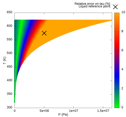
Figure 2.47 – Relative error on \tau compared with IAPWS-97, optimized vapor SG, with error saturation at 10%.
