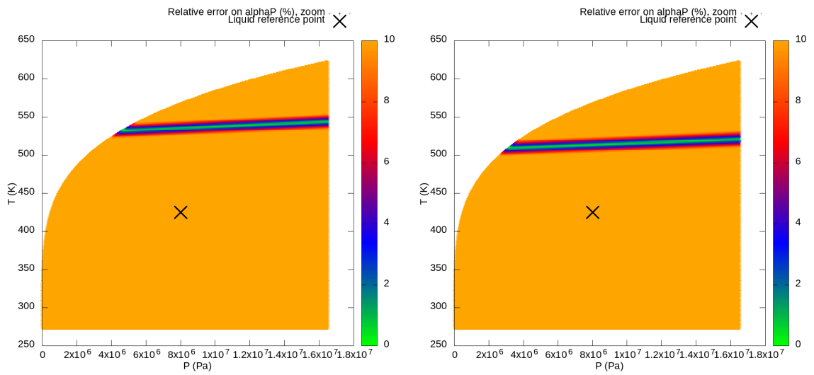
Figure 2.42 – Relative error on \alpha_P compared with IAPWS-97, initial liquid SRK, with error saturation at 10%.
