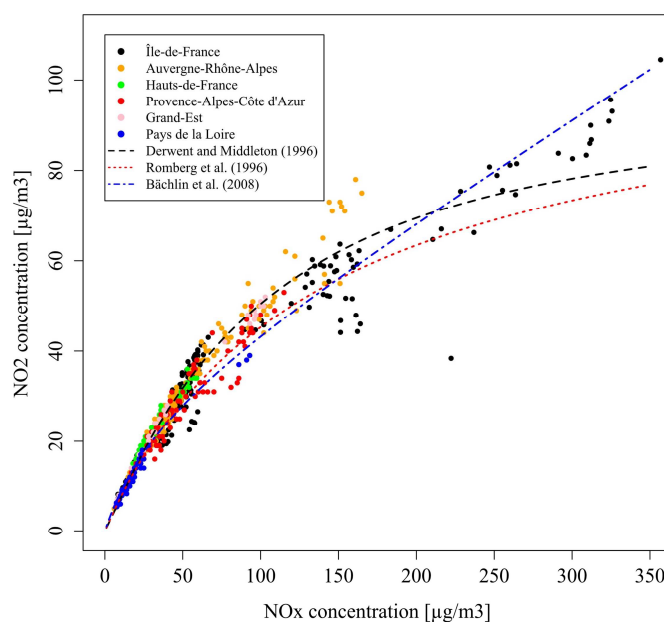
Figure 5.3 – Evolution of \text{NO}_2 concentration as a function of \text{NO}_x concentration and comparison with empirical functions.
