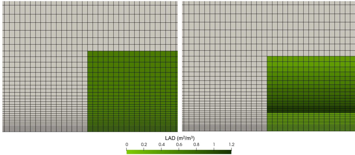
Figure 2.30 – Mesh illustration for the uniform LAD (left) and the chosen LAD (right).
