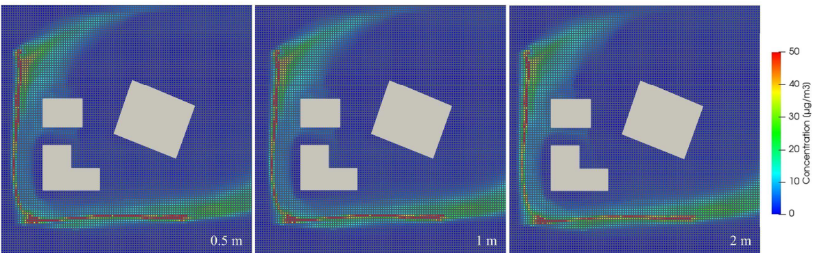
Figure 3.7 – Comparison of the results at z = 2 m for the different injection heights considered.
