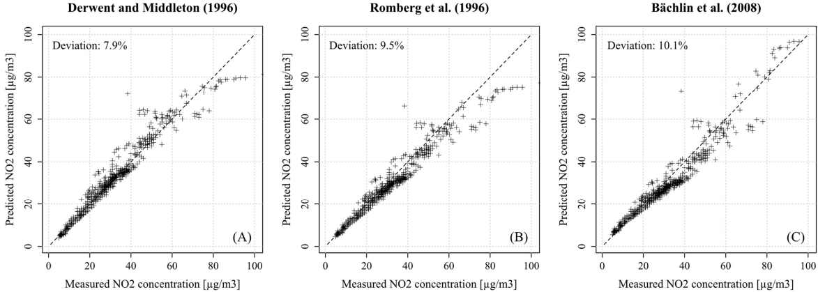
Figure 5.4 – Comparison between predicted and measured NO 2 concentrations for (A) the Derwent and Middleton function, (B) the Romberg et al. function, and (C) the Bächlin et al. function.
