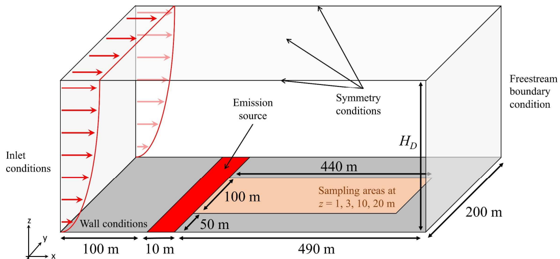
Figure 3.2 – Boundary conditions and domain size.
