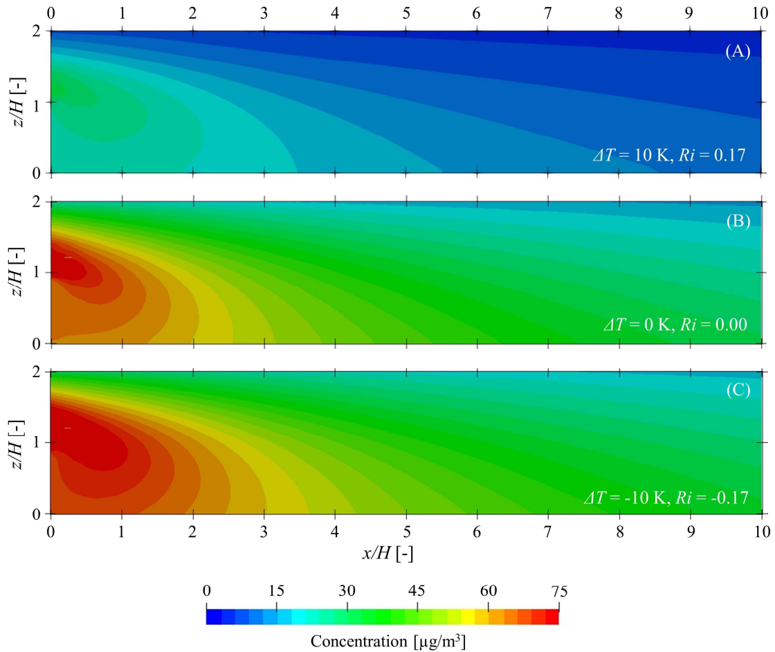
Figure 7.9 – Evolution of the concentration behind the downwind barrier as a function of the temperature variation in the same wind conditions (perpendicular wind, U_H = 3.15 m/s).
