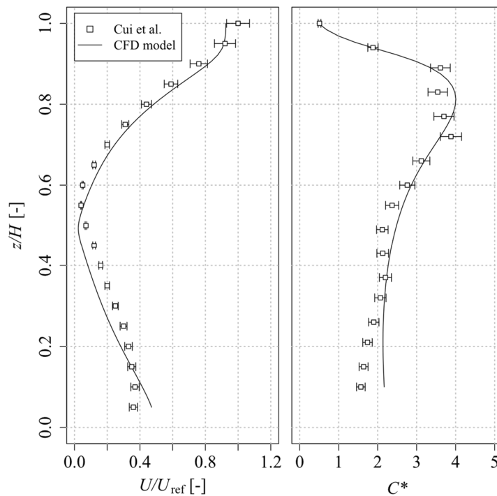
Figure 7.5 – Vertical distribution of dimensionless velocity and concentration for Ri = -1.22 given by Cui et al. for the wind tunnel measurements (Cui et al., 2016), and comparison with the CFD model used for this study with Sc_t = 0.25 .
