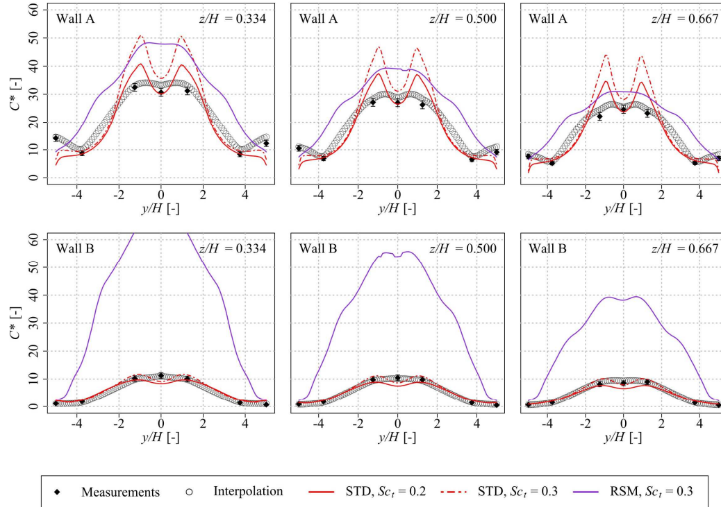
Figure 2.18 – Comparison of dimensionless concentrations between the numerical model and the experimental data with the standard k-\epsilon turbulence model (STD, red curves) and the Reynolds stress model (RSM, purple curve).
