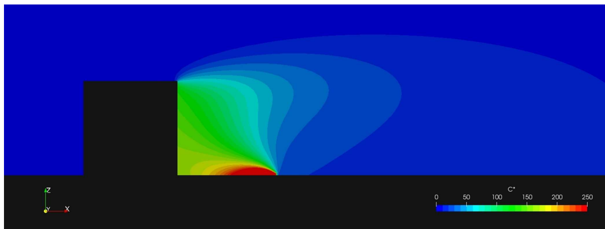
Figure 2.13 – Evolution of dimensionless concentrations after the 2D obstacle with the standard k- \epsilon turbulence model and Sc_t = 0.9
