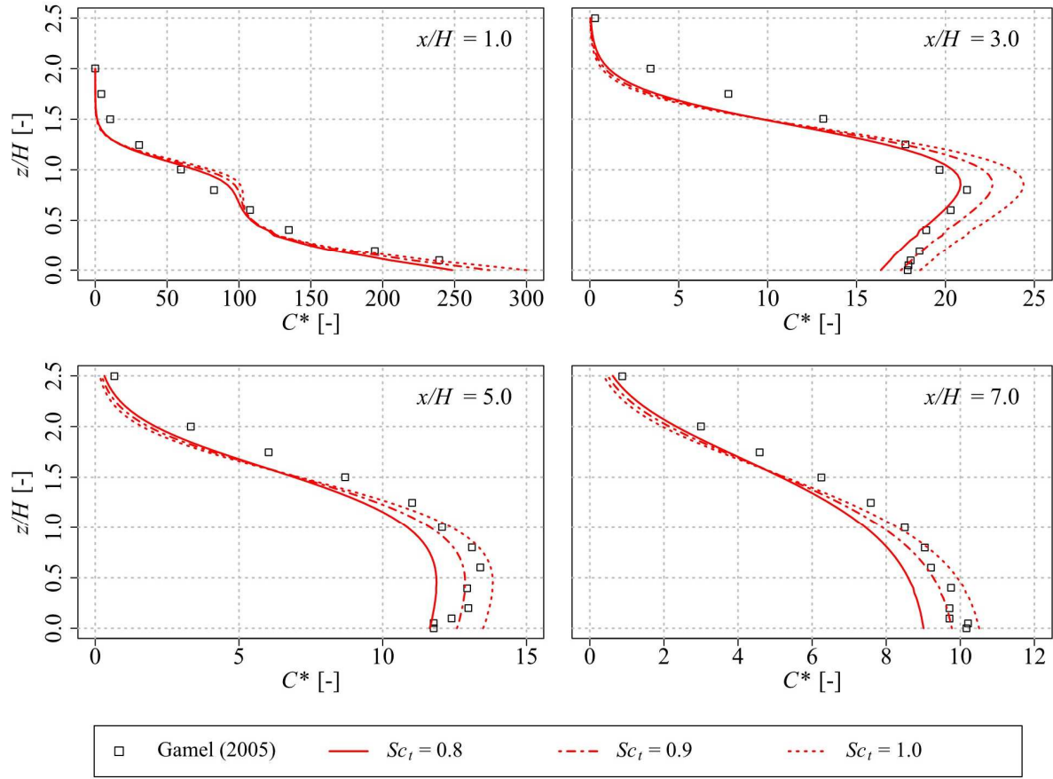
Figure 2.12 – Comparison of dimensionless concentrations between the numerical model and the experimental data of Gamel (2005) with the standard k- \epsilon turbulence model for three turbulent Schmidt numbers.
