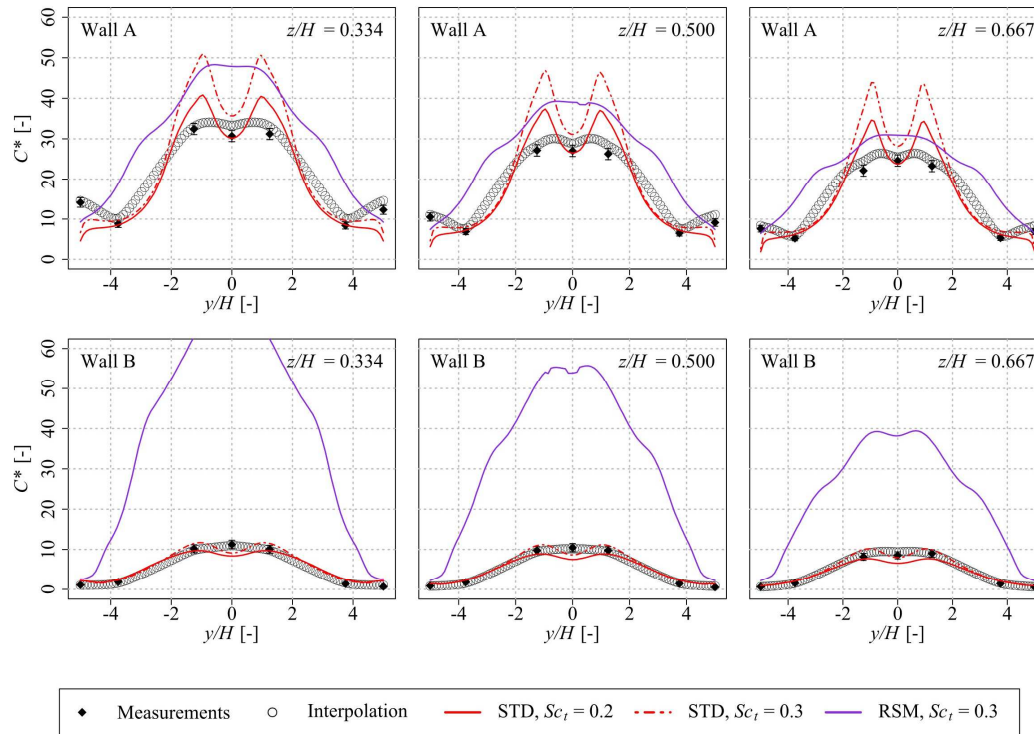
Figure 2.18 – Comparison of dimensionless concentrations between the numerical model and the experimental data with the standard k-ε turbulence model (STD, red curves) and the Reynolds stress model (RSM, purple curve).
