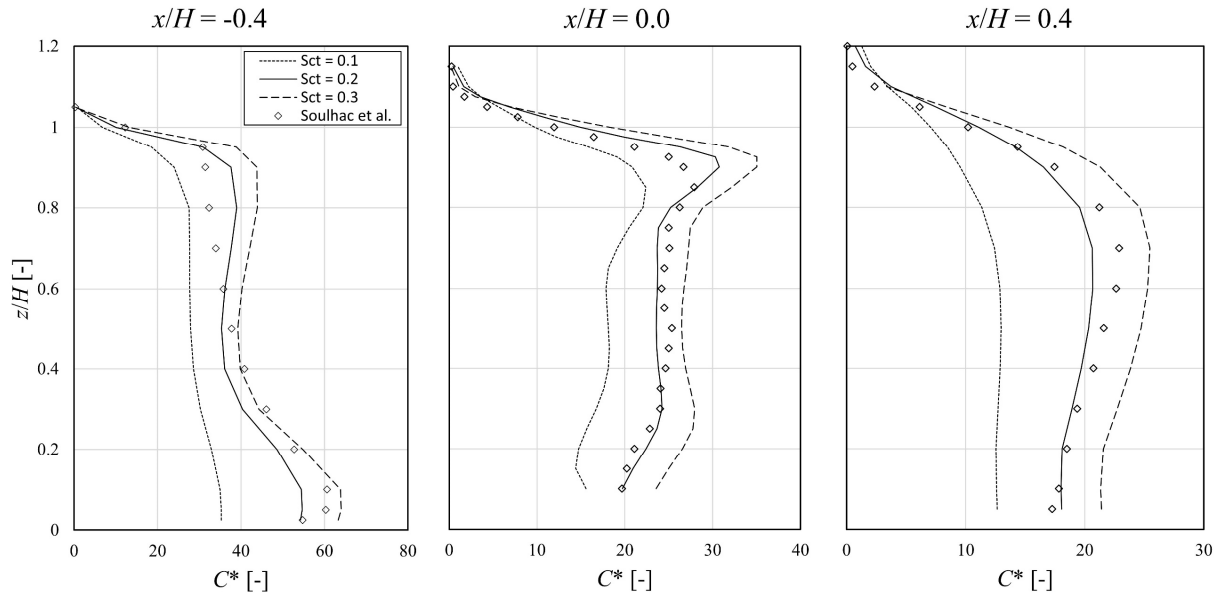
Figure 6.5 – Vertical distribution of numerical dimensionless concentrations for different Sc_t compared to Soulhac et al. (2001) experimental data.
