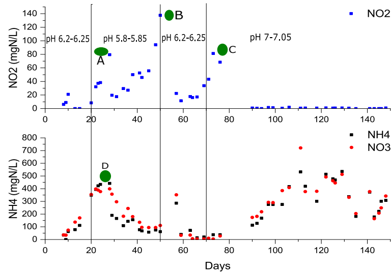
FIGURE 3.18: (a) NO 2 , (b) NH 4 and NO 3 concentration in the outlet over time of the second campaign.
