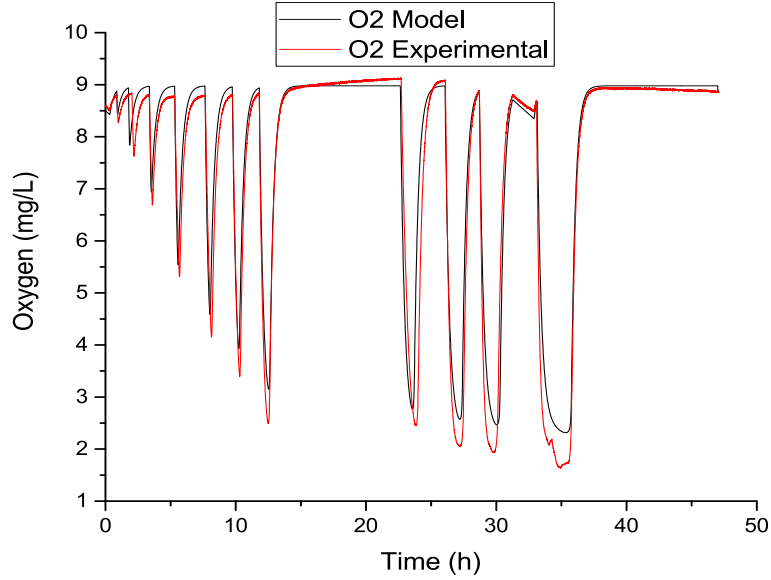
FIGURE 4.13: Parameters adjustment for NOB bacteria ( \mu_{max_N X_N} , K_{(S,FNA,N)} , K_{(i,FNA,N)} and K_{(O,N)} validation)
