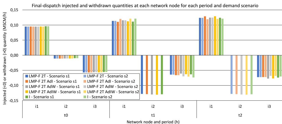
Figure 11: Network use for various adjustment-products offering for a congested network (D=0.4m) under time-uncertainty of demand
