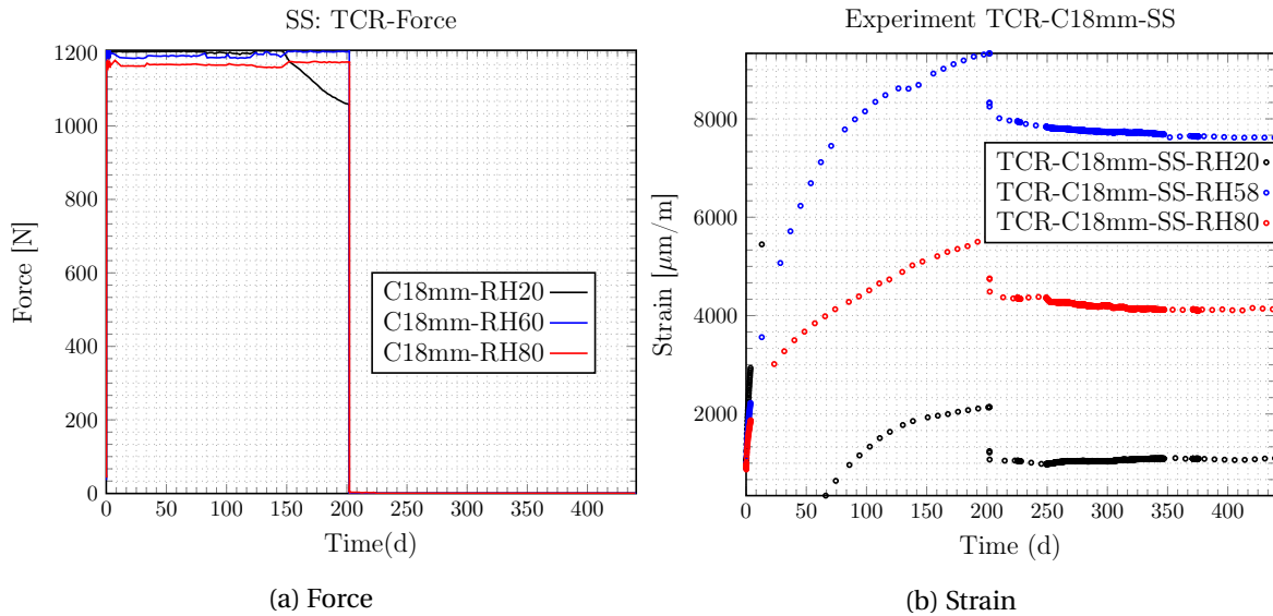
Figure 4.23: Loading history (a) and the evolution of delayed strains for three relative humidity history (b).
