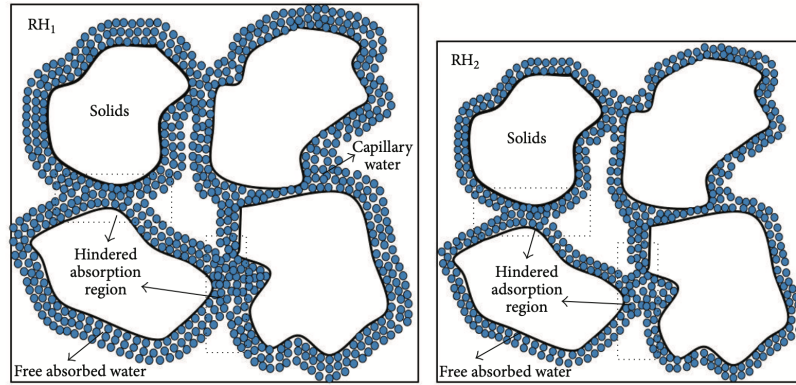
Figure 1.11: Schematic representation of Gibbs-Banham shrinkage (Ye and Radlinska, 2016)
