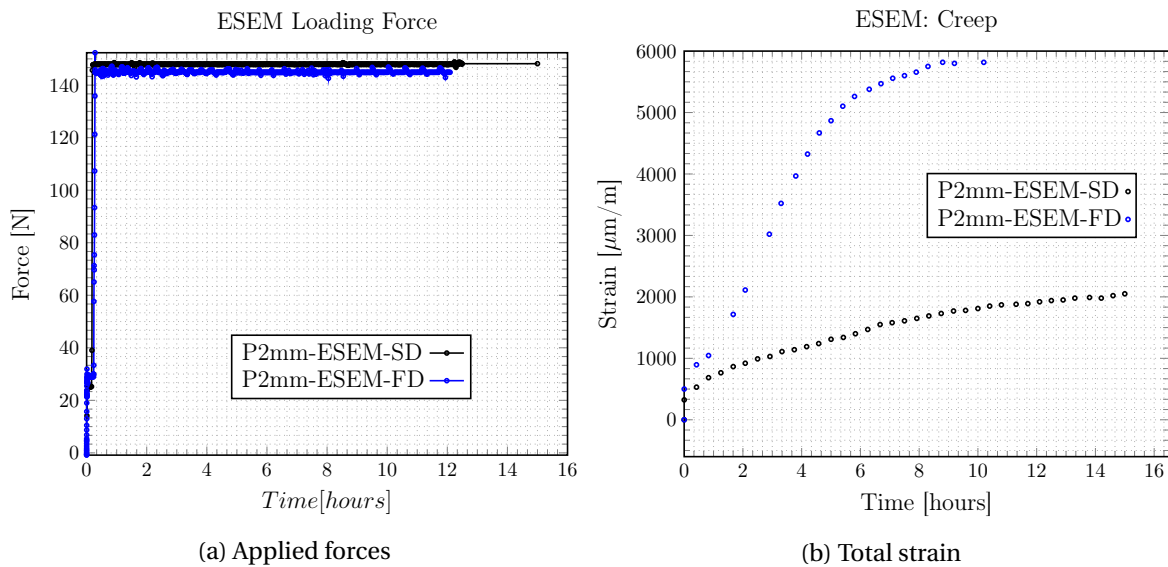
Figure 4.9: (a) Evolution of loading force and (b) corresponding creep strains for the tests under ESEM
