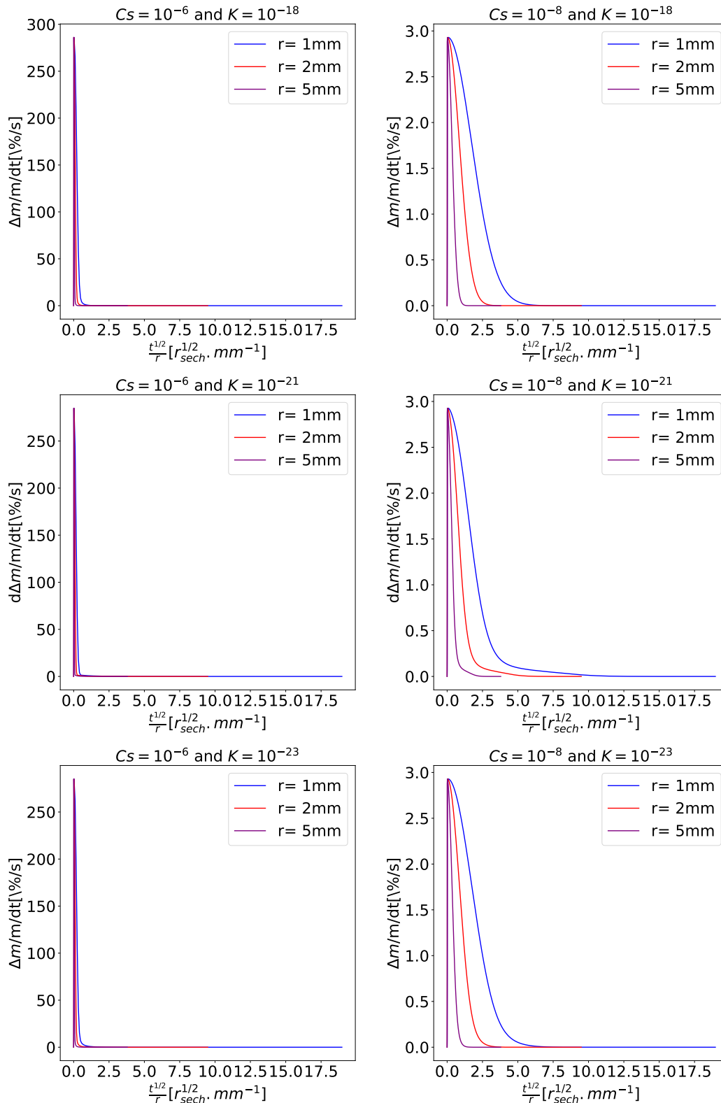
Figure 3.12: Kinetic of mass loss evolution for material intrinsic permeability of K = 10^{-18} , 10^{-21} and 10^{-23} m^2 , each for exchange coefficient C_s = 10^{-6} , 10^{-7} , 10^{-8} kg.m^{-2}.s^{-1} and drying thicknesses r = 1, 2, 5 mm
