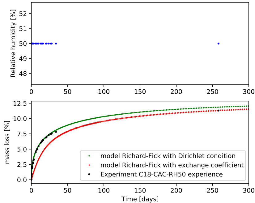
Figure 3.6: Simulation of the experiment DS-C18-CAC-RH50 using the complete Richards-Fick model with the two types of boundary conditions: Dirichlet (without exchange coefficient) and Neumann (with the identified exchange coefficient)
