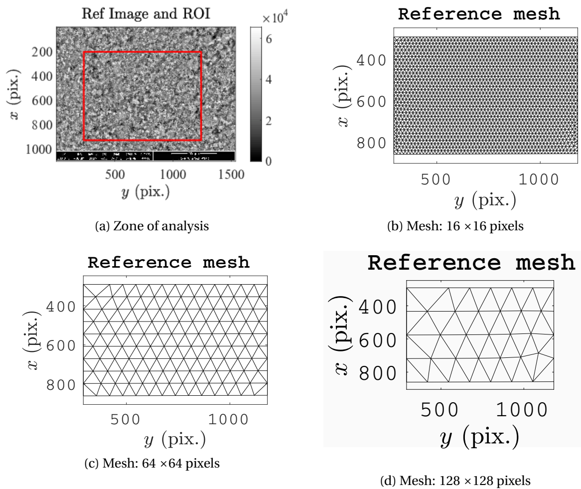
Figure 2.7: Region of Interest (a) and (b, c, d) different mesh sizes tested in uncertainty analysis.
