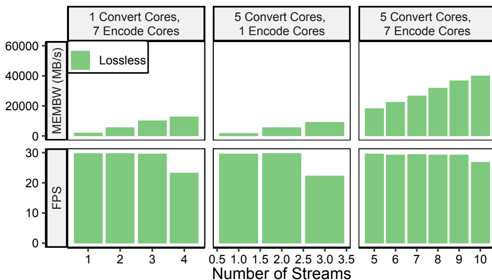
Figure 5.7: vMI performance using the kernel network stack, with a full media processing pipeline. A copy is performed at each stage of the pipeline. The optimal allocation is represented in the last column, as the total number of available cores is 24 = 3 \text{ IRQ Cores} + 5 \text{ RX Cores} + 4 \text{ Parse Cores} + 5 \text{ Convert Cores} + 7 \text{ Encode Cores} .
