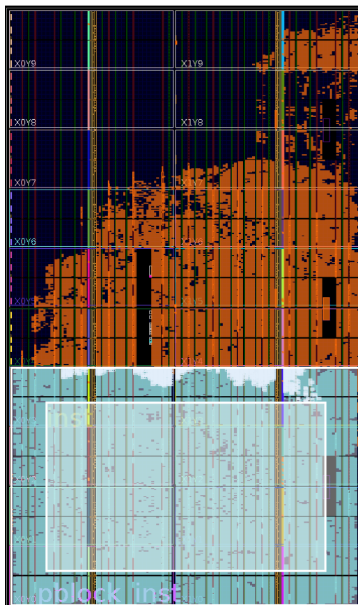
Figure 3.4: Floorplanning for OP4T with the packet processor defined in 3.4. The lower part is reconfigurable and allocated to the packet processor (blue), which almost fills it. The upper part is allocated to the static design (orange). In white are represented interconnection points between the reconfigurable packet processor and the static design.
