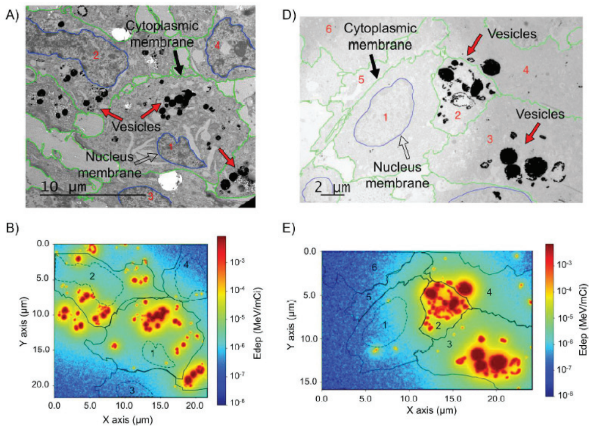
Figure 6.3.: Figure taken from Laprise-Pelletier et al. [2018] illustrating the dose inhomogeneity at cellular scale following the injection of radioactive ( ^{103}\text{Pd} ) GNPs in a prostate cancer. The biodistributions were obtained at 24 h and 8 days following the intratumoral injection.
