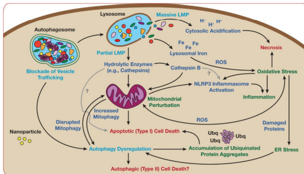
Figure 4.3.: Possible pathways of nanomaterial toxicity, taken from Stern et al. [2012]. LMP: lysosome membrane permeabilization.
