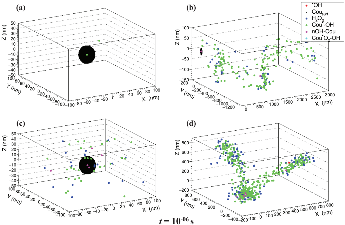
Figure E.3.: Spatial distribution of the chemical species after a GNP ionization at t = 10^{-6} s after the ionization. Panels (a) and (b) (respectively (c) and (d)) represent the same track, with (a) (respectively (c)) a zoom around the GNP.
