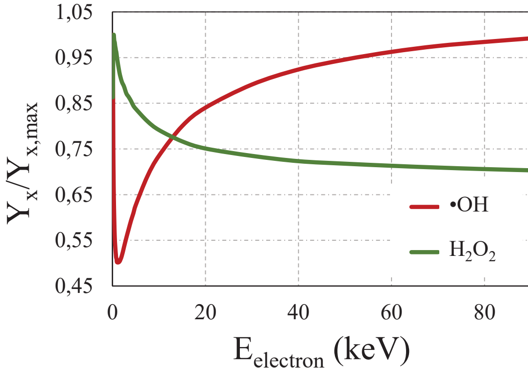
Figure D.1.: Chemical yields of \text{H}_2\text{O}_2 and \bullet\text{OH} as a function of the primary electron energy, at 1 \mu\text{s} , normalized to the maximum.
