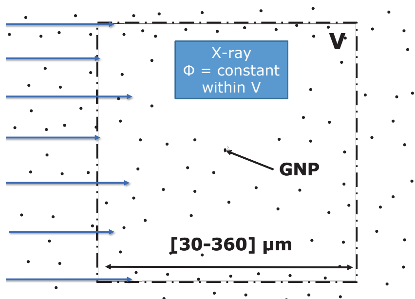
Figure 12.5.: Schematic view of the system considered for radical species calculation. \Phi represents the fluence of the beam, and is set constant within the volume of interest V . The GNPs represented by small dots have a concentration C_{\text{NP}} and are homogeneously distributed.
