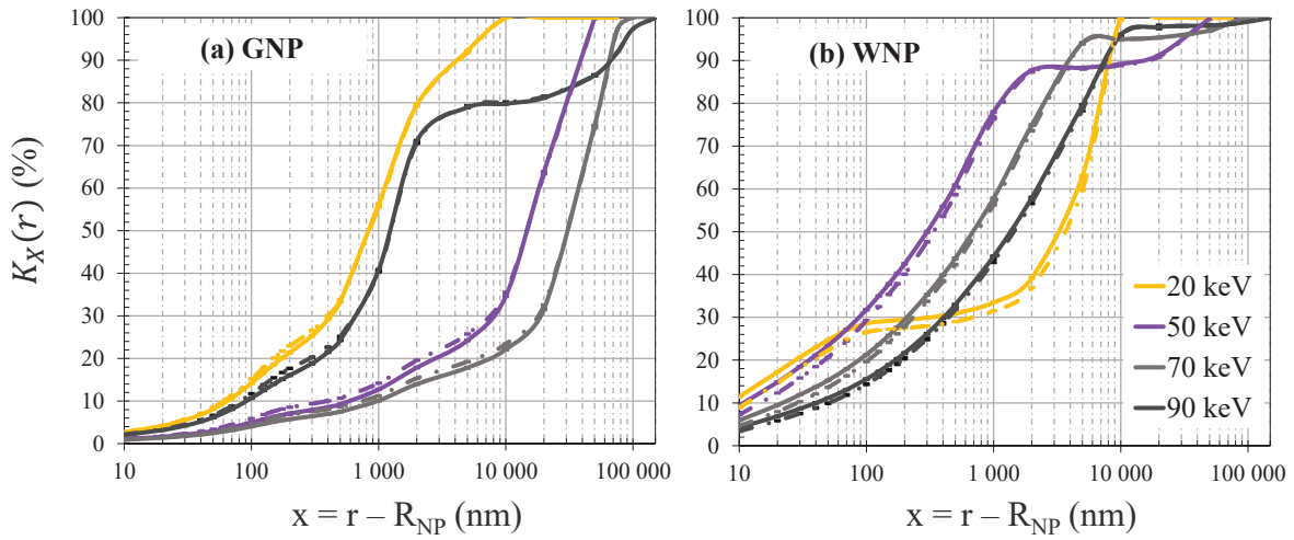
Figure 11.5.: Cumulative number of chemical species X , K_X(r) ( \bullet\text{OH} in solid line and \text{H}_2\text{O}_2 in dashed line), as a function of x . Results are displayed for E_{\text{photon}} varying from 20 to 90 keV. Panel (a): GNP, panel (b): WNP. R_{\text{NP}} = 5 nm, and t = 10^{-12} s.
