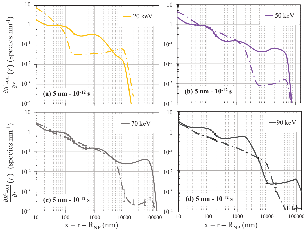
Figure 11.4.: Radial differential distribution of the number of chemical species \frac{\partial R^{\bullet\text{OH}}}{\partial r} as a function of x . In each panel, results are given for a GNP (solid line) and a WNP (dashed line). Results are displayed for E_{\text{photon}} varying from 20 to 90 keV. R_{\text{NP}} = 5 nm, and t = 10^{-12} s.
