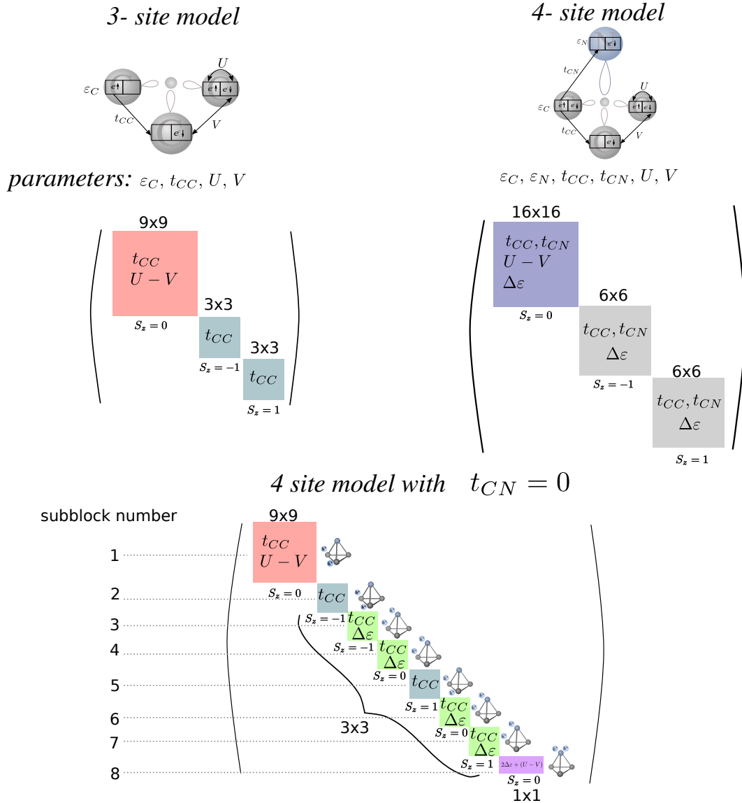
Figure 6.2.12: Schematic representation of the Hamiltonians of the 3-site model on the top left panel; 4-site model - top right panel; and the limit case t_{CN} = 0 in the 4-site model in the bottom panel. The identical sub-blocks in Hamiltonians are highlighted with the same color. The text within each sub-block indicates on which parameters it depends. A small drawing near each sub-block illustrates where the holes are localized in the basis functions corresponding to this sub-block.
