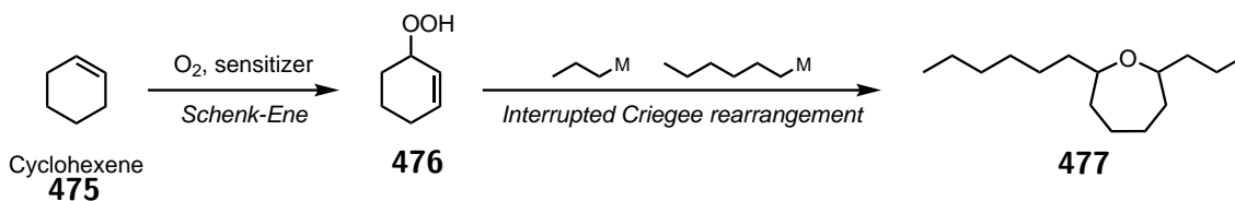
Figure 3.36: Possible pathway to isolaurepan from cyclohexene 475 .
