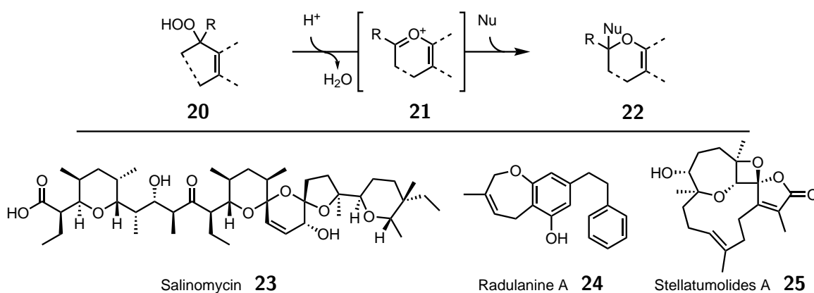
Figure 1.4: Top, Interrupted Hock cleavage; bottom, Natural products containing cyclic ethers.
