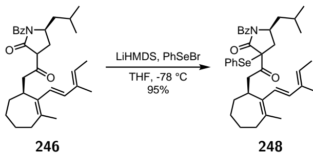
Figure 2.44: Synthesis of pre dienophile 248 .
