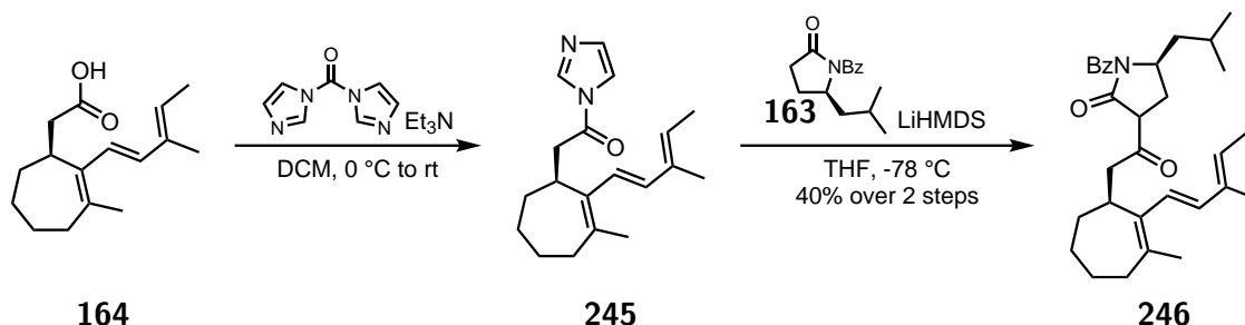
Figure 2.42: First pathway to \gamma -lactam 246 .
