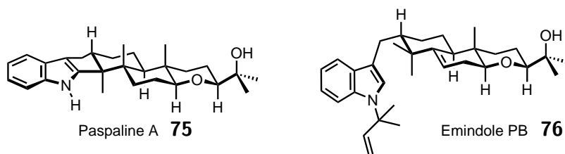
Figure 1.15: Paspaline A 75 and emindole PB 76 .
