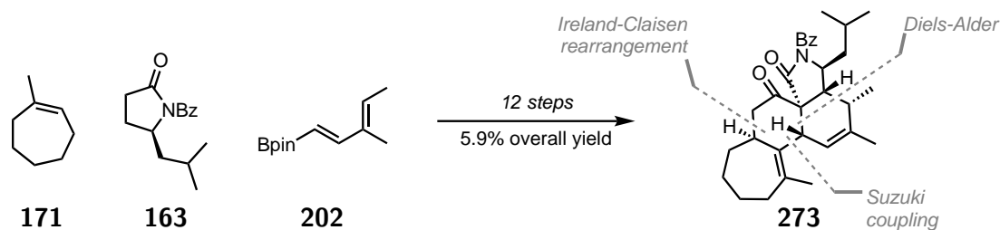
Figure 2.59: Total synthesis of key biomimetic intermediate 273 .
