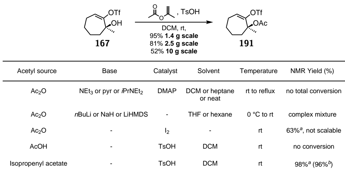
Figure 2.22: Synthesis of coupling partner 191 .
