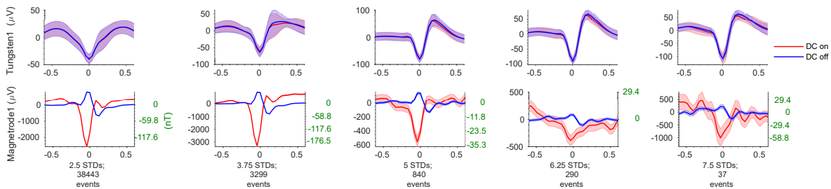
Figure 4.16: Experimental results of the averaged recordings on a tungsten electrode and M1 (2018-Block 23-Probe SOI-ref.712) when an external noise is generated by a coil, and the related effect according to the threshold level.
