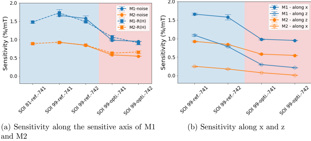
Figure 3.30: (a) Comparison of the sensitivity of M1 and M2 along their sensitive axis (respectively x and z). The results from R(H) and noise measurements are coherent. (b) Comparison of sensitivity of M1 and M2 along their sensitive axis (full circles) and perpendicularly to it (empty circles). For the reference GMR stack, sensitivity of M1 perpendicularly to its sensitivity axis and M2 along its sensitivity axis are very similar. For the optimized GMR stack, each sensitivity is well separated.
