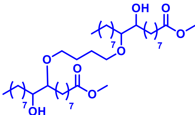
Figure S4.10 – Chemical structure of MO Diol-diester formed during MO Diol synthesis.
