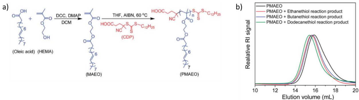
Figure 1.19 – (a) Synthesis of PMAEO by RAFT polymerization, and (b) GPC RI curves of products from thiol-ene reaction of PMAEO with different thiols. Adapted from reference (Maiti, Kumar, and De 2014).
