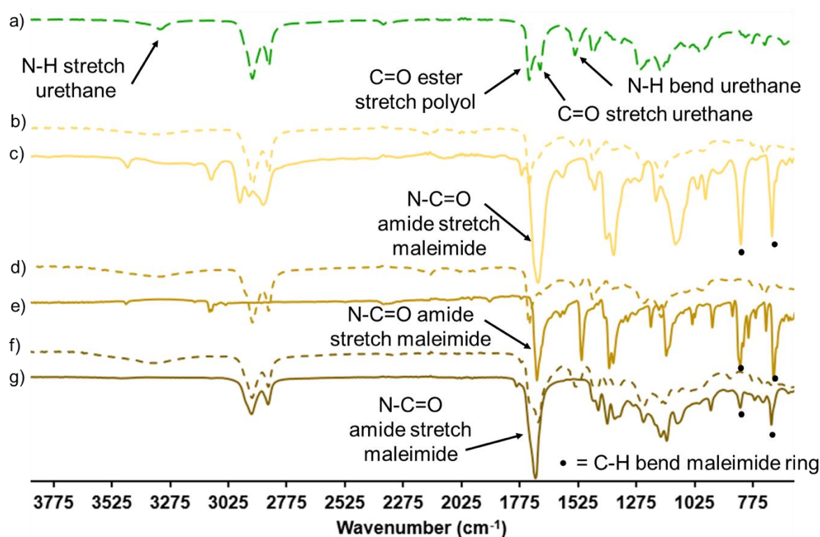
Figure 4.6 – FTIR spectra of, from top to bottom, (a) PU-HS20, (b) PU-HS20-PPOBMI, (c) PPOBMI, (d) PU-HS20-MPBMI, (e) MPBMI, (f) PU-HS20-MOBMI, and (g) MOBMI.
