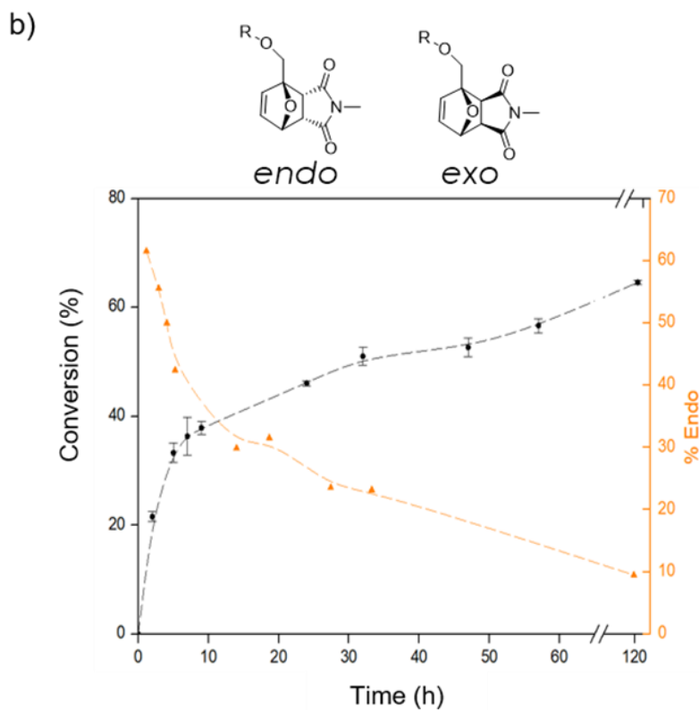
Figure 2.3 – (a) ^1\text{H} NMR spectra of mixture of FO and N-methylmaleimide after 0 and 24 h. (b) Conversion and percentage of endo structure with respect to time at 65 °C.
