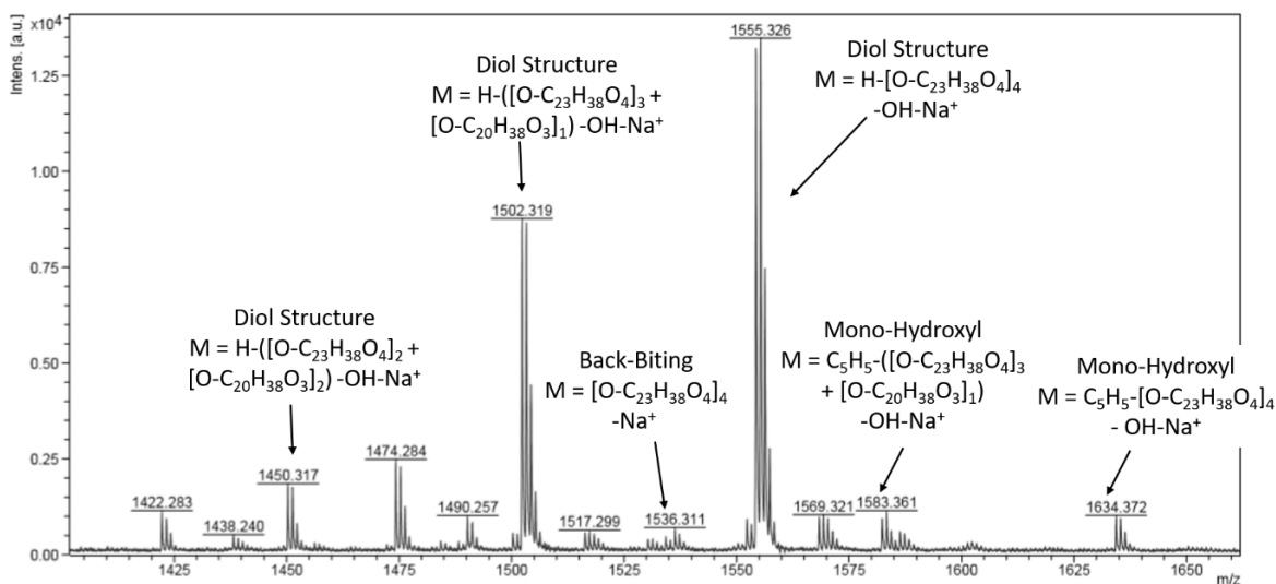
Figure S2.17 – MALDI-TOF MS spectrum of oligomer B zoom on series n = 4 on the ion. Matrix solutions was freshly prepared: DHB was dissolved to saturation in a \text{H}_2\text{O}/\text{CH}_3\text{CN}/\text{HCOOH} (50/50,1%) solution.
