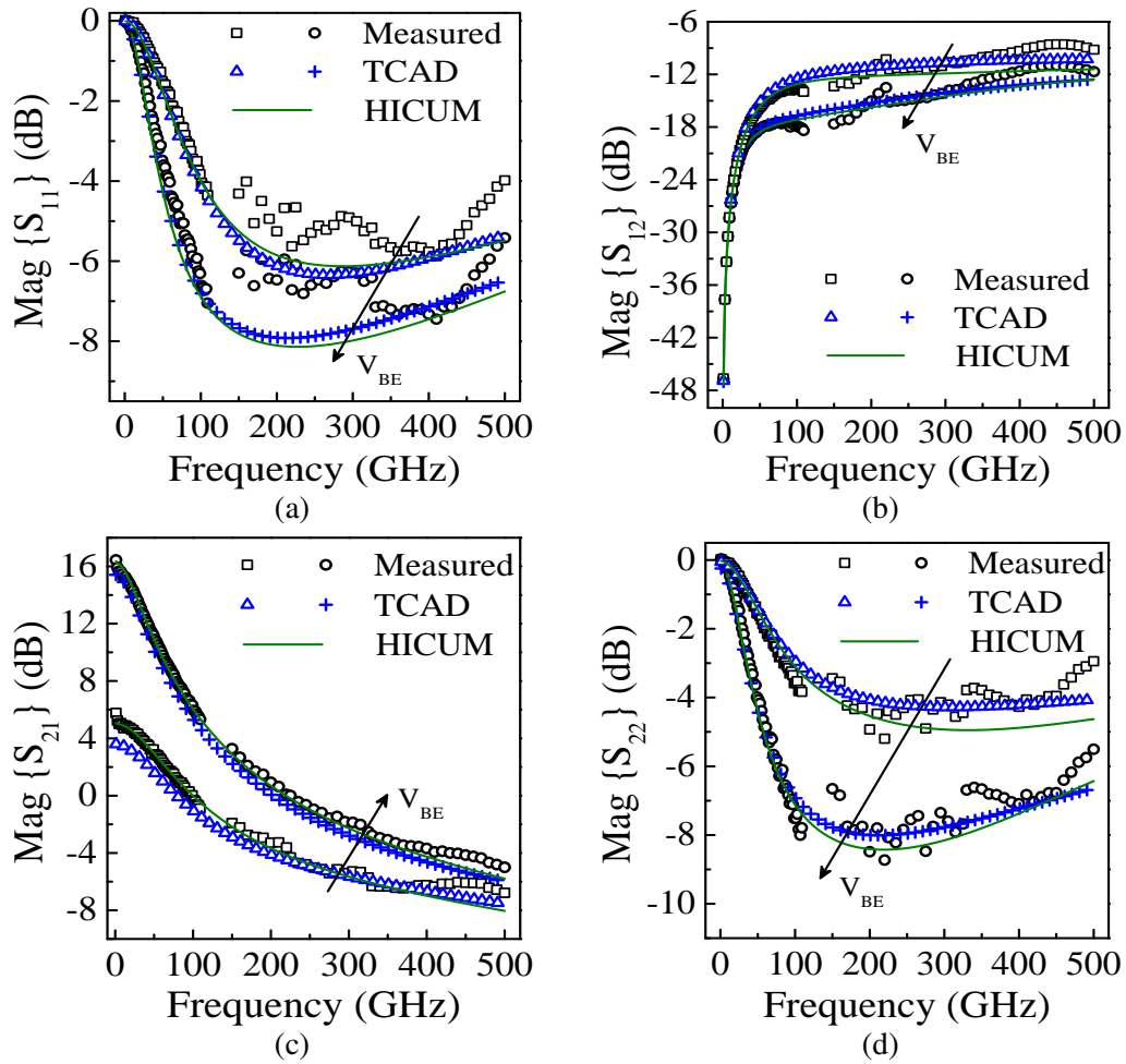
Fig. 5.19: Frequency-dependent magnitude of scattering parameters for the 0.09 \mu\text{m} \times 4.8 \mu\text{m} SiGe HBT biased at V_{BC} = 0\text{V} with V_{BE} = 0.8 \text{V} and 0.85 \text{V} : comparison between measured data (rectangles and circles), TCAD (triangle and cross) and HICUM (solid lines).
