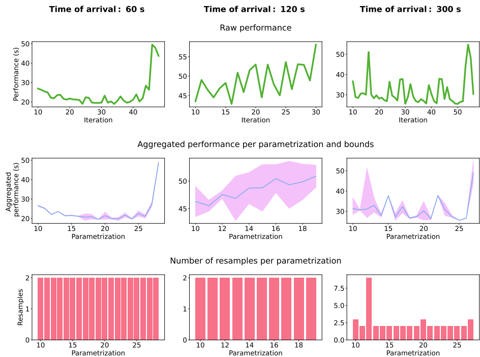
Figure 5.15: Example of trajectories for dynamic resampling on the SRO experiment
