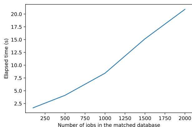
Figure 7.4: Time to match applications per database size
