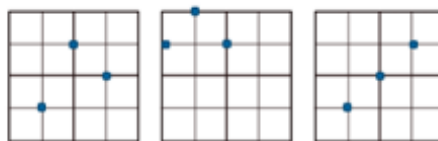
Figure 3.2: Example of designs respecting the non-collapse constraint but not space-fill constraints
