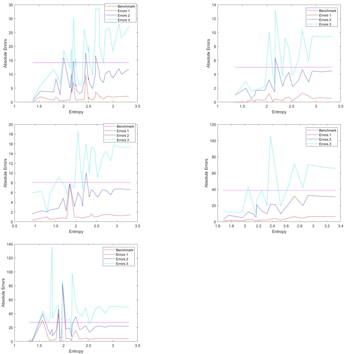
FIGURE 2.6: Shannon entropy analysis. As in the previous charts: [Top] (Left) Uniform distribution; (Right) Beta distribution with \alpha = 1 and \beta = 3 . [Center] (Left) Beta distribution with \alpha = \beta = 0.5 ; (Right) Beta distribution with \alpha = \beta = 2 . [Bottom] (Left) Beta distribution with \alpha = 1 and \beta = 0.5 .
