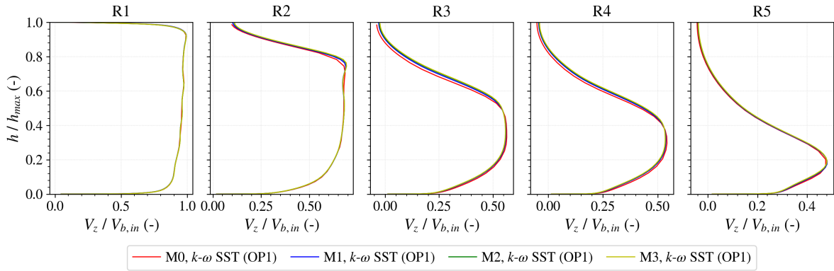
Figure 4.5: Normalized mean axial velocity profiles obtained with meshes M0 to M3 in RANS.
