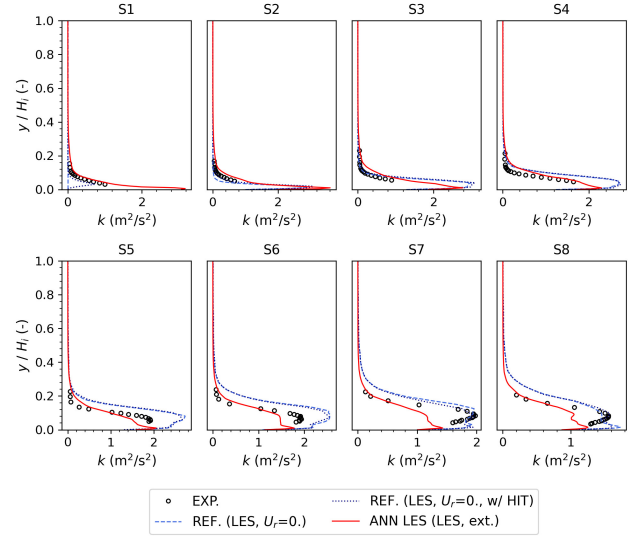
FIG. 26: Comparisons of experimental and numerical turbulence kinetic energy profiles inside the diffuser using LES and the proposed strategy.
