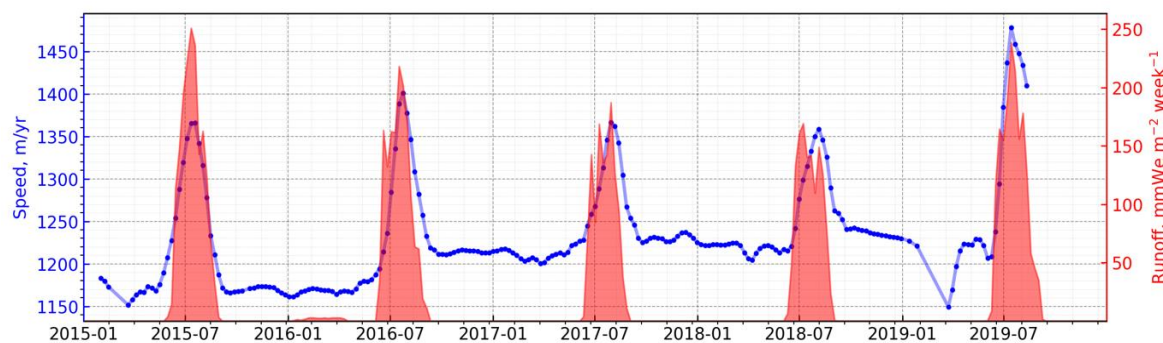
Figure 32 Satellite-derived ice surface velocity and the MAR modelled surface water runoff on the Petermann Gletscher near the front (orange point in Figure 31-c).
