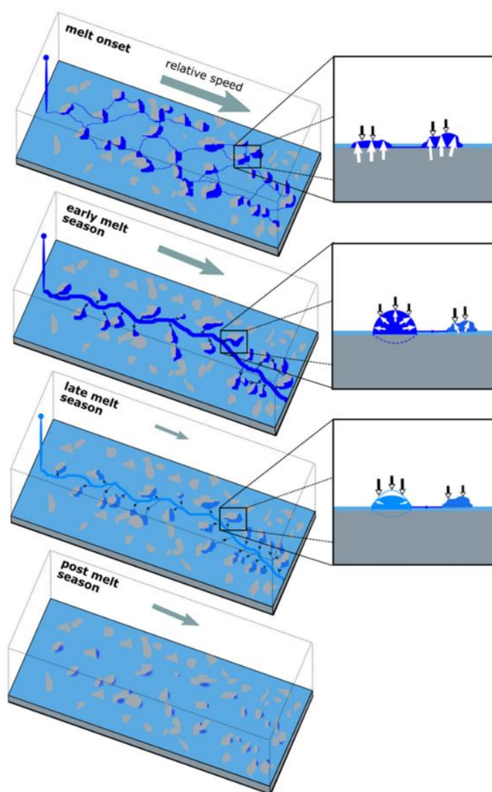
Figure 12 Stages of subglacial hydrological system development from early spring to late autumn. The main subplots present a planar view of the network, zoom subplots on the right show vertical cross-sections of the channels and water-filled cavities. The size of the gray arrows is proportional to the ice speed; white and black arrows in zoom subplots indicate the relative ice creep closure force and water pressure opening force, respectively. From Davison et al., 2019.
