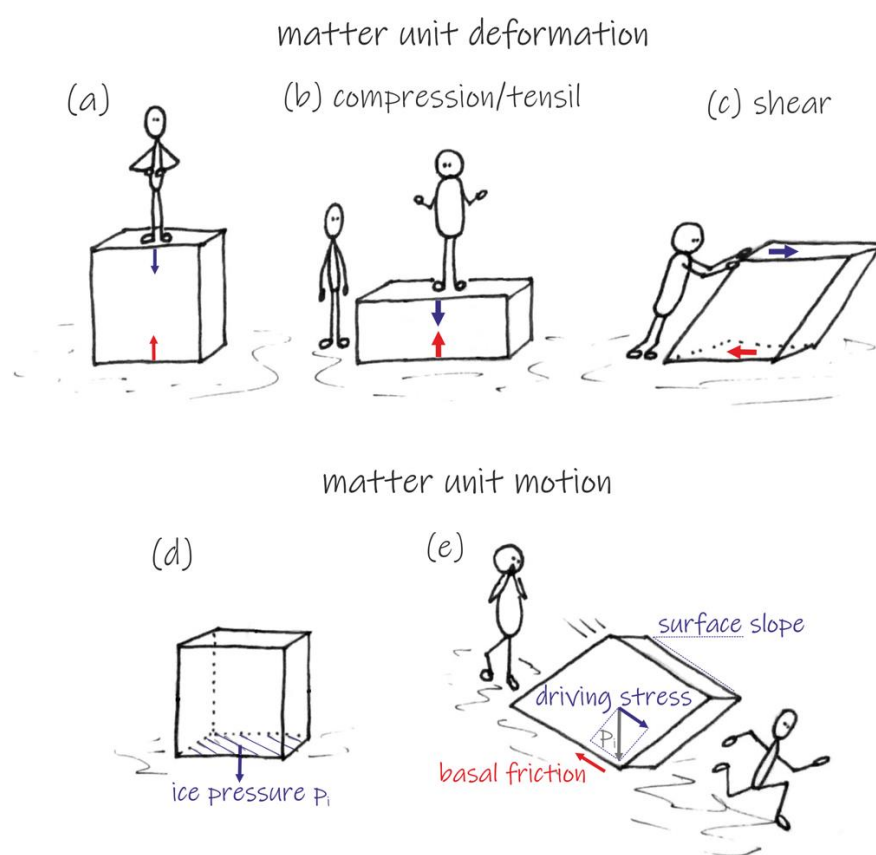
Figure 4 (a)-(c) types of matter deformation under the stresses; (d)-(e) ice pressure generates the stress for the ice block motion.
