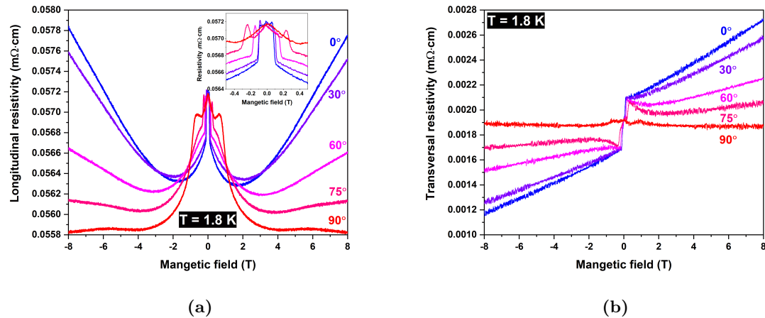
Figure 6.6: (a) and (b) The longitudinal and transverse magnetoresistance of \text{MnBi}_4\text{Te}_7 measured up to 8T. (Sample FMBT1)
