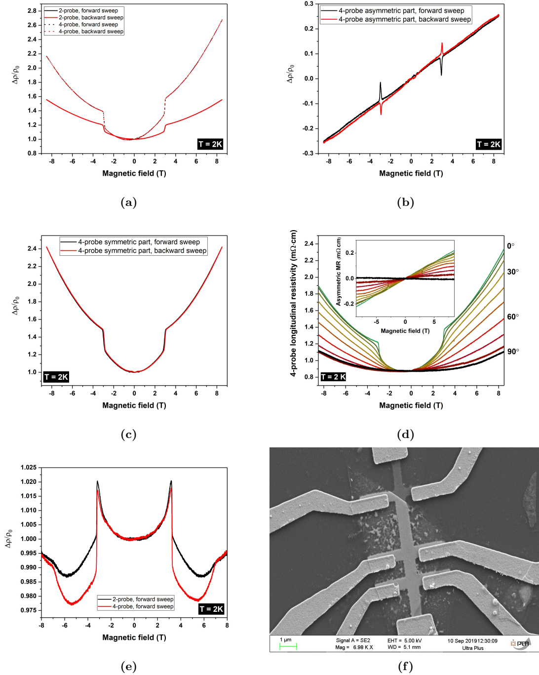
Figure C.4: Comparison of 2-probe and 4-probe magnetoresistivity. In this work, sample ATMBT2, ATMBT4 and ATMBT5 were not patterned as Hall bars. The measurement results shown in the text for these samples were measured with 2-probe configuration to exclude the Hall contribution. As shown in (a) the uncorrected 4-probe longitudinal resistivity compared with the 2-probe longitudinal resistivity, the 4-probe results have additional linear background, which can be further confirmed by separating (b) the asymmetric component and (c) the symmetric component of the magnetoresistivity (sample ATMBT2). One can carefully examine that the asymmetric component is due to the Hall contribution with (d) the angular dependence results. As the field angle increases, the asymmetric component vanished (inset in (d)), which proves the Hall contribution. With patterned Hall geometry, the linear Hall background can be significantly smaller as shown in (e) (sample ATMBT7). The SEM image of the patterned device is shown in (f).
