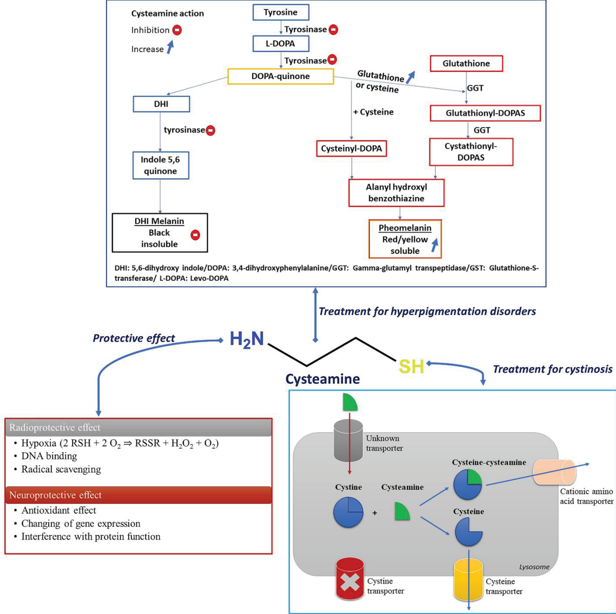
Figure 10: Cys pharmacodynamics.
