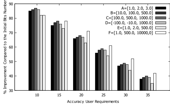
(c) Optimization of the number of bits compared to the original rotation matrix-vector multiplication program.
