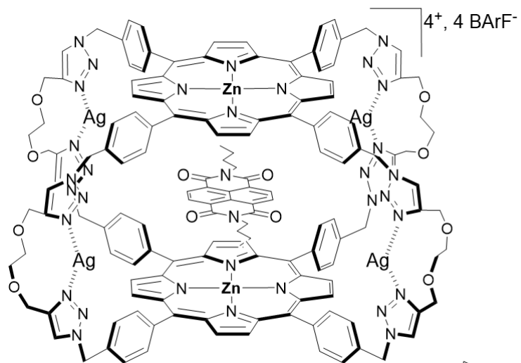
NDI@[Ag 4 C](BARF) 4
