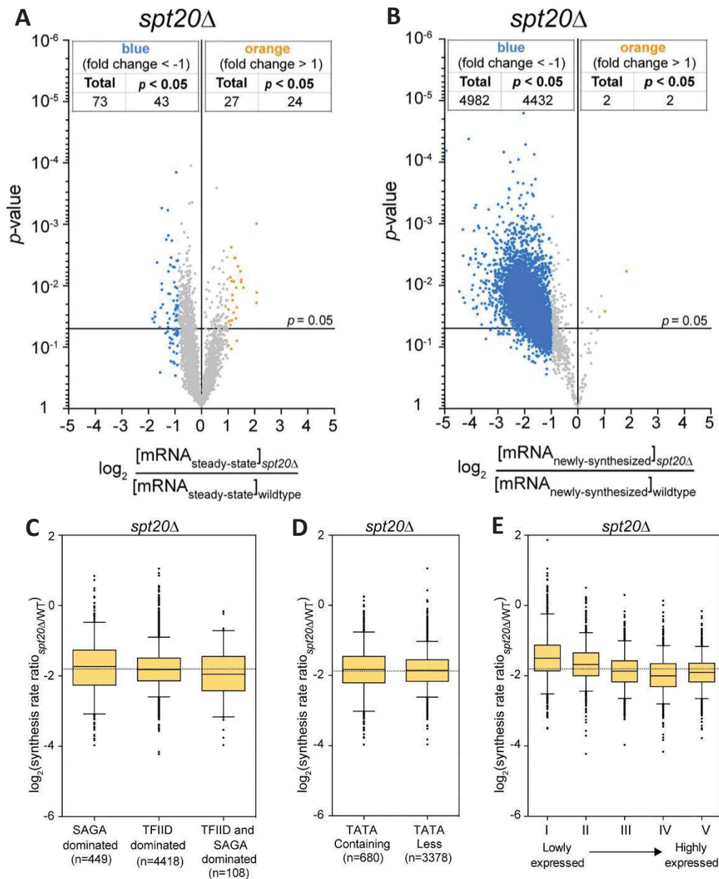
Figure 42: SAGA acts as a general cofactor for RNA polymerase II transcription in yeast. A. and B. Volcano plot representation of log 2 fold changes of steady-state mRNA levels (A) or newly synthesized mRNA levels (B) relative to their statistical significance (p-value) observed in spt20Δ strains compared to wildtype strains. Downregulated genes in blue, upregulated genes in orange. C., D. and E. Box plot representation of changes in newly synthesized RNA levels between spt20Δ and wildtype cells for different gene classifications. No obvious difference in degree of transcription changes could be observed whether genes were classified as SAGA- or TFIID-dominated (C) or if their promoters were TATA-box containing or TATA-less (D). In contrast, more highly expressed genes tended to have a more strongly reduced expression upon loss of Spt20 compared to lowly expressed genes (E). Adapted from Baptista et al., 2017.
