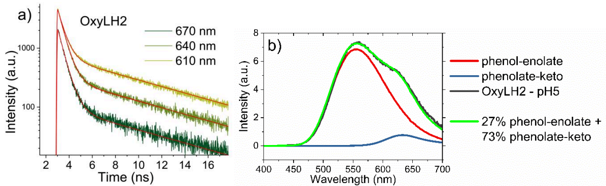
Figure S5: Excited-state keto-enol conversion a) Fluorescence decays measured for different emission wavelengths upon excitation at 430 nm (red curves correspond to the best fits obtained using the bi-exponential model: \tau_1 = 0.62 \text{ ns} and \tau_2 = 7.92 \text{ ns} ). b) Measured emission spectra of OxyLH 2 (black), of phenol-enolate (red) and phenolate-keto (blue). The two latter spectra were normalized as described above. The calculated steady-state emission spectrum (green curve) is obtained by using the relative concentrations of the phenol-enolate and phenolate-keto forms retrieved from the analytical model.
