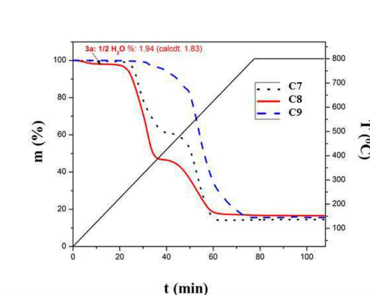
Figure 2-19. TGA traces for C7 – C9 complexes.
