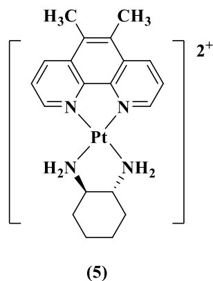
Figure 1-3. Schematic representation of [(5,6\text{-dimethyl-}1,10\text{-phen})(1\text{S},2\text{S-DACH})\text{Pt(II)}]\text{Cl}_2 .
