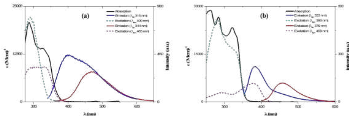
Figure 3-24. Absorption, emission and excitation spectra of: (a) C19 in diluted DMSO solution ( 1.2 \times 10^{-5} M) and (b) C20 in diluted \text{CHCl}_3 solution ( 6.1 \times 10^{-5} ).
