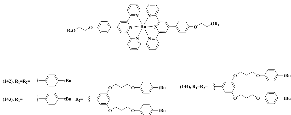
Figure 1-36. Structures of homo- and heteroleptic benzyl ether Ru(II) tpy dendrimers. Adapted from ref. 265 .
