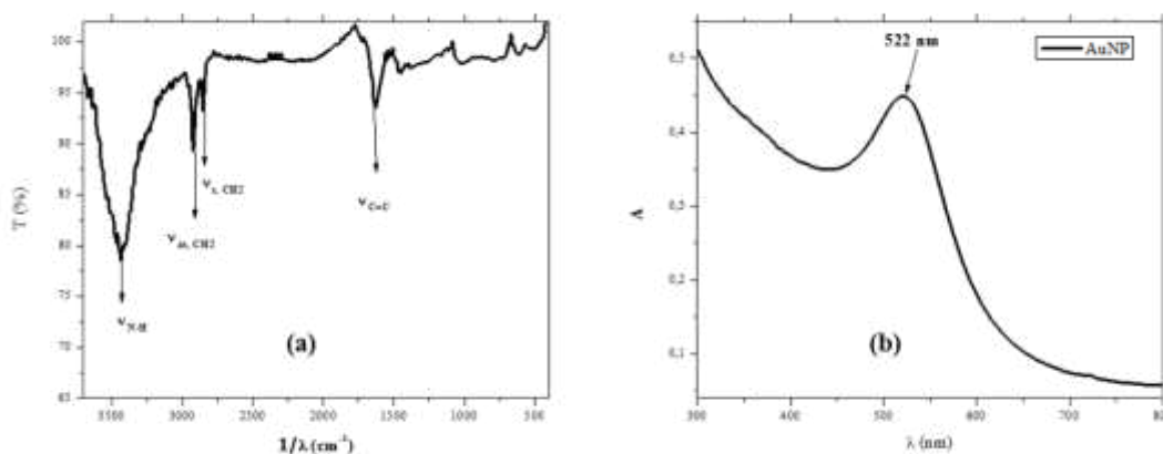
Figure 4-2. (a) FT-IR spectra of Au NPs and (b) UV-Vis spectra of Au NPs in CH 2 Cl 2 .
