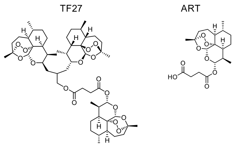
Figure1. Structures of artesunate (ART) and TF27, a trimeric derivative of ART
