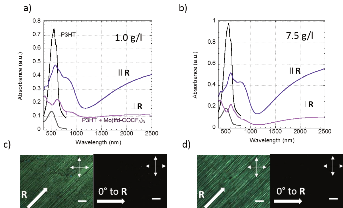
Figure 8. Polarized UV-vis-NIR absorbance spectra of rubbed P3HT and the same P3HT film sequentially doped with \text{Mo}(\text{tfd-COCF}_3)_3 , c_{\text{Mo}} \sim 1.0 \text{ g L}^{-1} (a) and c_{\text{Mo}} \sim 7.5 \text{ g L}^{-1} (b), measured parallel (||) and perpendicular ( \perp ) to the rubbing direction R. Corresponding polarised optical microscopy images (c, d) under crossed polariser and analyser 0^\circ and 45^\circ to the rubbing direction. White bold arrows indicate the rubbing direction R.
