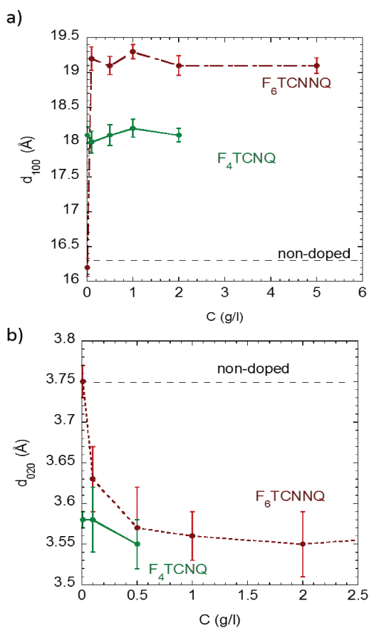
Figure 8. Evolution of the layer spacing along the alkyl side chain direction d_{100} (a) and the \pi -stacking periodicity (b) as a function of doping concentration. The curves in green (dark red) correspond to the F 4 TCNQ (F 6 TCNNQ) doped films.
