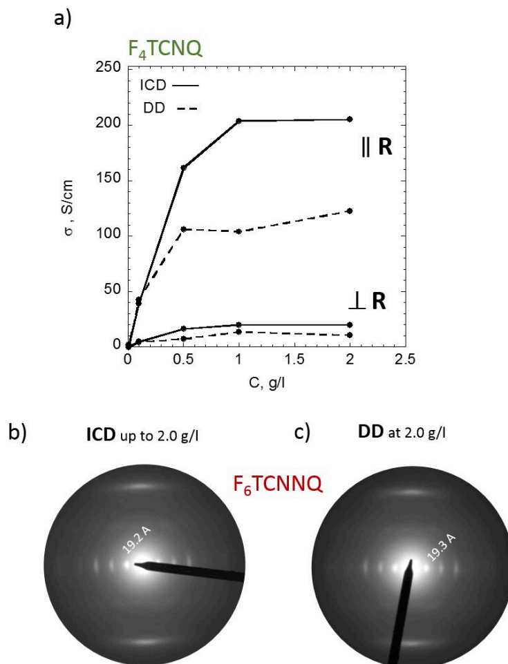
Figure 3. a) Electrical conductivity of oriented P3HT films doped by F_4TCNQ by both ICD and DD for comparison; b, c) Electron diffraction patterns of F_6TCNNQ -doped samples at 2 g/l using ICD and DD doping methods.
