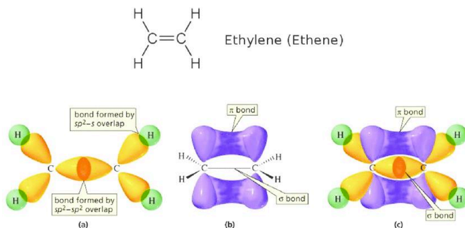
Figure 1.1 (a) Sigma (Single bond) hybridization for ethylene, (b) pi (Single bond) hybridization for ethylene and (c) both sigma and pi bond hybridization which give delocalization of pi-electron. Reproduced from the ref 5
