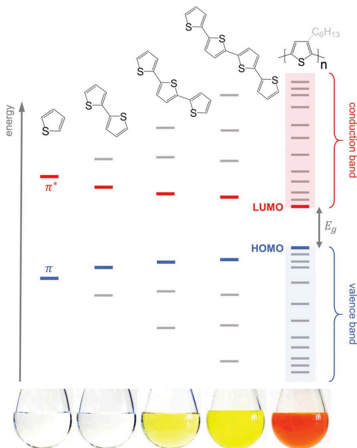
Figure 1.2 Evolution of the HOMO and LUMO levels as well as bandgap E_g with increasing number of thiophene repeat units, resulting in valence and conduction bands for polythiophene; the images of 5 g/l solutions in chloroform illustrate the narrowing of E_g ,
