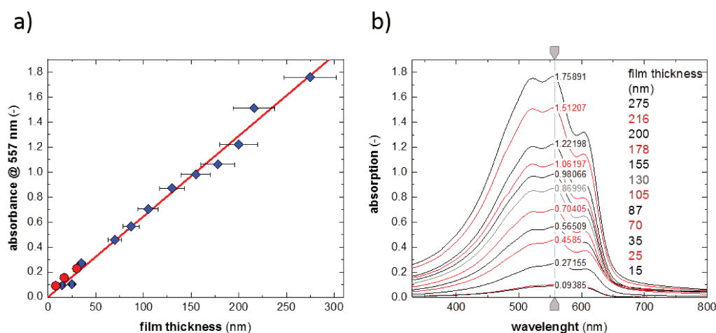
Figure E7. (a) Calibration curve for P3HT film thickness obtained by plotting the absorption at 557 nm versus film thickness. Average measurement deviation was \sim 5\% , error bars in the graph represent an error of 10%. Red circles: absorbance vs. thickness measured for films prepared with the P3HT batch used in this study ( M_w \sim 43.6 \text{ kg mol}^{-1} , RR \sim 95.9\% , PDI \sim 1.8 ) obtained from AFM measurements; Blue diamonds: absorbance vs. thickness measured for films prepared with other P3HT batch ( M_w \sim 63.8 \text{ kg mol}^{-1} , RR \sim 96\% , PDI \sim 2.2 ) of spectra shown in b); (b) Representative absorption spectra of spin-coated P3HT ( M_w \sim 63.8 \text{ kg mol}^{-1} , RR \sim 96\% , PDI \sim 2.2 ) from a 1:1 mixture of chlorobenzene:oDCB, the concentration of P3HT was varied from 2 to 30 \text{g L}^{-1} to obtain films with different thicknesses. The UV-vis absorption spectra were measured with a Pekin Elmer Lambda 950 spectrophotometer and the thickness was measured with a KLA Tencor AlphaStep D-100 profilometer. Both methods show a good agreement for both batches.
