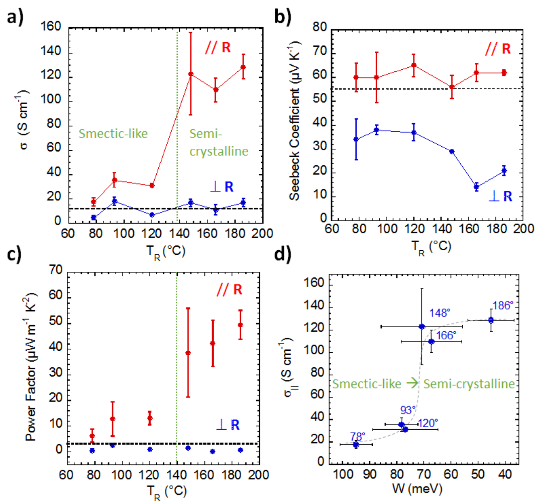
Figure 7: Evolution of the a) charge conductivity, b) Seebeck Coefficient, and c) power factor measured along (// R) or perpendicular ( \perp R) to the rubbing direction for P3HT films rubbed at different temperatures and doped with F 4 TCNQ (1 mg/ml). The black dashed lines represent the values for a non-oriented sample. The error bars are mainly related to the statistic dispersion in alignment level of samples. In a and c, the vertical green lines are a guide for the eye to differentiate the ranges of smectic-like and semi-crystalline phases. d)
