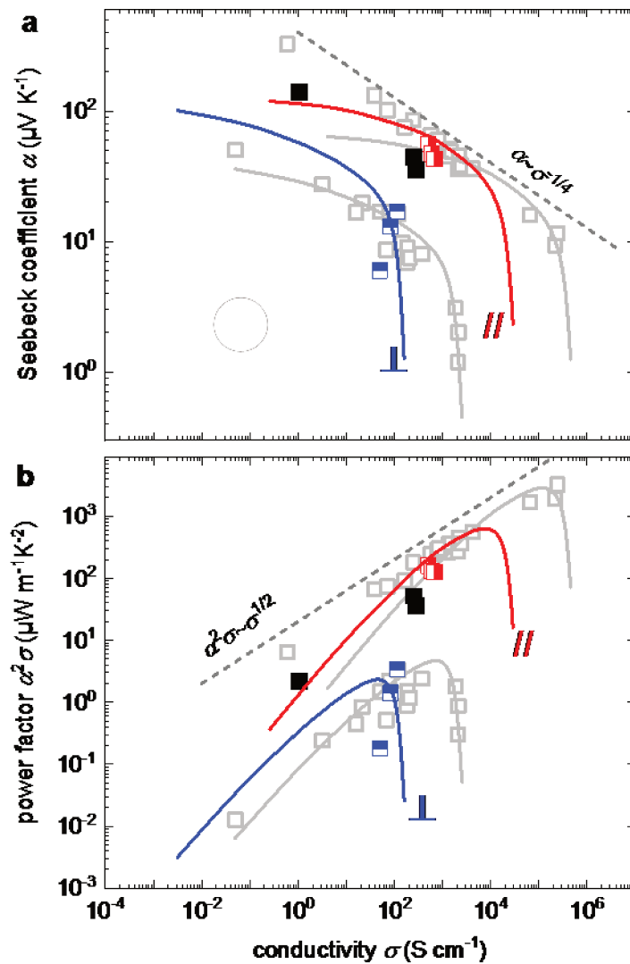
Figure 12. (a) Seebeck coefficient \alpha and (b) power factor \alpha^2\sigma versus electrical conductivity \sigma of isotropic P3HT (black squares), and rubbed P3HT measured parallel (red squares and line) and perpendicular to the rubbing direction (blue squares and line); grey data points are literature values extracted from refs for PBTTT 9,40 . Full lines correspond to simulations calculated from the kMC model, with an anisotropy ratio of \xi_{\parallel}/\xi_{\perp} = 4 , where \xi is the localization
