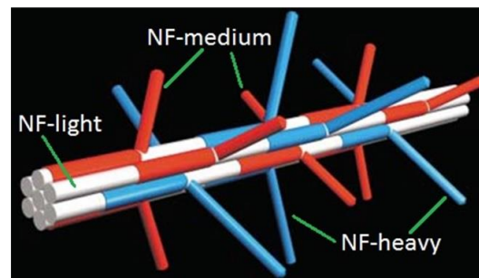
Figure 1.11: Structure of neurofilament (Smith and Meaney, 2000).
