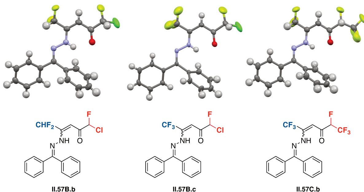
Figure II.18: Crystallographic analyses of single crystals of compounds II.57B.b (left), II.57B.c (centre, unpublishable) and II.57C.b (right).
