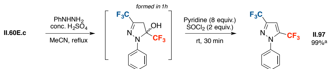
Scheme II.28: Preparation of the corresponding bis(fluoroalkyl) pyrazoles from both unprecedented vinamides II.60E.b and II.60E.c (top); facile synthesis of a challenging bis-CF 3 -pyrazole reported in the literature (bottom)
