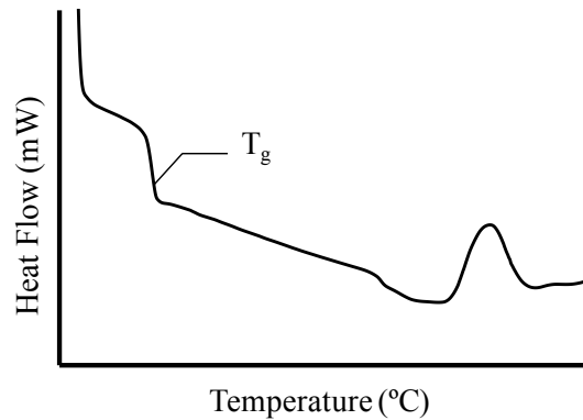
Figure 7 – Graph displaying a common DSC trace of an elastomer ( T_g = glass transition temperature).
