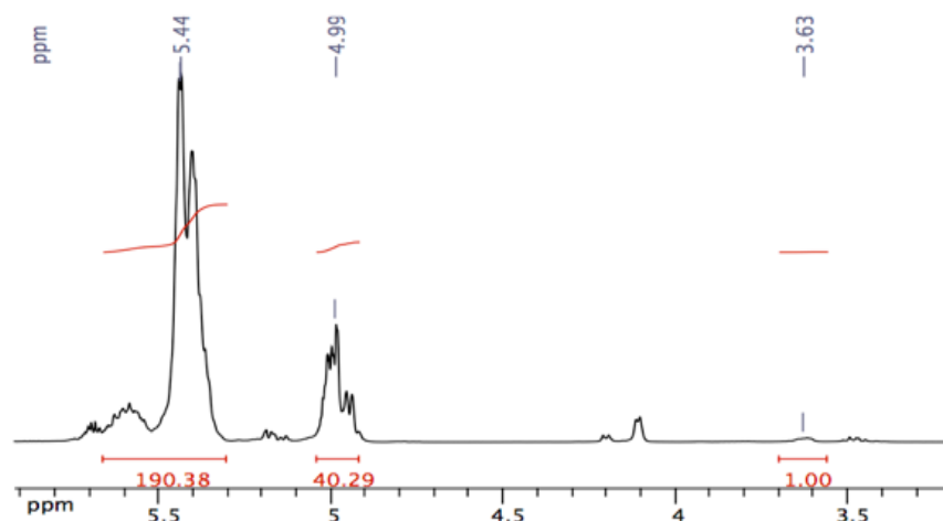
Figure 48 – Partial ^1\text{H} NMR spectrum of Polyvest ® EPHT displaying proton resonances from cis/trans -1,4 ( \delta 5.44) and 1,2 ( \delta 5.44 and 4.99) microstructures integrated to the -\text{CH}_2\text{OH} resonance ( \delta 3.63)
