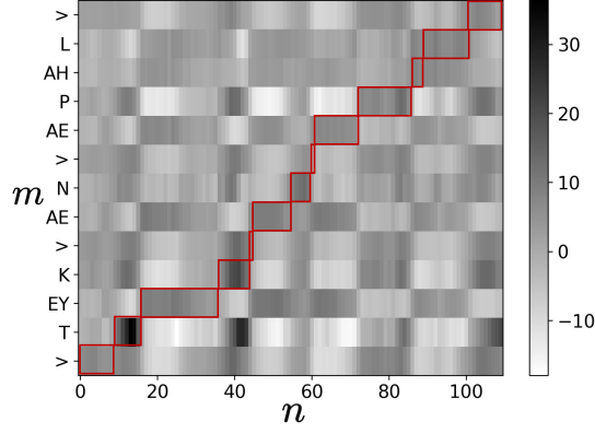
Figure 5.3: Example of a score matrix \mathbf{S} = [s_{m,n}]_{m,n} with optimal DTW path in red which assigns one phoneme to each audio frame.
