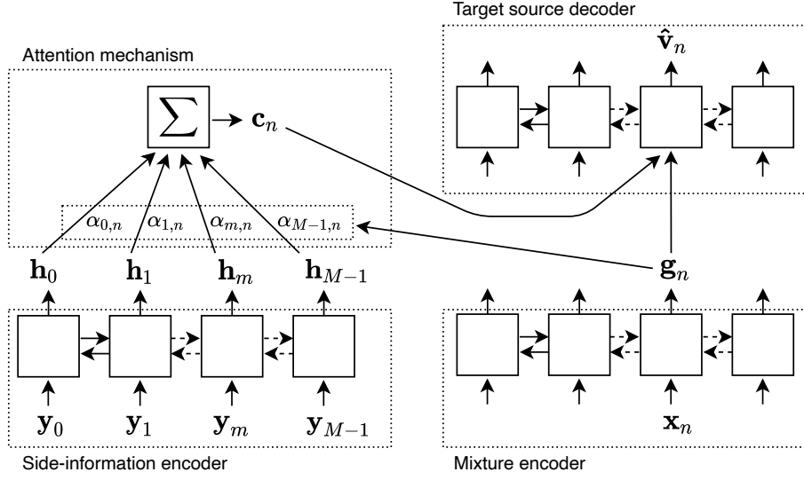
Figure 4.1: Schematic model architecture and workflow of the attention mechanism to compute the n -th prediction frame \hat{v}_n .
