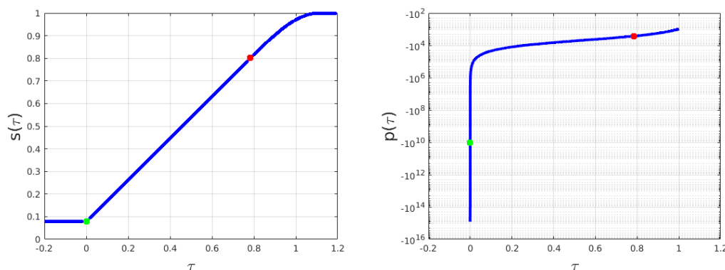
Figure 4.1: Plot of saturation and pressure parametrized van Genuchten-Mualem curves, using values of rock type 1 reported in Table 4.2. The green dot indicates the value for \tau = \tau_* and the magenta one \tau = \tau_s .
