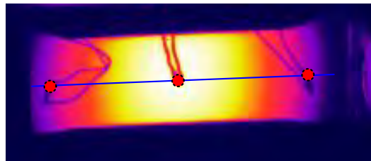
Figure 5: Temperature field for the test V2 captured by the thermal camera. The highest temperatures are represented in yellow and the lowest by the violet. The line passing through the mid-plane of the specimen ( y = 0 mm) is represented in blue and the thermocouples position by the red circles.
