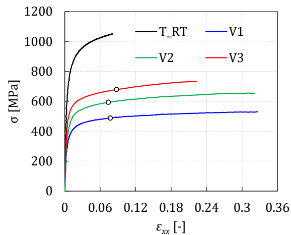
Figure 9: Stress vs strain curves computed for a central section of the specimens. The colour lines correspond to 500 °C. The black curve (T_RT) corresponds to room temperature obtained from a homogeneous tensile test [22].
