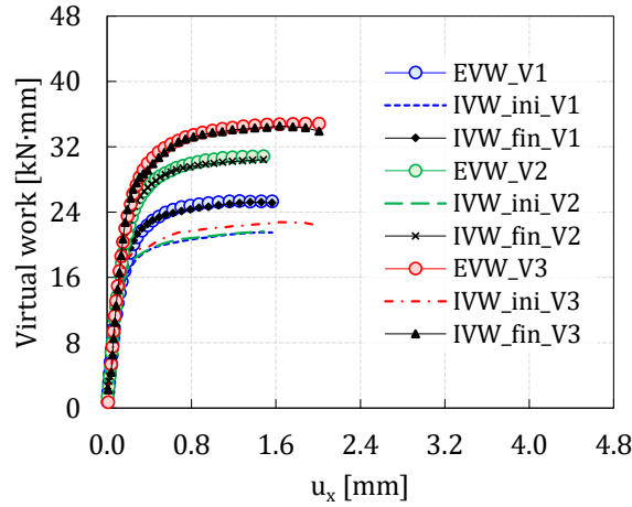
Figure 11: Internal virtual work (IVW) vs external virtual work (EVW). The IVW is plotted for the initial (IVW_ini) and final (IVW_fin) sets of parameters using the first virtual field \mathbf{U}_1^* .
