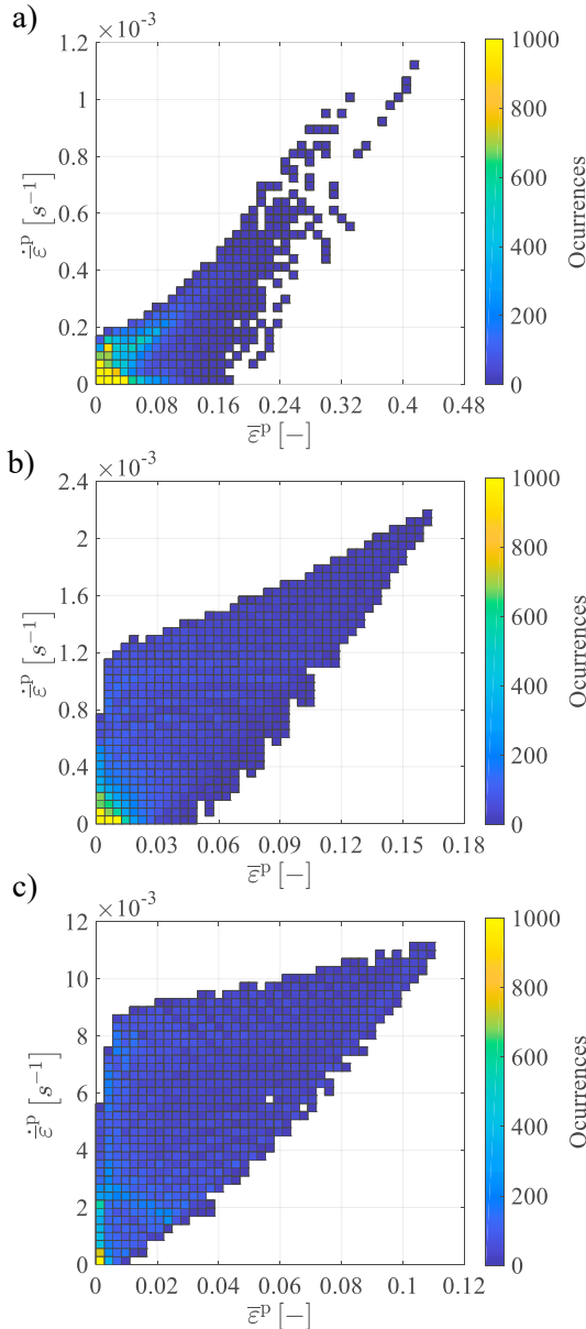
Fig. 5. Equivalent plastic strain rate versus equivalent plastic strain for the complete deformation process of the heterogeneous tests. Three different average strain rates: a) 10^{-4} \text{ s}^{-1} , b) 10^{-3} \text{ s}^{-1} and c) 10^{-2} \text{ s}^{-1} .
