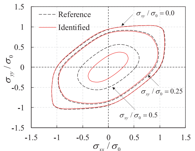
Fig. 14. Comparison of the reference yield locus with the identified yield locus for different levels of \sigma_{xy}/\sigma_0 .
