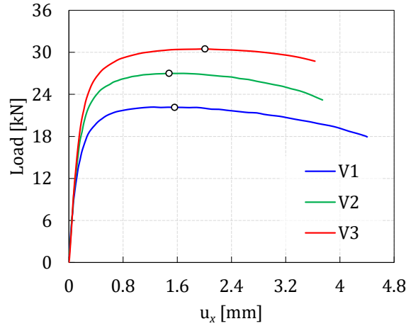
Figure 2: Load vs displacement ( u_x ) curves for the three displacement rates: 0.006, 0.06 and 0.6 mm s -1 , which correspond to V1, V2 and V3, respectively.
