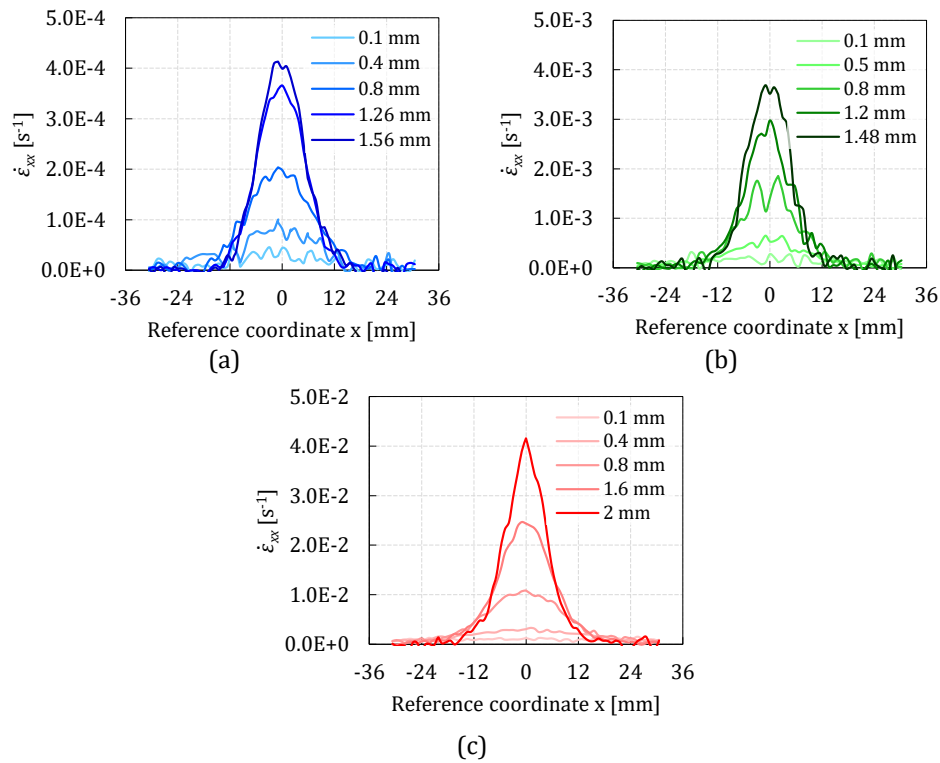
Figure 8: Strain-rate ( \dot{\epsilon}_{xx} ) distribution along the mid-plane y=0 mm in the ROI and, for the tests a) V1, b) V2 and c) V3.
