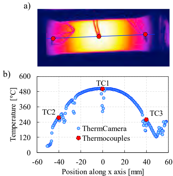
Fig. 2. Temperature field obtained during a test in a Gleeble equipment: a) thermographic camera measurement and b) temperature along a line and thermocouples measurements on the specimen's surface.
