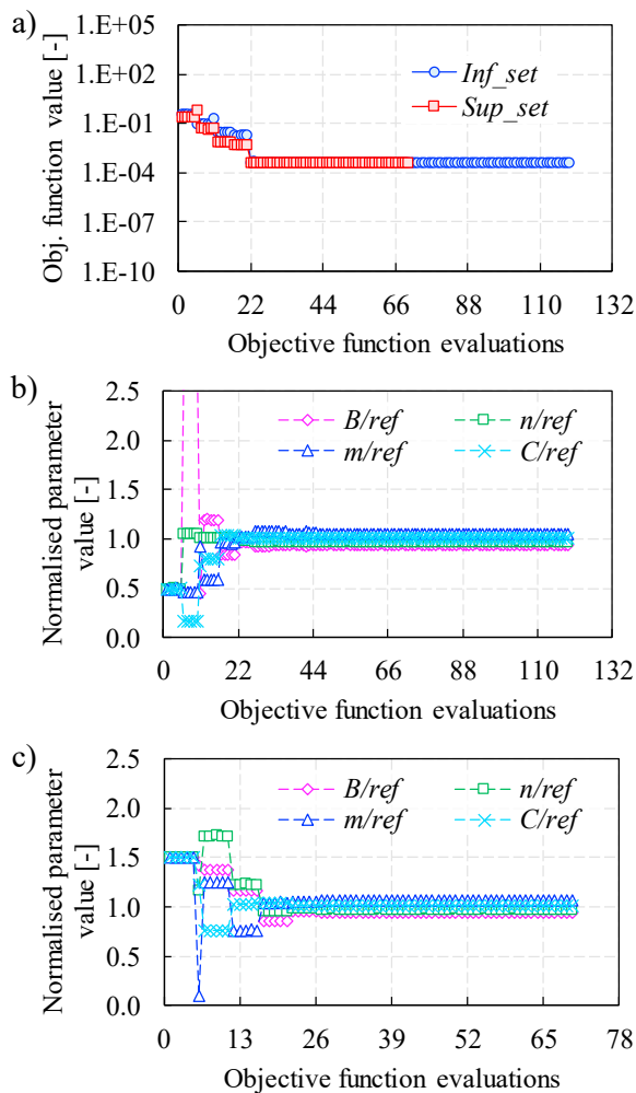
Fig. 8. Results for the identification with a virtual database with noise, assuming a fixed value for parameter A : a) evolution of the objective function for two different initial sets, b) and c) evolution of the material parameters for the Inf_set and Sup_set initial sets, respectively.
