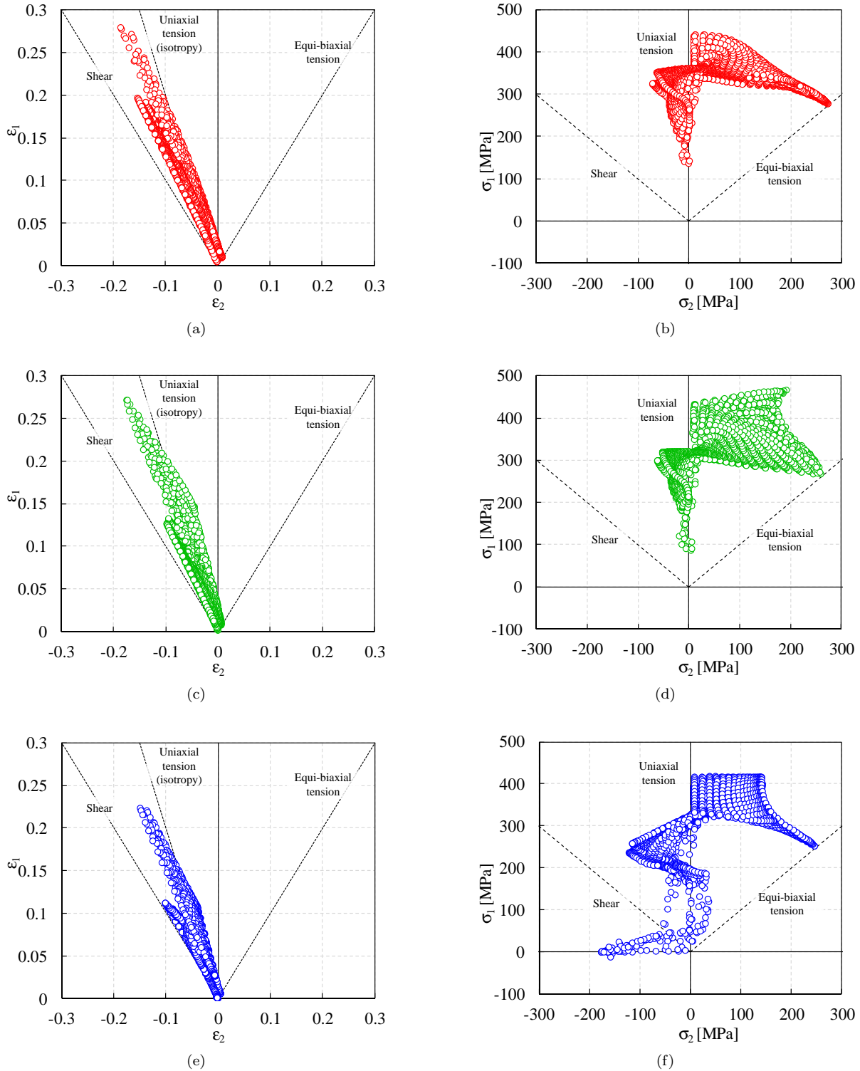
Fig. 4. Plot of the principal strain and stress fields at the end of the tests: (a) and (b) Cr1, (c) and (d) Cr2, and (e) and (f) Cr3.
