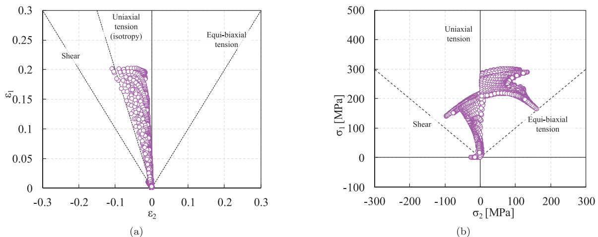
Fig. 11. Plot of the strain (a) and stress (b) fields at the end of the test in the principal axes, corresponding to the model of Fig. 10.
