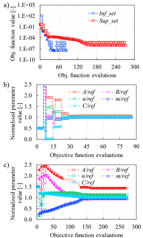
Fig. 6. Results for the identification with a virtual database without noise: a) evolution of the objective function for two different initial sets, b) and c) evolution of the material parameters for the Inf_set and Sup_set initial sets, respectively.
