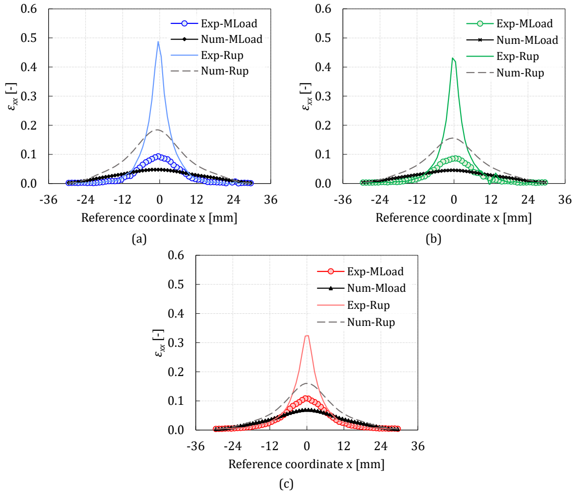
Figure 20: Comparison of experimental (Exp) and numerical (Num) spatial distribution of the logarithmic strain in the x -direction. The numerical results are obtained through FE analysis with the final set of parameters presented in Table 2: (a) V1, (b) V2 and (c) V3.
