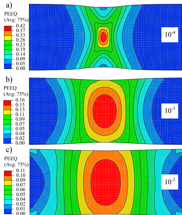
Fig. 4. Equivalent plastic strain (PEEQ) distribution for the last instant of each test, which correspond to 958 s, 107s and 11.75 s. Three different average strain rates: a) 10^{-4} \text{ s}^{-1} , b) 10^{-3} \text{ s}^{-1} and c) 10^{-2} \text{ s}^{-1} .
