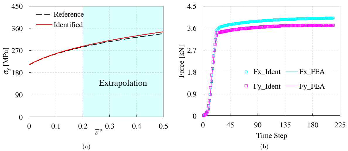
Fig. 13. Results obtained with the identified parameter set Sup_set of Table 6: (a) plot of Swift's law and (b) force prediction based on the internal work.
