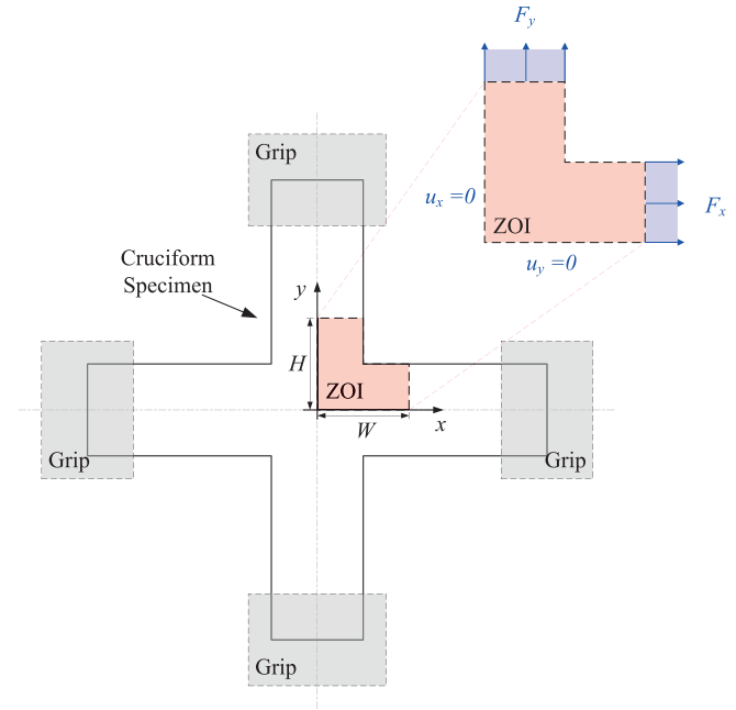
Fig. 1. Illustrative example of a biaxial test with a cruciform specimen and the respective zone of interest (ZOI) selected for the present study.
