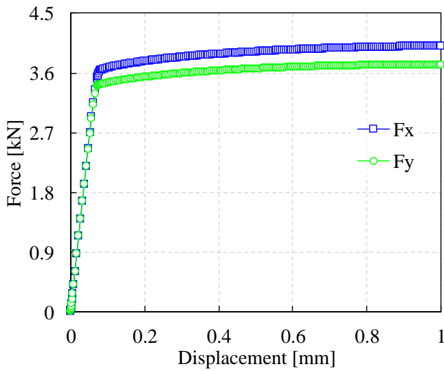
Fig. 12. Force vs displacement for the two arms of the model of Fig. 10.
