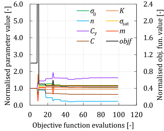
Figure 16: Evolution of the material parameters and objective function value ( objf ) during the calibration process for the experimental database composed by three tests. The values of the parameters and objective function are normalised by the initial value.
