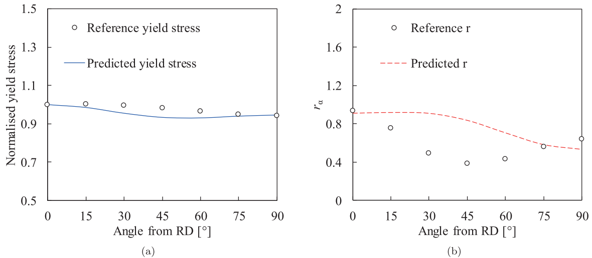
Fig. 15. Evolution of the (a) normalised yield stress and (b) plastic anisotropy coefficient according to the tension axis angle from the rolling direction for the parameters identified with Cr3 and the aluminium alloy.
