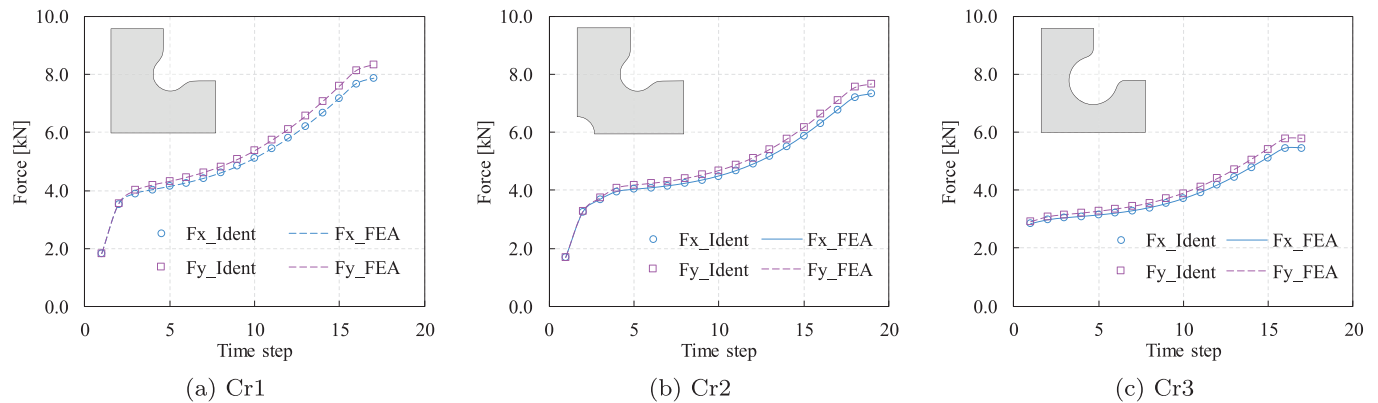
Fig. 7. Comparison between computed force from the identified parameters ( F_{x\_Ident} and F_{y\_Ident} ) and the resultant force from the FE analysis for the three geometries ( F_{x\_FEA} and F_{y\_FEA} ) for x and y -directions.
