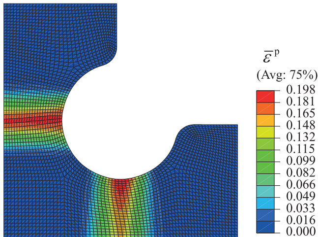
Fig. 10. Equivalent plastic strain distribution for the last increment and the deformed FE mesh for Cr3 using the YLD2000-2d yield criterion and the material parameters of Table 2.
