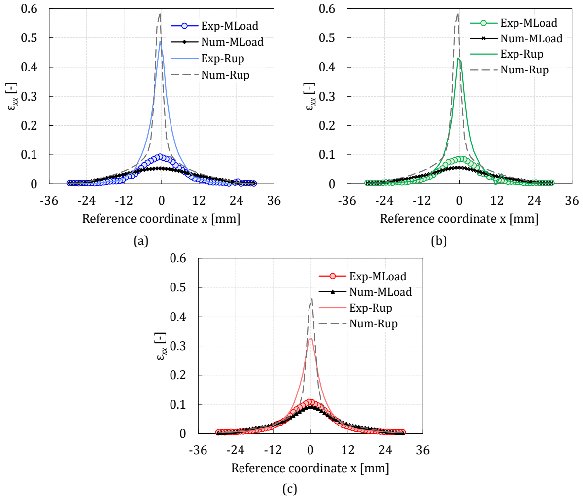
Figure 15: Comparison of experimental (Exp) and numerical (Num) spatial distribution of the logarithmic strain along the x -direction. The numerical results are obtained through FE analysis with the obtained sets of parameters presented in Table 1: (a) V1, (b) V2 and (c) V3.
