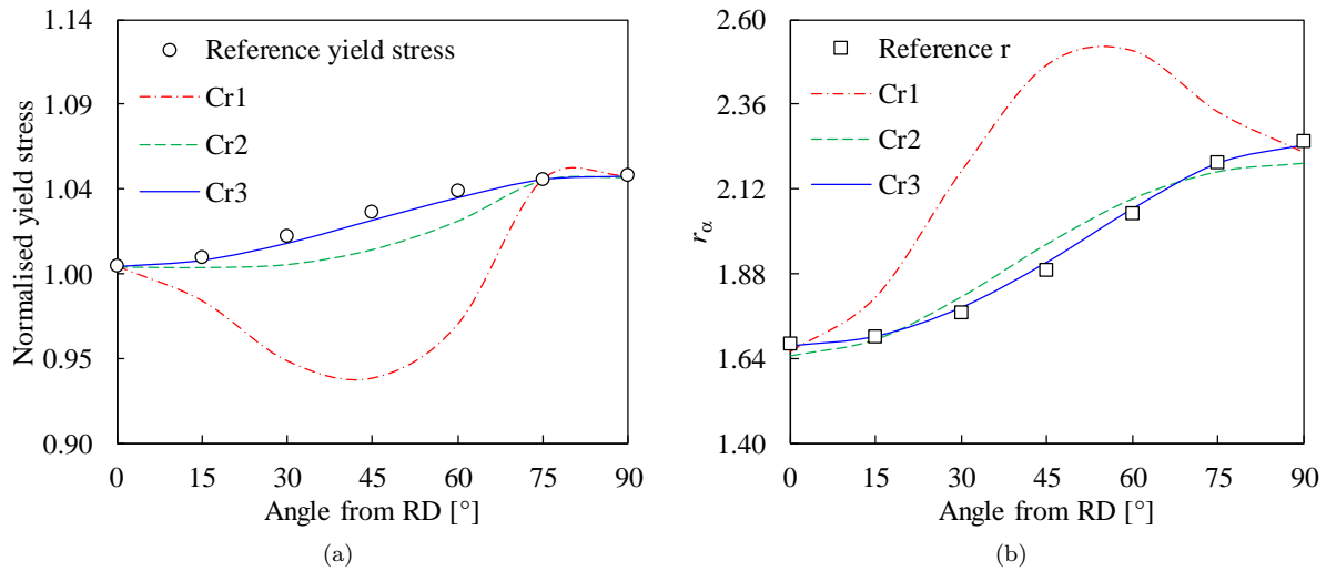
Fig. 8. Evolution of the (a) normalised yield stress and (b) plastic anisotropy coefficient according to the tension axis angle from the rolling direction for the identified parameters with Cr1, Cr2 and Cr3.
