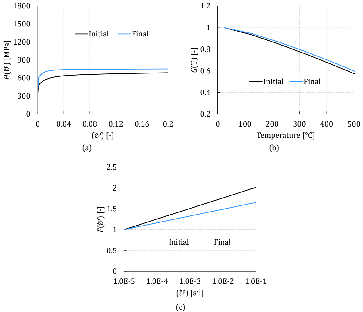
Figure 18: Evolution of three terms that compose the modified J-C model using the final set of parameters presented in Table 2: (a) strain-hardening term (Eq. 2), (b) temperature term (Eq. 3) and (c) strain-rate term (Eq. 4).
