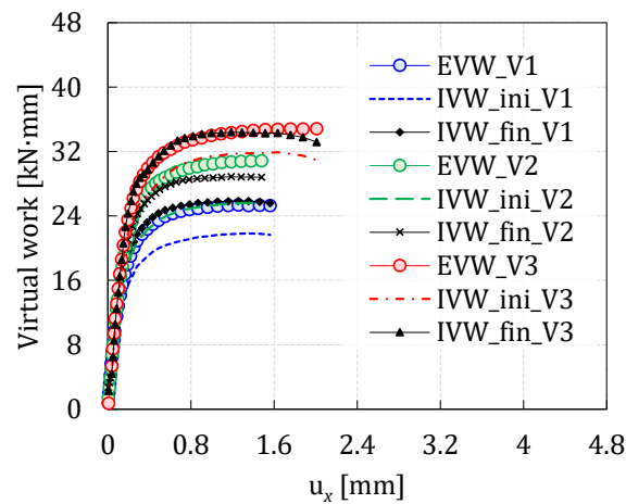
Figure 17: Internal virtual work (IVW) vs external virtual work (EVW). The IVW is plotted for the initial (IVW_ini) and final (IVW_fin) sets of parameters using the first virtual \mathbf{U}_1^* .
