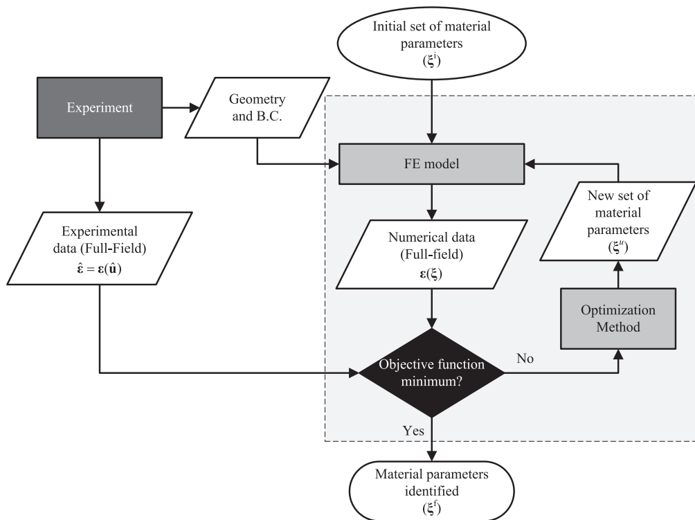
Fig. 2. Detailed flowchart for the FEMU.
