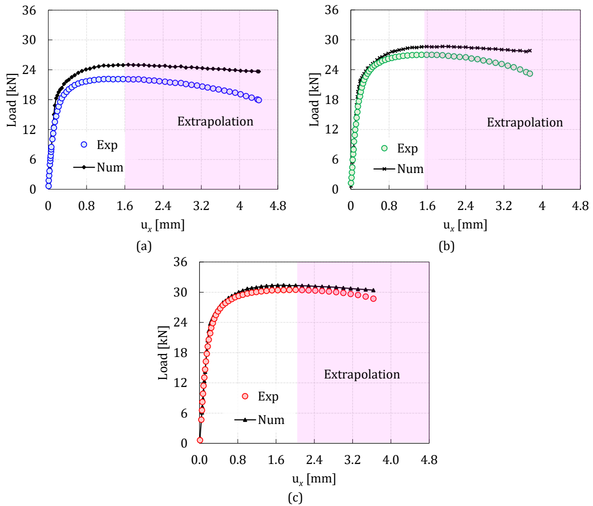
Figure 19: Comparison of experimental (Exp) and numerical (Num) load curves. The numerical load curves are obtained through FE analysis with the final set of parameters presented in Table 2: (a) V1, (b) V2 and (c) V3.
