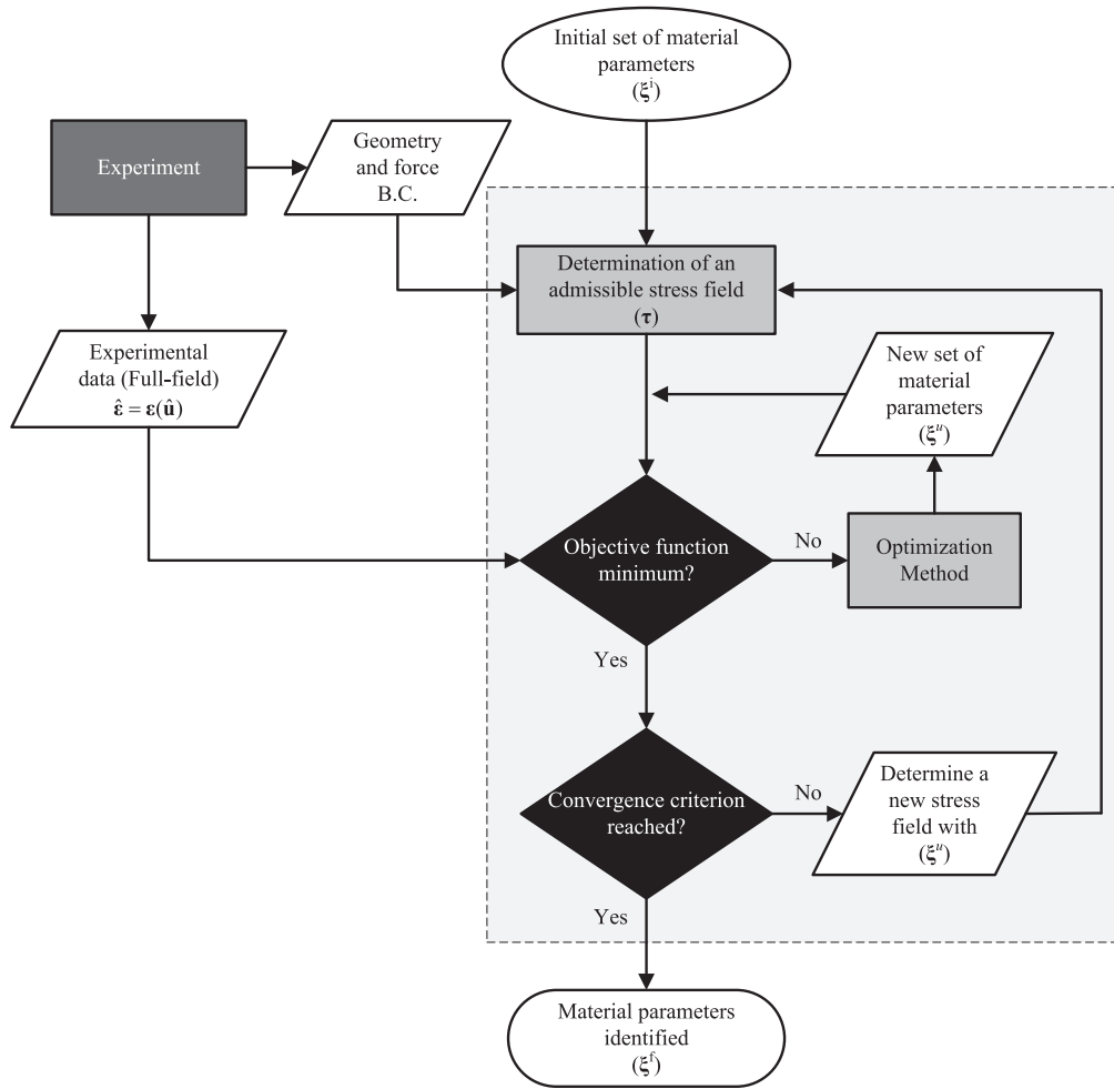
Fig. 3. Detailed flowchart for the CEGM.
