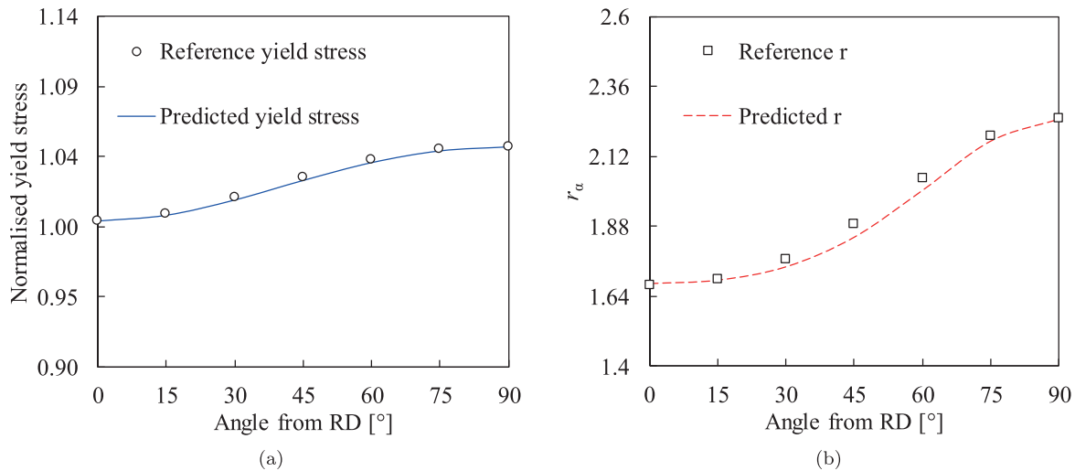
Fig. 16. Evolution of (a) the normalised yield stress and (b) plastic anisotropy coefficient according to the tension axis angle from the rolling direction for the parameters identified with Cr3 and mild steel.
