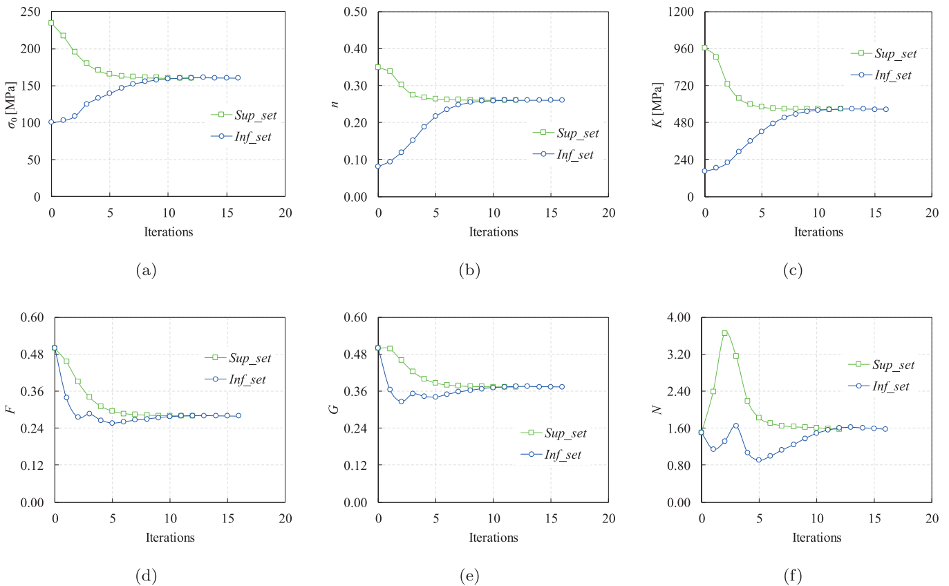
Fig. 9. Evolution of the identified parameters for Cr3 during the optimisation process.
