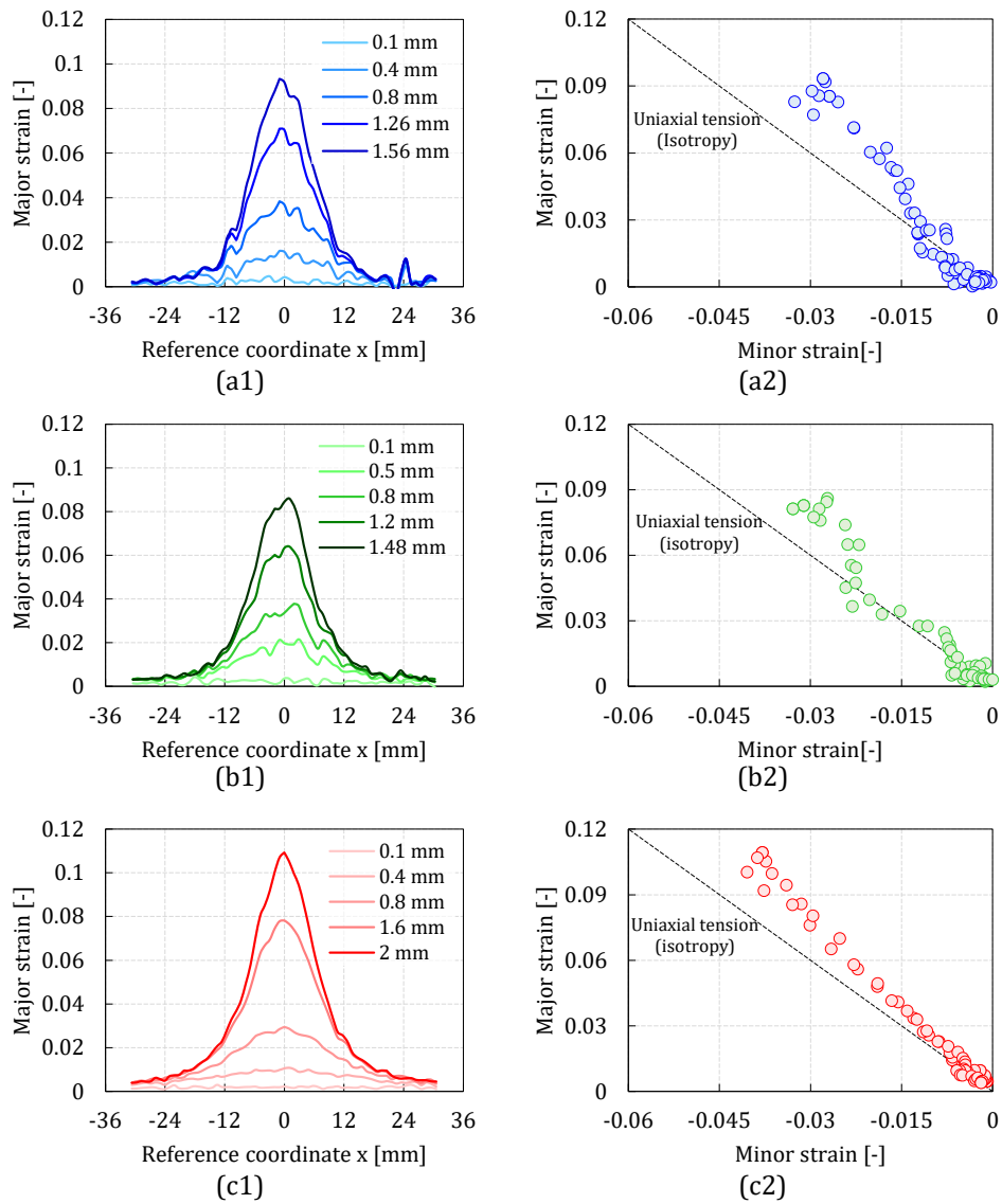
Figure 7: Major strain distribution and major strain vs minor strain along the mid-plane y = 0 mm for the ROI, for the tests a) V1, b) V2 and c) V3.
