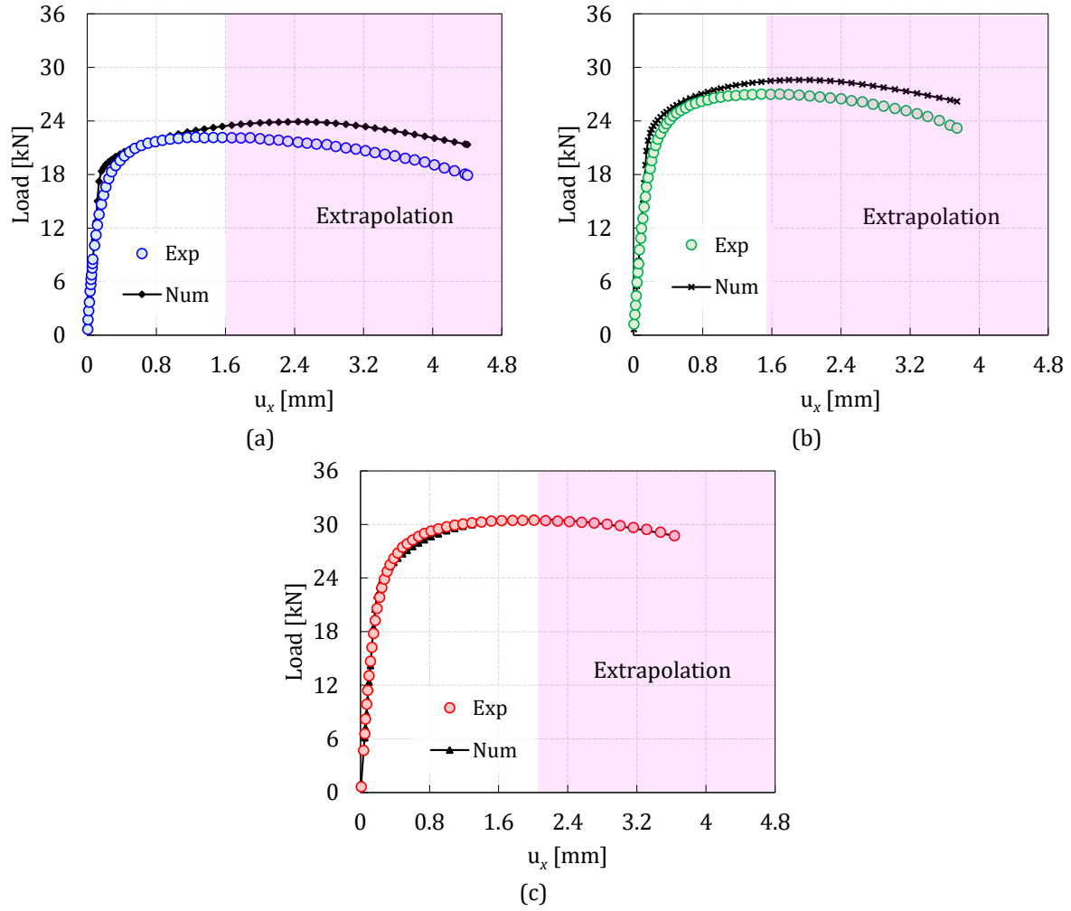
Figure 14: Comparison of experimental (Exp) and numerical (Num) load curves. The numerical load curves are obtained through FE analysis with the final sets of parameters presented in Table 1: (a) V1, (b) V2 and (c) V3.
