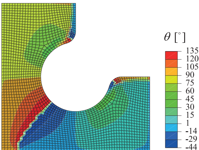
Fig. 5. Rotation angle between principal stress base and material frame for Cr3.
