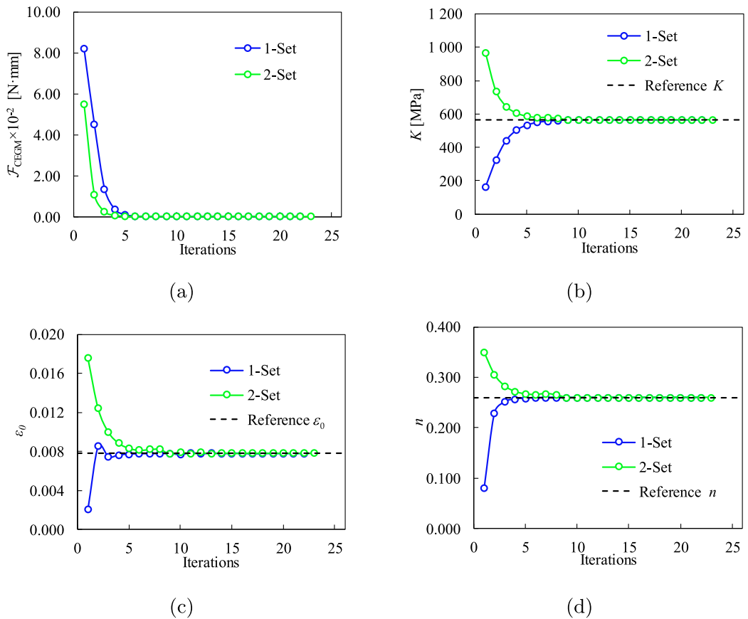
Fig. 11. Results of the identification process for CEGM strategy: (a) objective function evolution; parameters (b) K ; (c) \epsilon_0 and (d) n evolutions.
