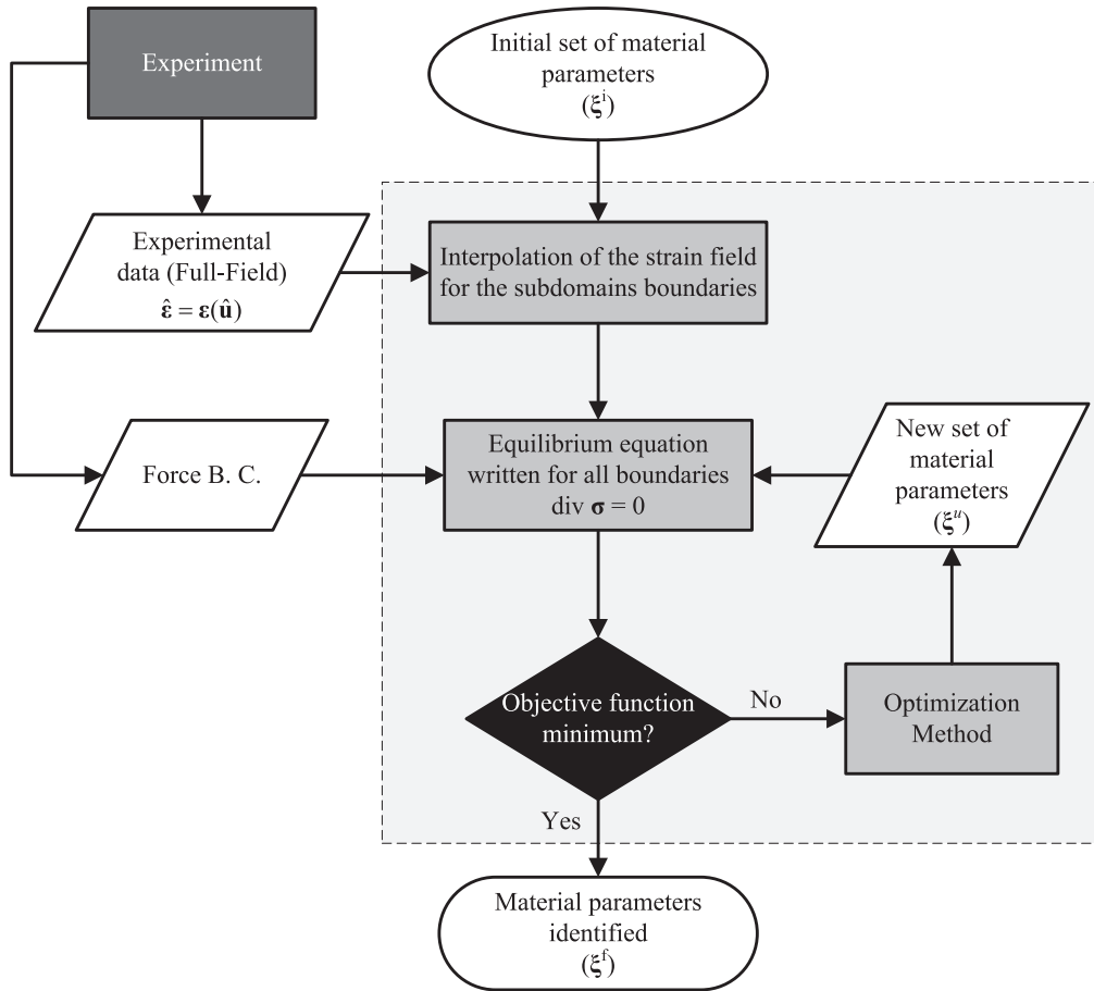
Fig. 5. Detailed flowchart for the EGM.
