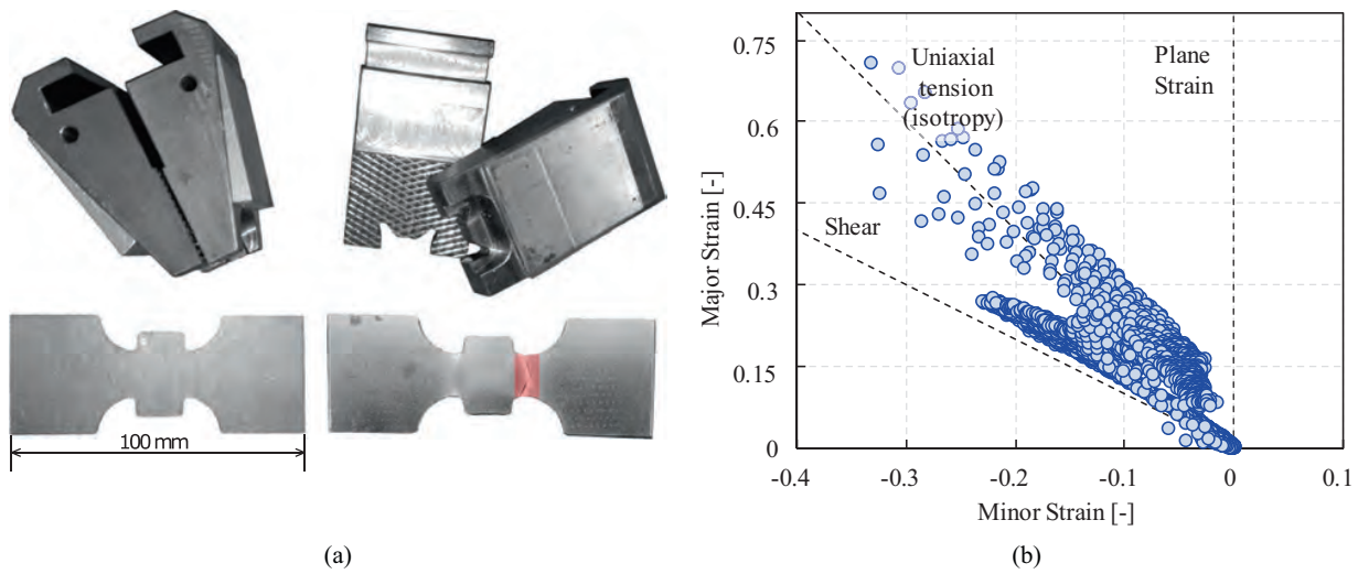
Fig. 5.1 (a) Grips and specimen used for the adapted butterfly test and (b) principal strains distribution for a tool displacement of 7.1 mm
