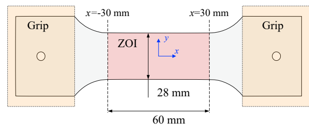
Fig. 1. Schematic representation of the specimen for the heterogeneous thermo-mechanical test and its respective ZOI.
