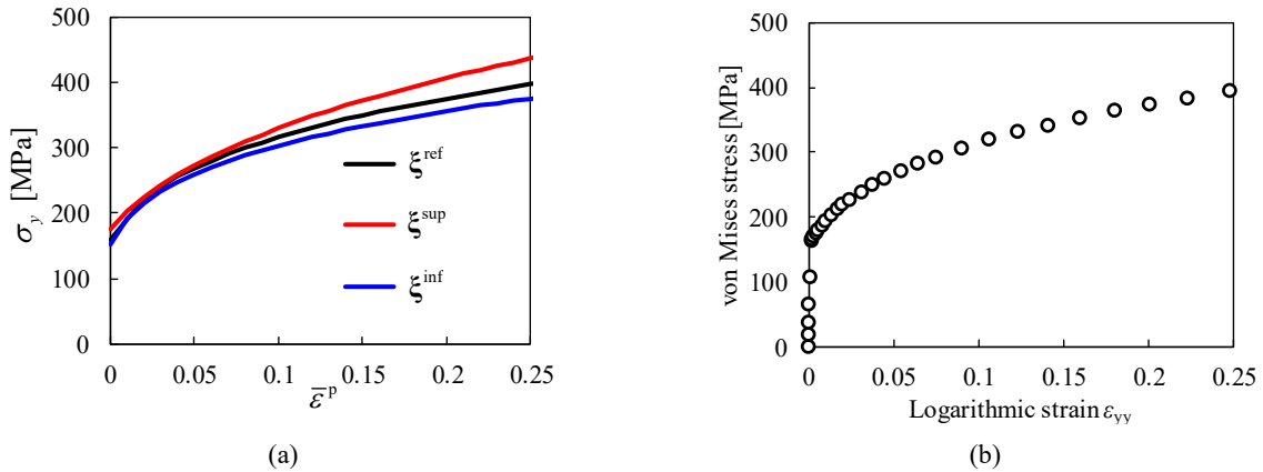
FIGURE 2. Swift's law plotted for the solutions obtained with FEMU strategy (see Table 1) (a) and stress-strain curve obtained with the reference set of parameters for the nearest element to the centre of the specimen presented in Fig. 1(b).
