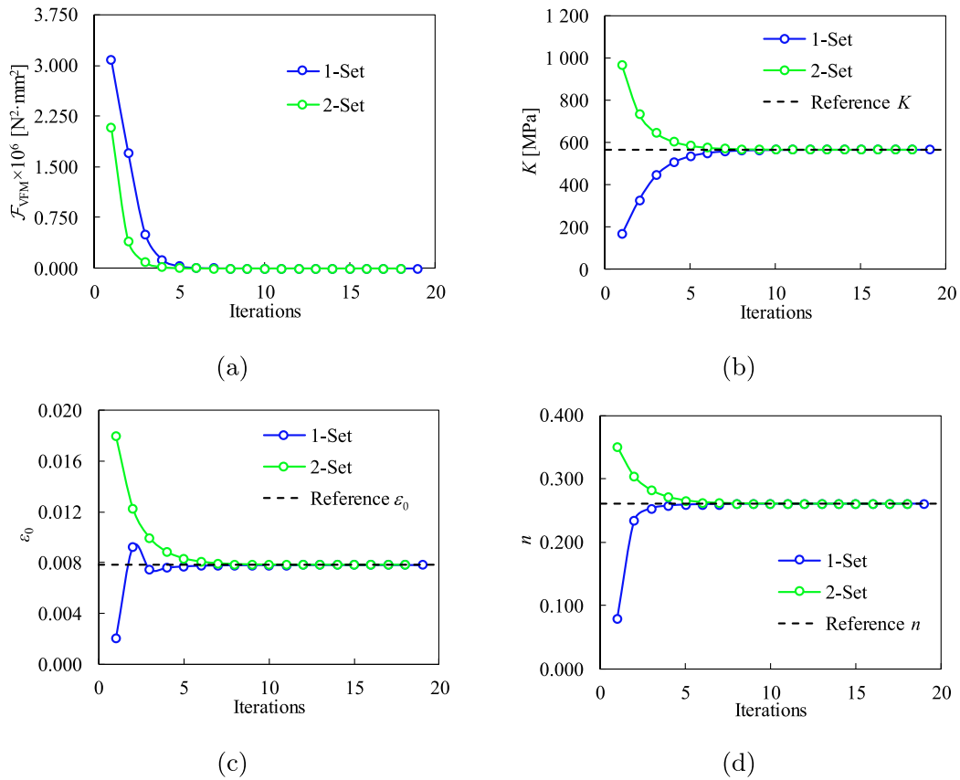
Fig. 10. Results of the identification process for VFM strategy: (a) objective function evolution; parameters (b) K ; (c) \epsilon_0 and (d) n evolutions.
