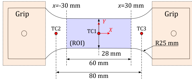
Figure 1: Geometry of the tensile specimen, region of interest (ROI) and position of the thermocouples.
