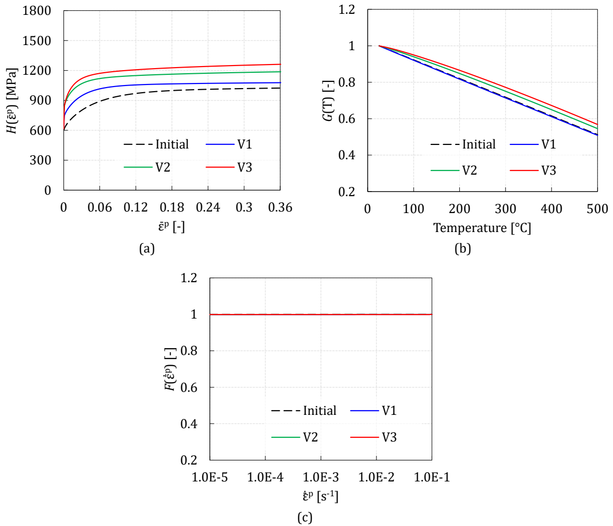
Figure 12: Evolution of three terms that compose the modified J-C model using the obtained sets of parameters presented in Table 1: (a) strain-hardening term (Eq. 2), (b) temperature term (Eq. 3) and (c) strain-rate term (Eq. 4).
