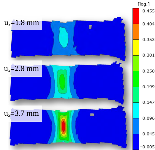
Figure 6: Major strain distribution for the test V2.
