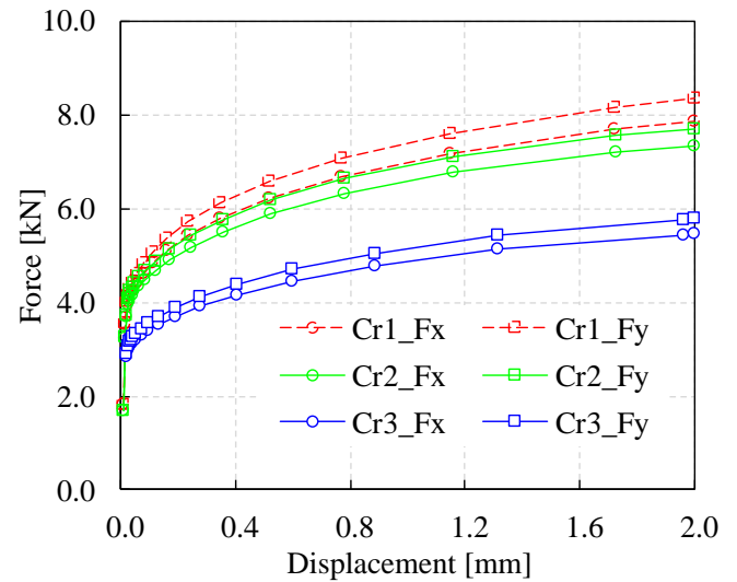
Fig. 6. Force vs displacement for the three geometries: Cr1, Cr2 and Cr3.
