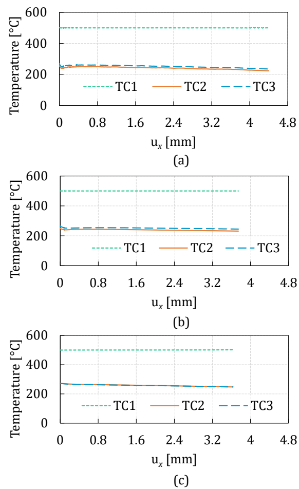
Figure 3: Temperature measurements acquired by the three thermocouples TC1, TC2 and TC3, for the tests: a) V1, b) V2 and c) V3.
