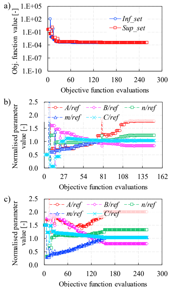
Fig. 7. Results for the identification with a virtual database with noise: a) evolution of the objective function for two different initial sets, b) and c) evolution of the material parameters for the Inf_set and Sup_set initial sets, respectively.
