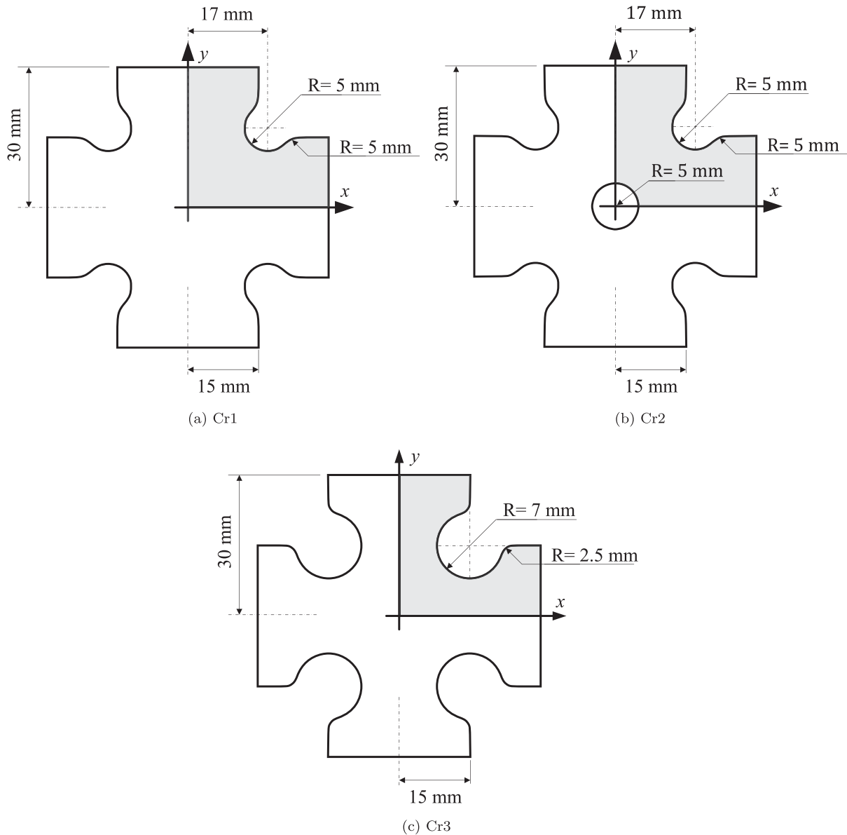
Fig. 2. Cruciform geometries: (a) Cr1 has been proposed by Zhang et al. (2014), (b) Cr2 and (c) Cr3 are adaptations of Cr1. The grey areas represent the geometry of the FE model.
