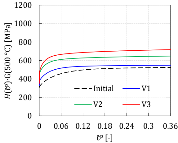
Figure 13: Evolution of the strain-hardening term (Eq. 3) affected by the temperature term (Eq. 3) at 500 °C for the final sets of parameters presented in Table 1.
