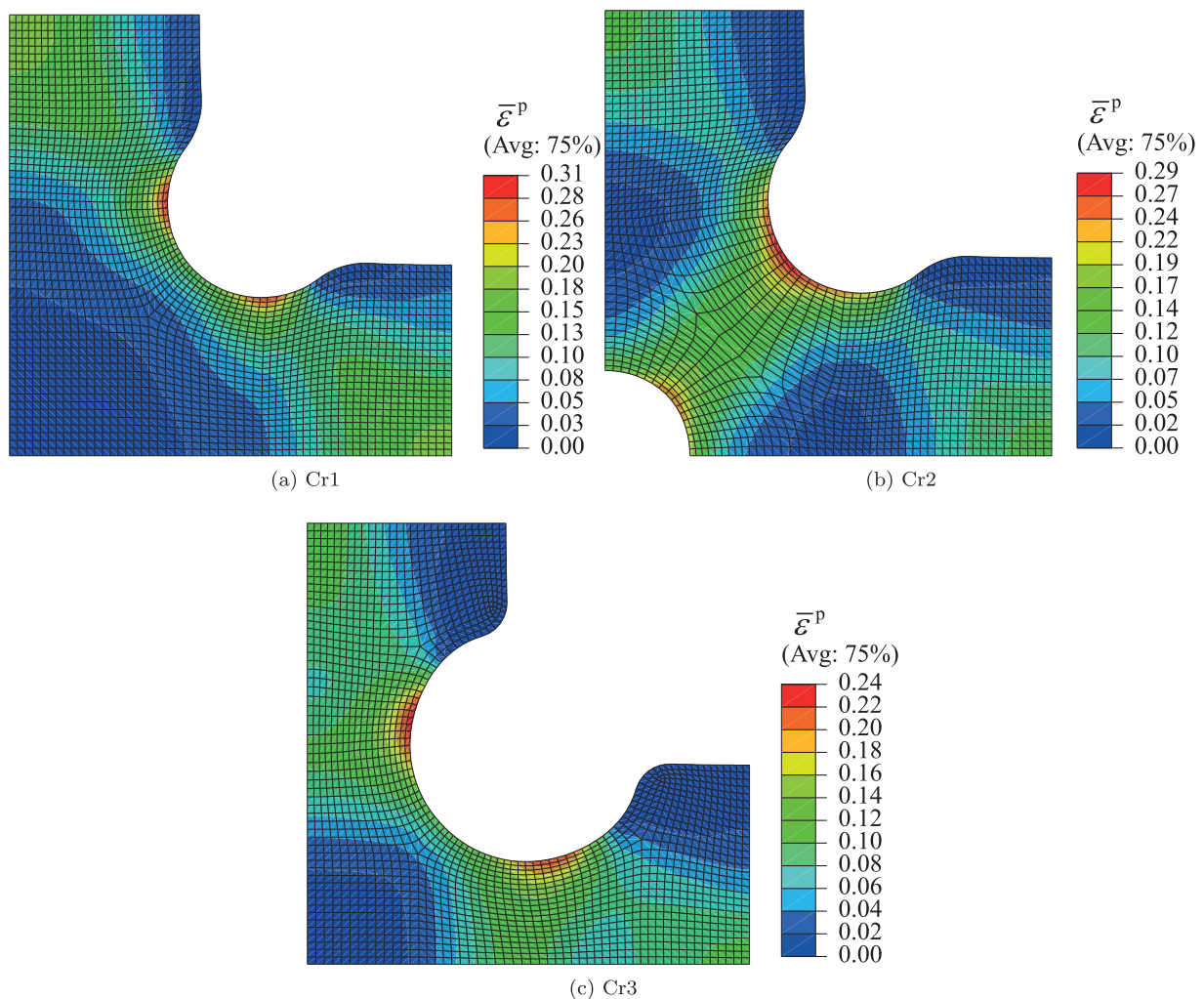
Fig. 3. Equivalent plastic strain distribution for the last increment and deformed FE mesh for the three geometries.
