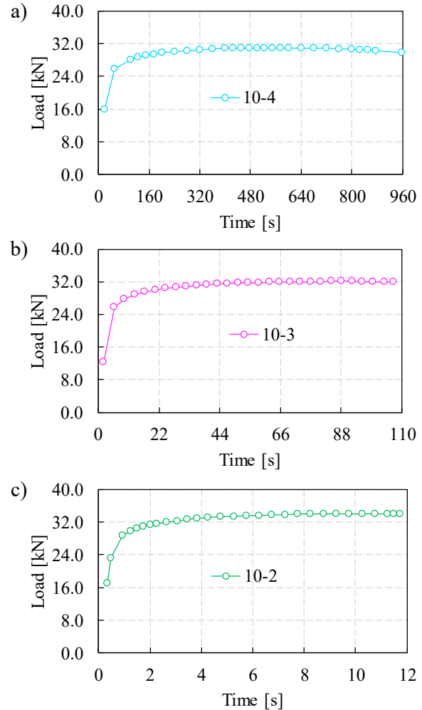
Fig. 3. Load signals of the heterogeneous thermo-mechanical tests performed at three different average strain rates: a) 10^{-4} s -1 , b) 10^{-3} s -1 and c) 10^{-2} s -1 .
