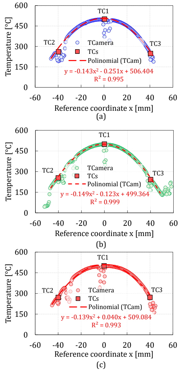
Figure 4: Spatial temperature distribution along a line passing through the mid-plane of the specimen ( y = 0 mm) (see Fig. 5) for each test: a) V1, b) V2 and c) V3.
