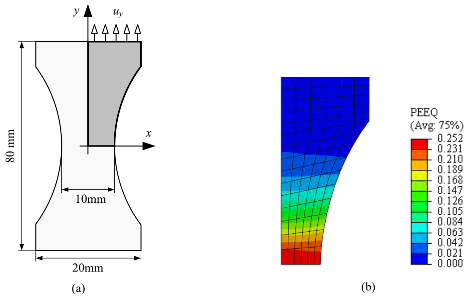
FIGURE 1. Specimen geometry (a) and corresponding finite element model (b). Equivalent Plastic strain distribution after a displacement of 3 mm
