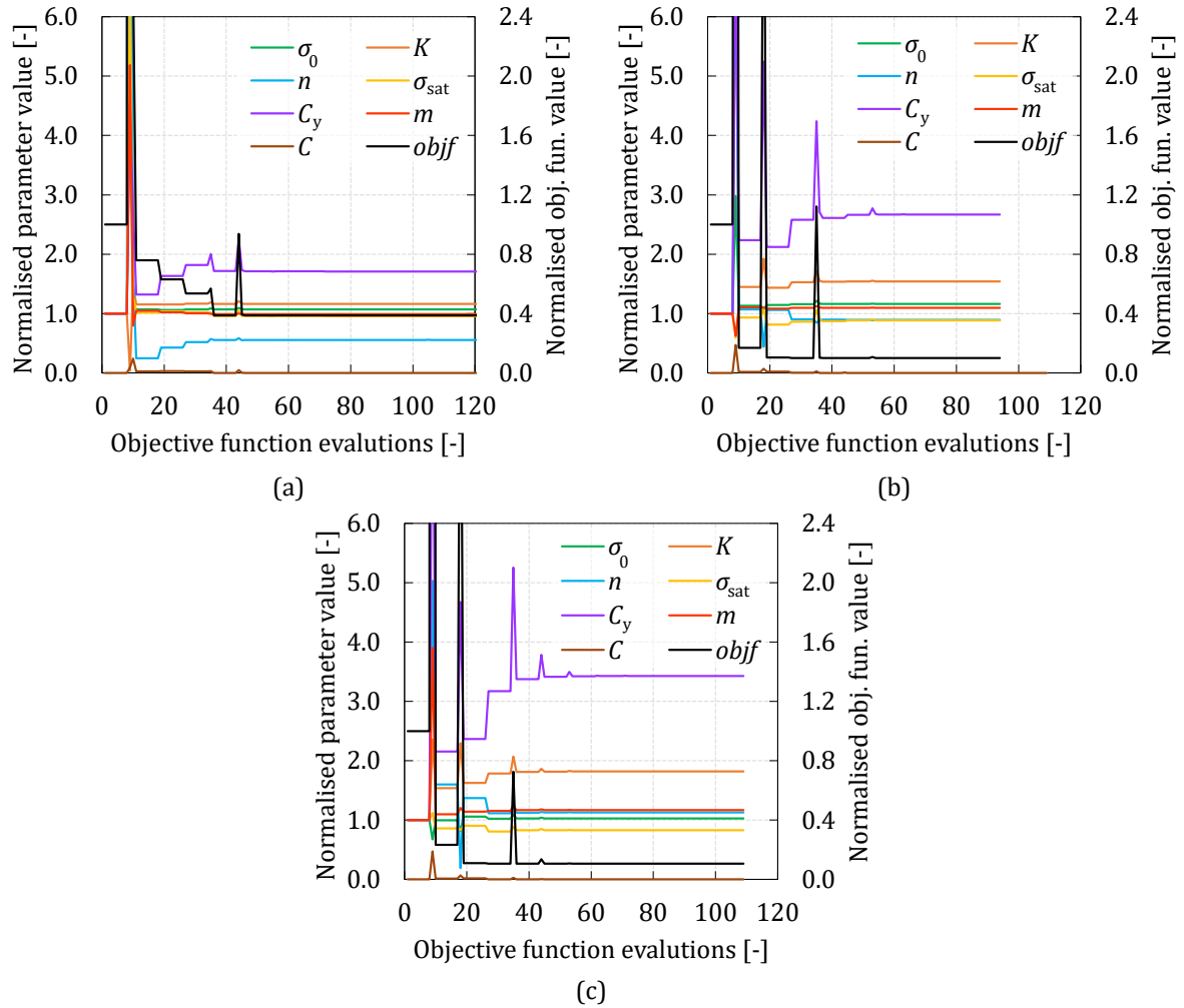
Figure 10: Evolution of the material parameters and objective function value ( objf ) during the calibration process: (a) V1, (b) V2 and (c) V3. The value of the parameters and objective function are normalised by the initial value, except for the case of the parameter C .
