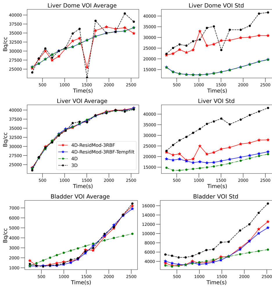
Figure 8.3: Average and standard deviation time curves of the dome of the liver the whole liver and bladder VOIs, for the comparison of 4D reconstruction with residual modelling with and without temporal filtering of residuals.
