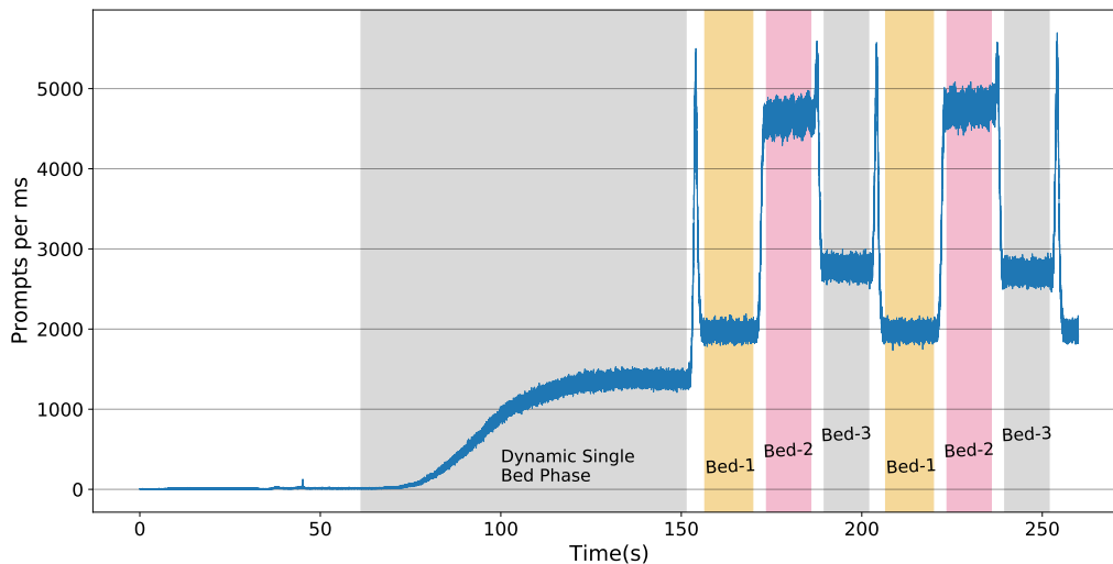
Figure 5.7: Head curve (prompts rate against time) of the acquired NHP study showing the DSB and DWB phases of the acquisition and the three DWB bed positions.
