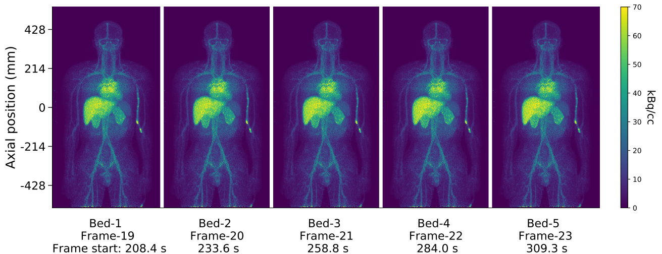
Figure 7.9: MIP image of the first whole-body pass frames from 4D reconstruction (15it28sub) of the CTRL scan.
