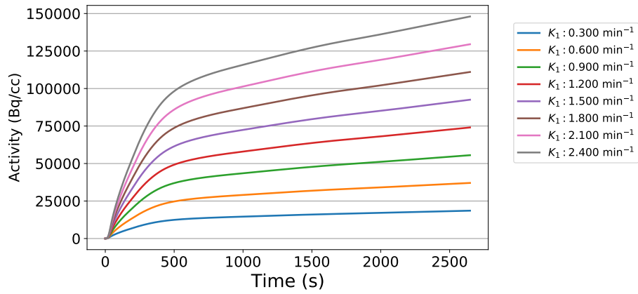
Figure C.5: Simulation of Liver TACs, using dual input function model and varying K_1 values.
