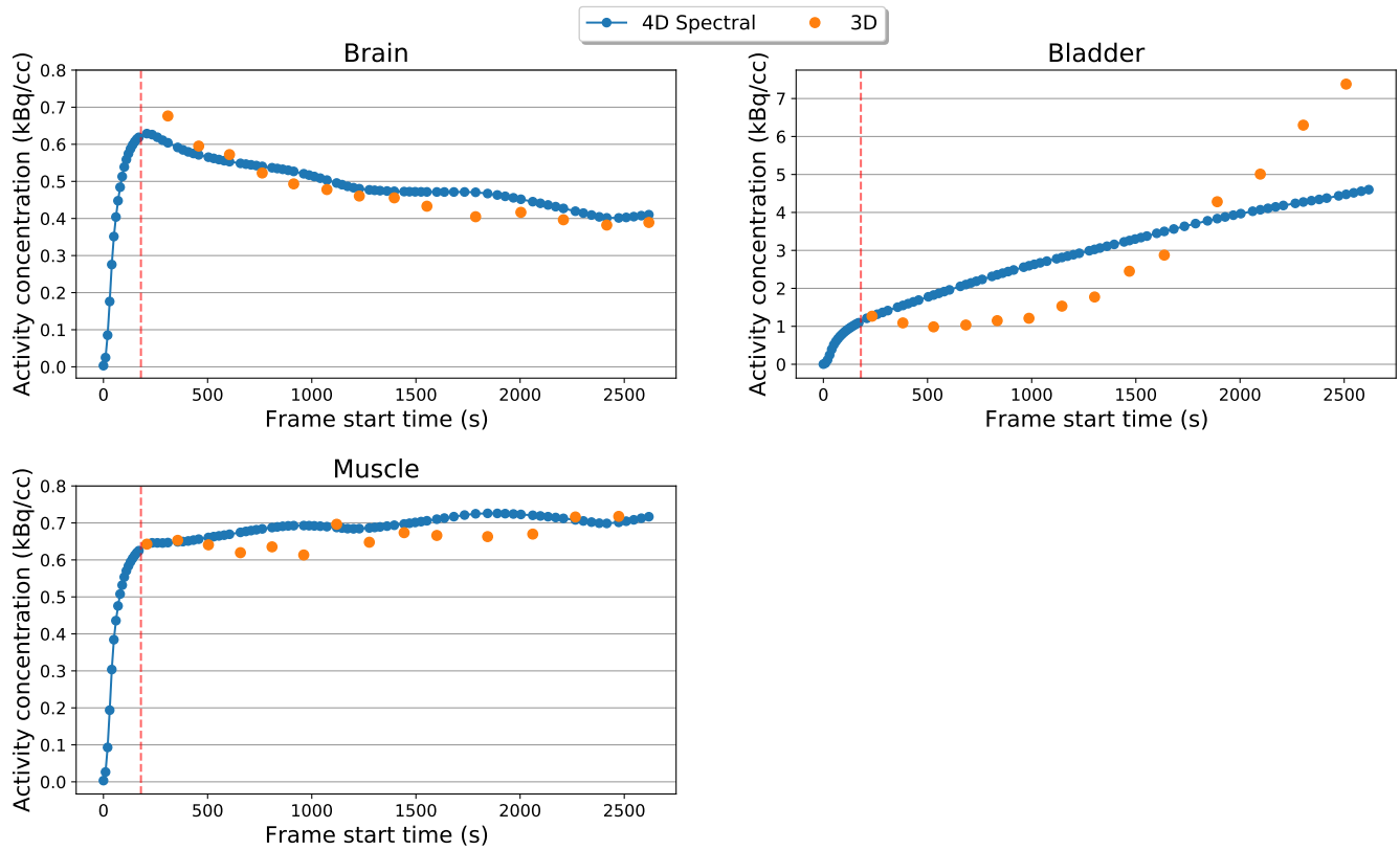
Figure 7.11: VOI mean time activity curves for 3D and 4D spectral reconstruction. VOI regions shown which are covered only by the DWB acquisition, whose start time is designated with a vertical dotted line.
