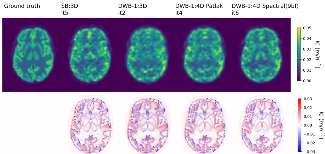
Figure 6.13: Single slice through parametric K_i images of one noise replicate (with 3mm Gaussian Filtering) (top) and their corresponding Bias images (over noise replicates) (bottom) from SB and DWB data 3D and 4D reconstructions at matched RMS CoV in the eroded thalamus.
