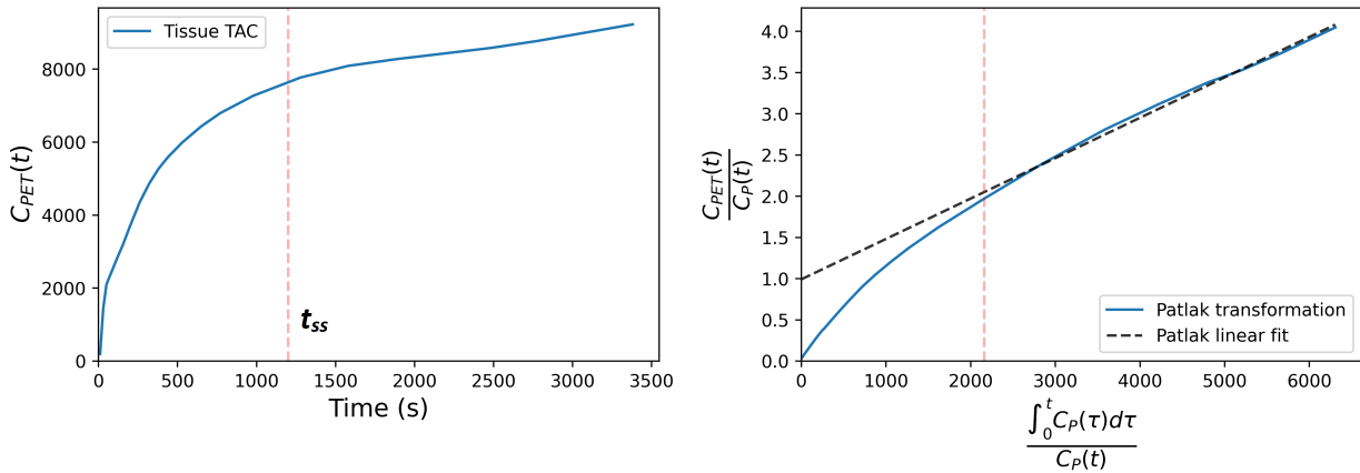
Figure 2.2: 2TCM example TAC (left) and its Patlak transformation and linear fit (right)
