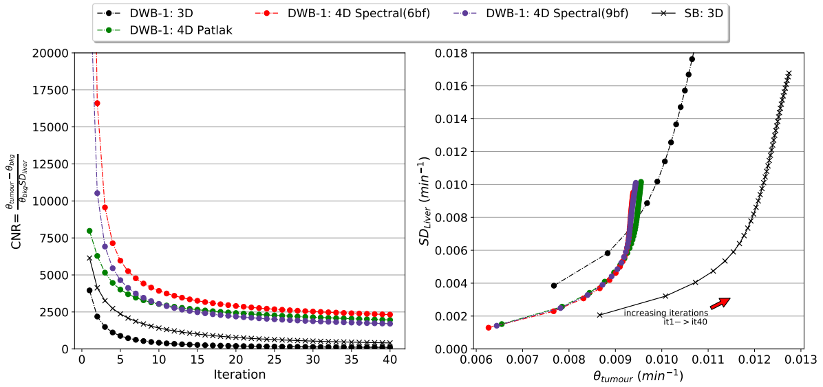
Figure 6.10: Real Data: Contrast to Noise ratio (left) and liver SD vs. VOI mean of the tumour (right) for 3D and 4D reconstructions using TOF information.
