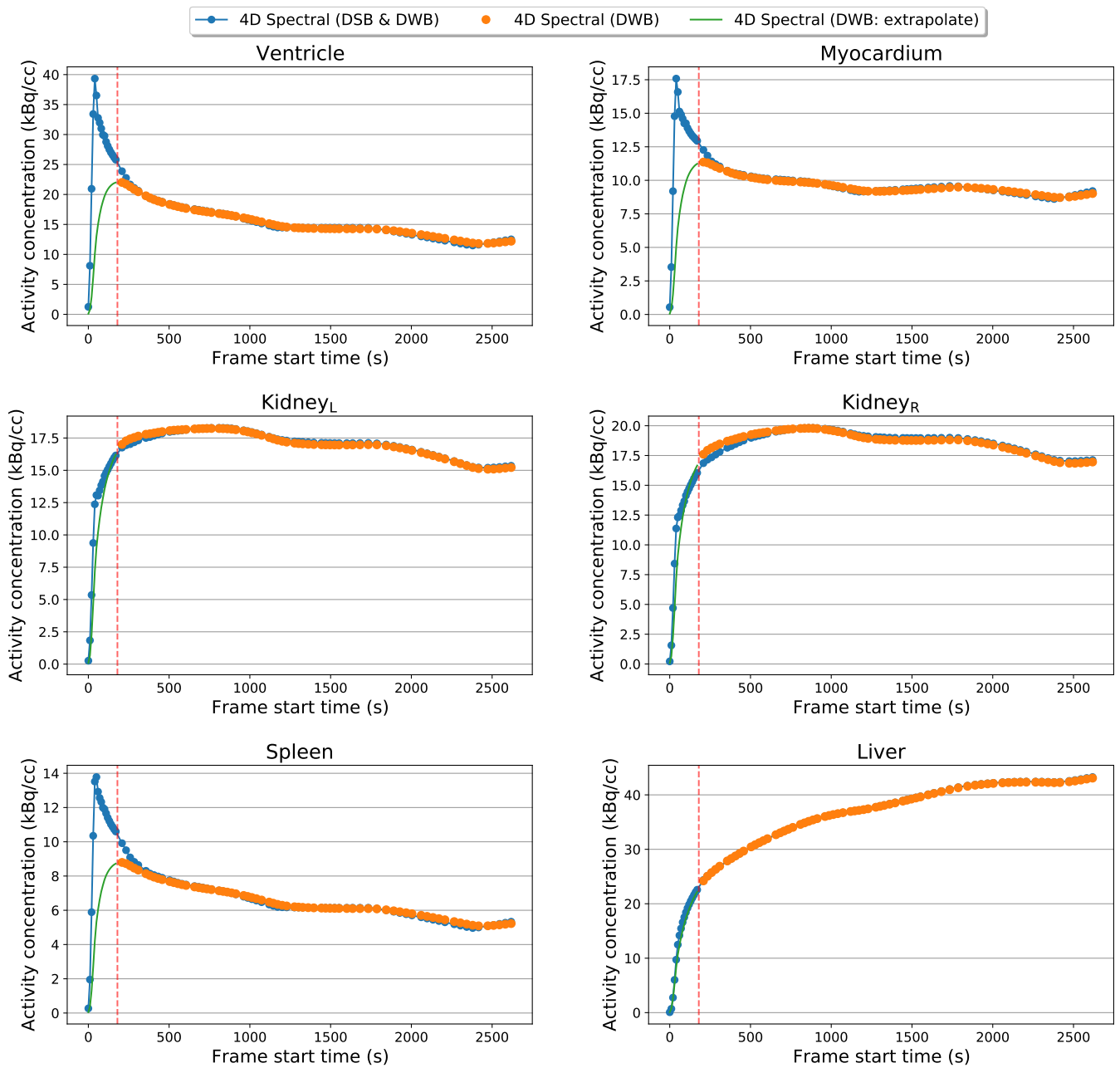
Figure 7.12: VOI mean time activity curves for 4D spectral reconstructions, with and without the use of DSB data. VOI regions shown are included in both DSB and DWB acquisitions.
