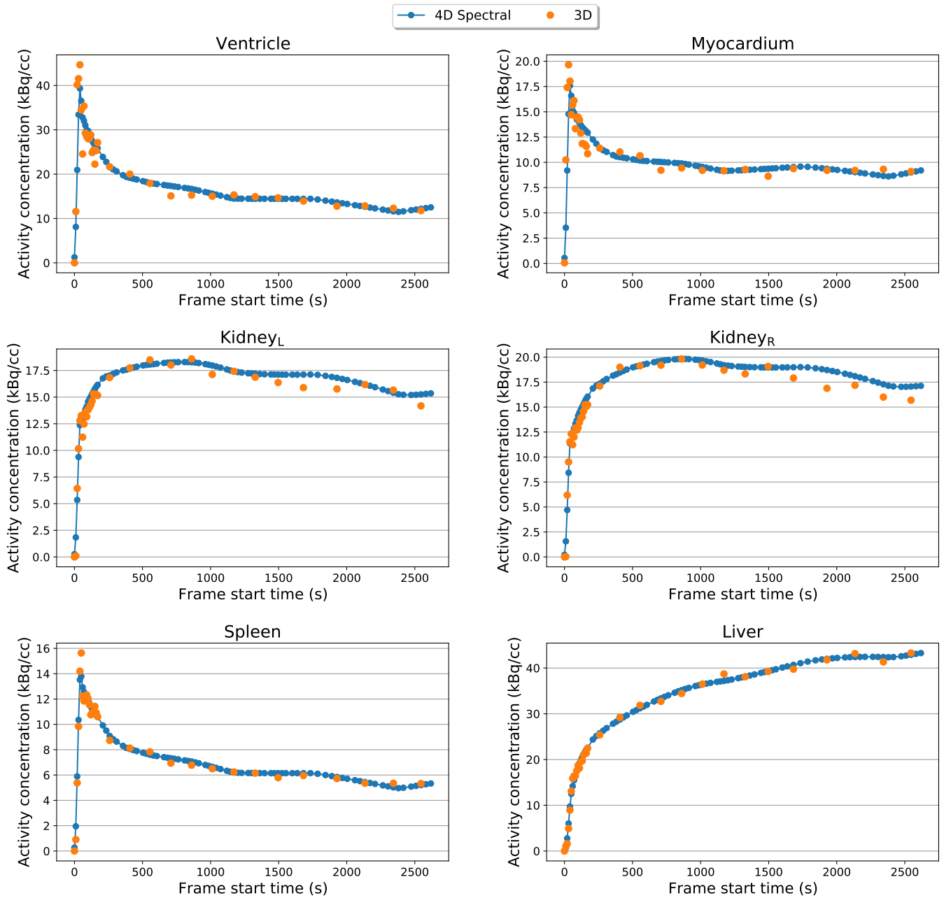
Figure 7.10: VOI mean time activity curves for 3D and 4D spectral reconstruction. VOI regions shown which are included in both DSB and DWB acquisition.
