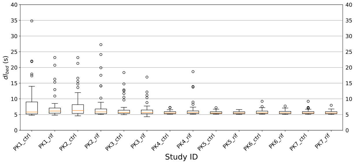
Figure 5.3: Box plots of intra-bed delays dl_{bed} of the IsotoPK DWB protocol used in practice.
