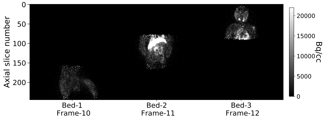
Figure 7.3: Example three frame images from a three bed DWB acquisition (NHP study of chapter 5)
