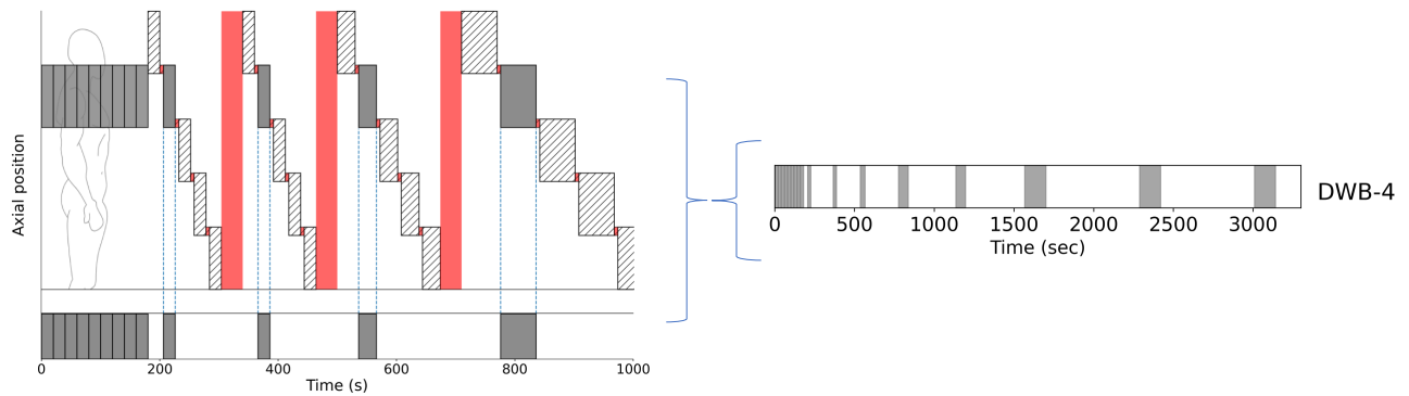
Figure 6.3: Fourth dynamic whole-body acquisition protocol considered for simulation, which includes an initial dynamic single bed phase centred over considered bed position.
