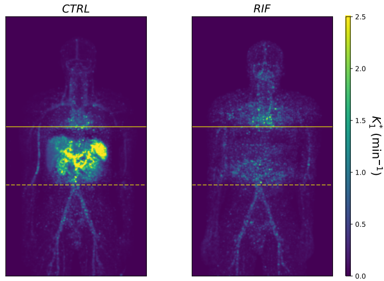
Figure 7.13: K_1 MIP images from the 4D spectral reconstruction using both DSB and DWB acquisitions, shown for the CTRL and RIF scan.
