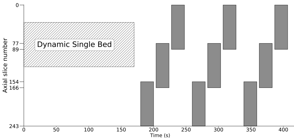
Figure 7.2: Axial slice number vs time for an example three bed positions DWB acquisition, including an initial DSB phase of 180 s.
