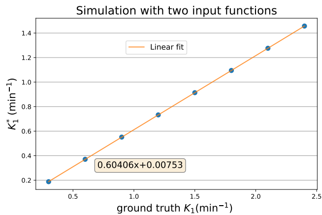
Figure C.6: Result estimates of K_1^* from spectral analysis on noiseless simulations of Liver TACs against ground truth simulated value.
