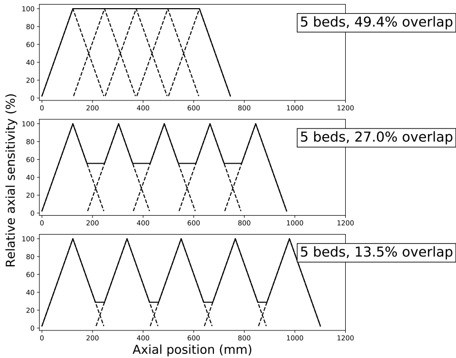
Figure 1.8: Relative axial sensitivity of 5 bed positions with decreasing overlap for the Signa PET/MR.
