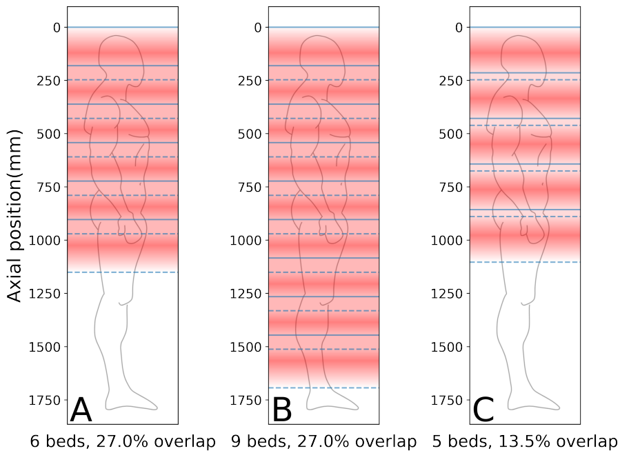
Figure 1.9: Combinations of overlap and number of bed positions for static (A&B) and dynamic whole-body imaging(C). Relative axial sensitivity is shown in shades of red, with bed start (——) and end (-----) positions.
