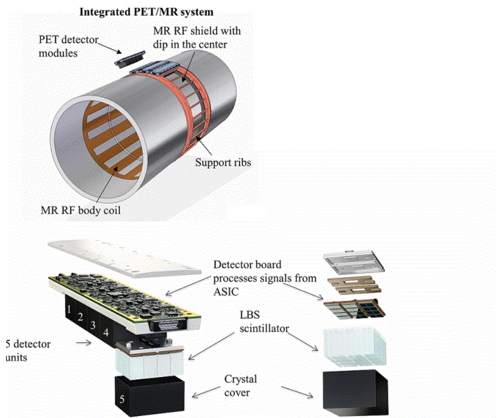
Figure 1.6: Schematic of the GE Signa hybrid PET-MR system, comprising of detector module units (bottom) in a ring formation within the MR RF body coil (top) [48].
