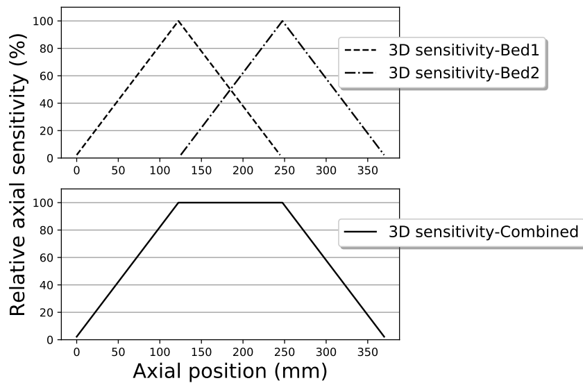
Figure 1.7: Relative axial sensitivity of individual beds (top) and combined sensitivity profile (bottom) for approximately 50% overlap for the Signa PET/MR.
