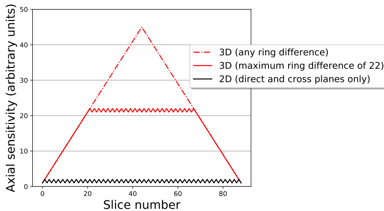
Figure 1.5: Example of 2D and 3D axial sensitivity profiles, with and without maximum ring difference limits, for a scanner with 45 crystal rings which provide 45 direct and 44 cross-planes.
