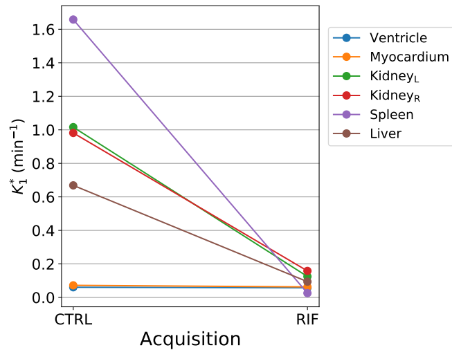
Figure 7.15: K_1^* values as estimated from the 4D spectral reconstruction for VOI regions included in both DSB and DWB acquisitions, shown for the CTRL and RIF scan
