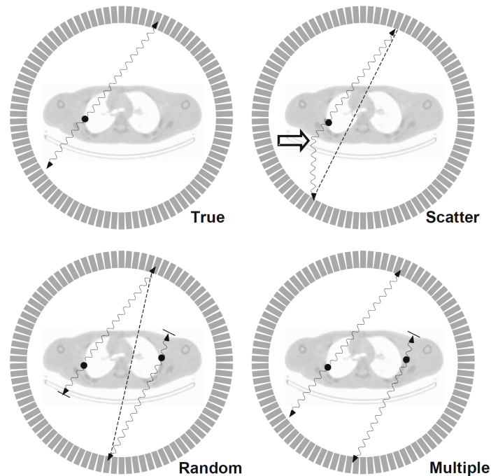
Figure 1.3: Representation of different types of detected coincidence events. Adapted from Bailey et al. [1] (Reproduced with permission).
