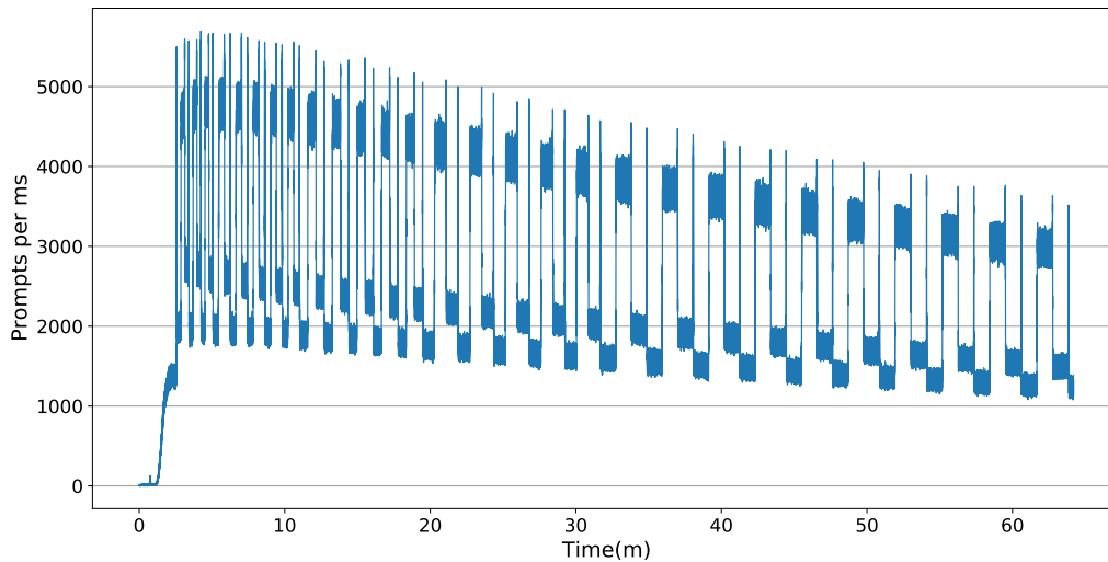
Figure 5.6: Head curve (prompts rate against time) of the acquired NHP study data in a single list-mode file using the fully-automated protocol.
