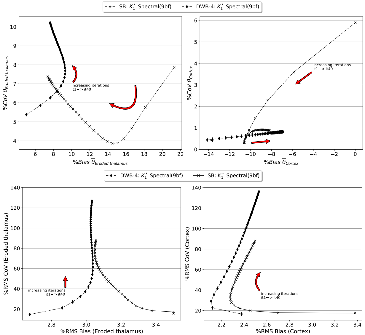
Figure 6.15: Simulation: Eroded thalamus (left) and Cortex (right) noise versus bias trade-off curves for K_1 parametric imaging from 4D spectral reconstructions of the simulated SB and DWB-4 protocol data. ROI based metrics (top row) and voxel-based metrics (bottom row).
