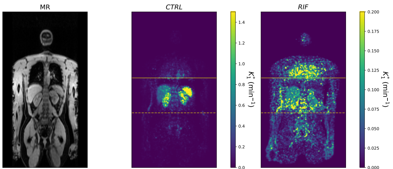
Figure 7.14: K_1^* values as estimated from the 4D spectral reconstruction for VOI regions included in both DSB and DWB acquisitions, shown for the CTRL and RIF scan
