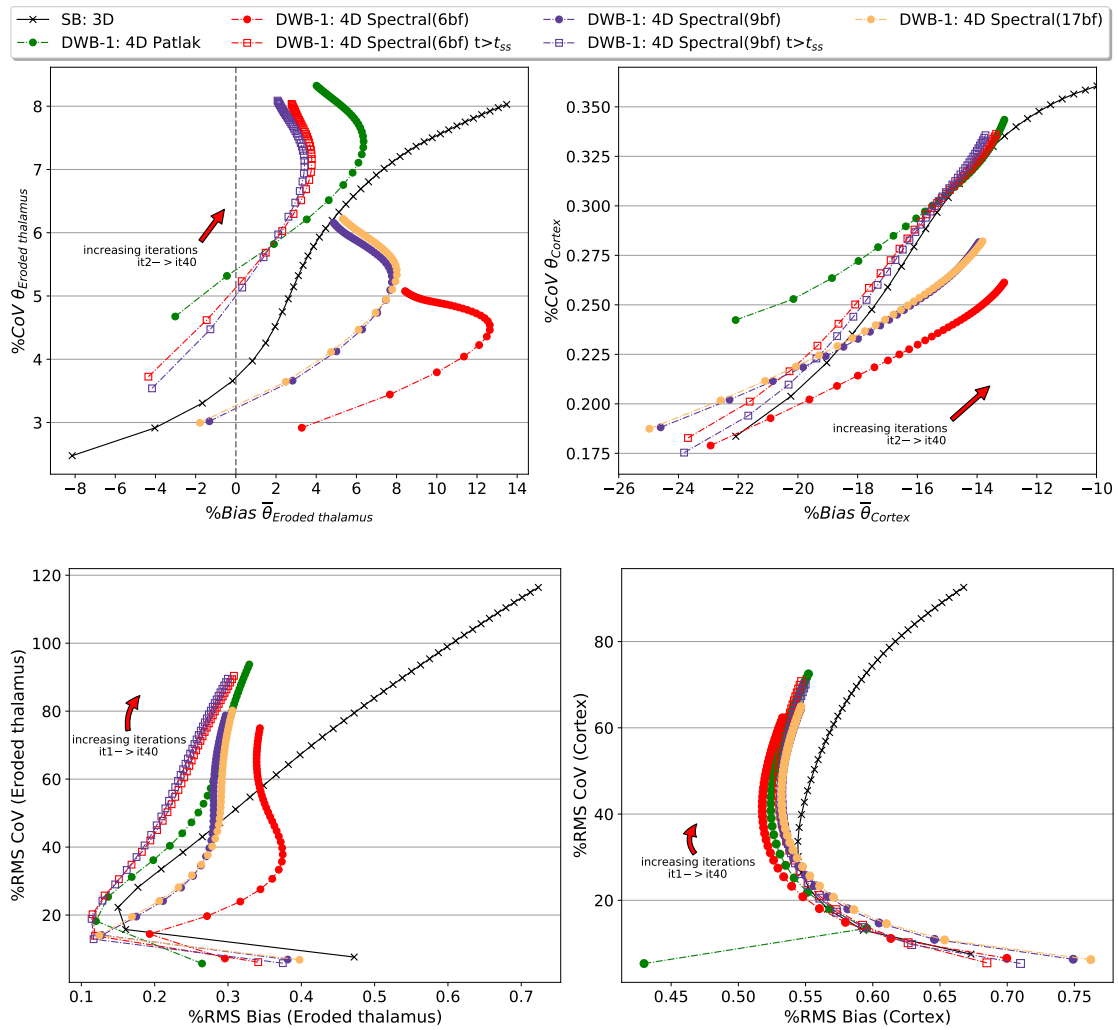
Figure 6.6: Simulation: Eroded thalamus (left) and Cortex (right) noise versus bias trade-off curves for 4D reconstructions of DWB-1 protocol data. VOI based metrics (top row) and voxel-based metrics (bottom row).
