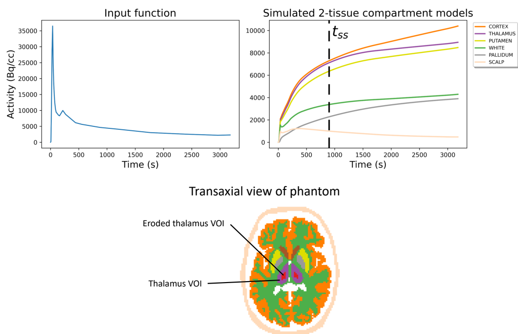
Figure B.1: Input function and selection of simulated 2-tissue compartment model TACs (top), and transaxial view of the segmented zupal phantom, with the addition of an eroded thalamus VOI (bottom). The same colours are used for the TACs and the VOIs.
