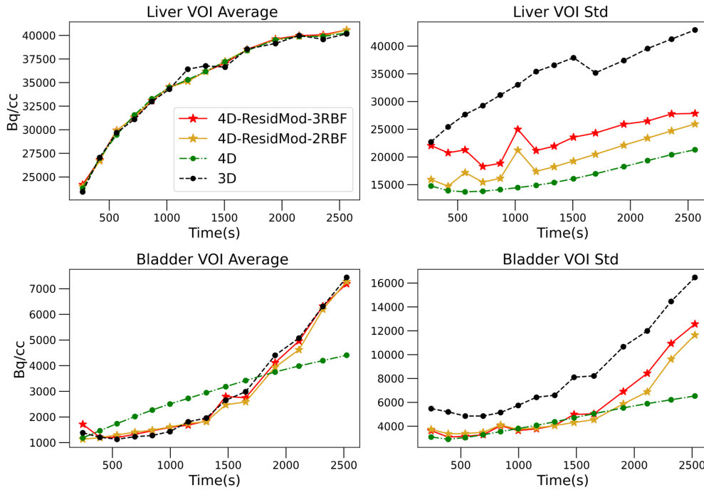
Figure 8.2: Average and standard deviation time curves of the liver and bladder VOIs, for the comparison of 3D to 4D reconstruction results as well as 4D reconstruction with residual modelling using different number of residual basis functions.
