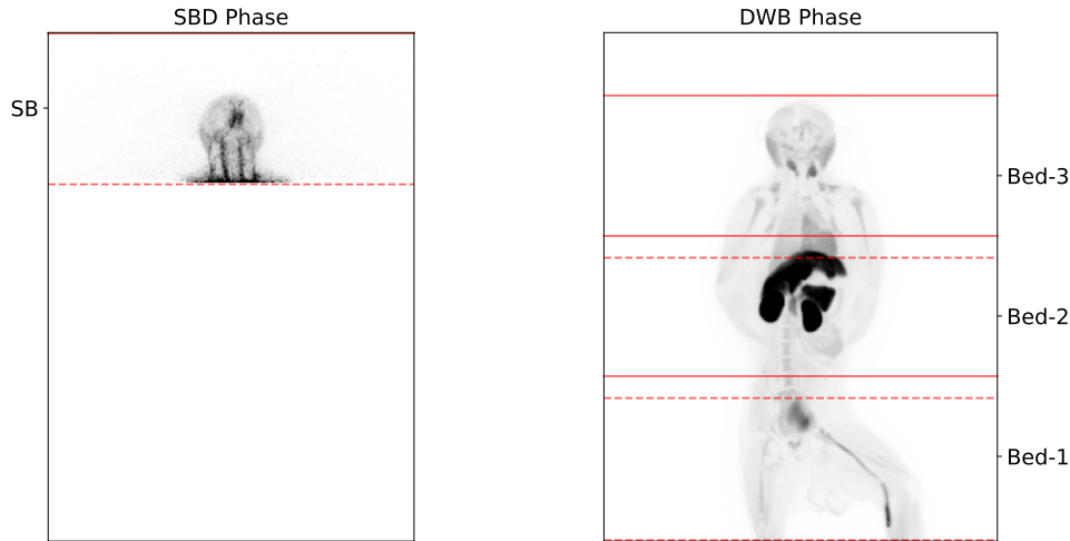
Figure 5.8: Coronal MIP views of the NHP study's reconstructed PET images, for the two phases of the acquisition, with overlay of axial bed start (—) and end (-----) location.
