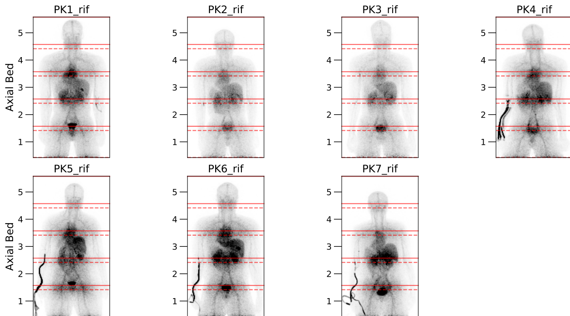
Figure 5.2: Coronal MIP projections of 7 volunteer rif DWB scans with overlay of axial bed start (—) and end (-----) location.
