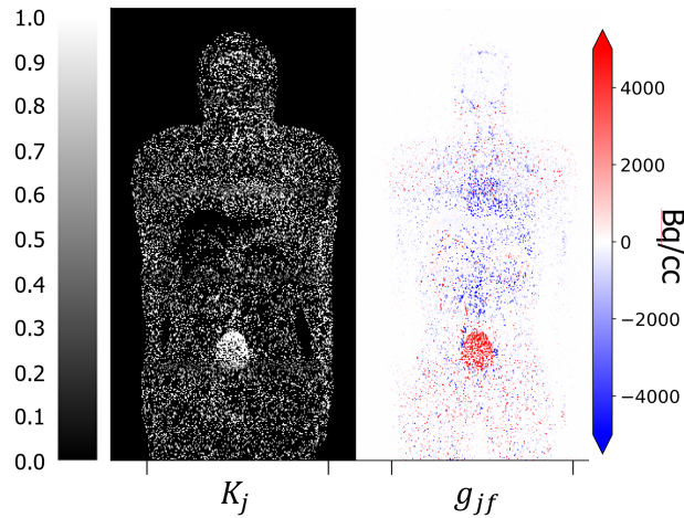
Figure 8.4: Fraction map of K_j and modelled residuals g_{jf} of the residual model 4D-ResidMod-3RBF-Tempfilt at iteration 75.
