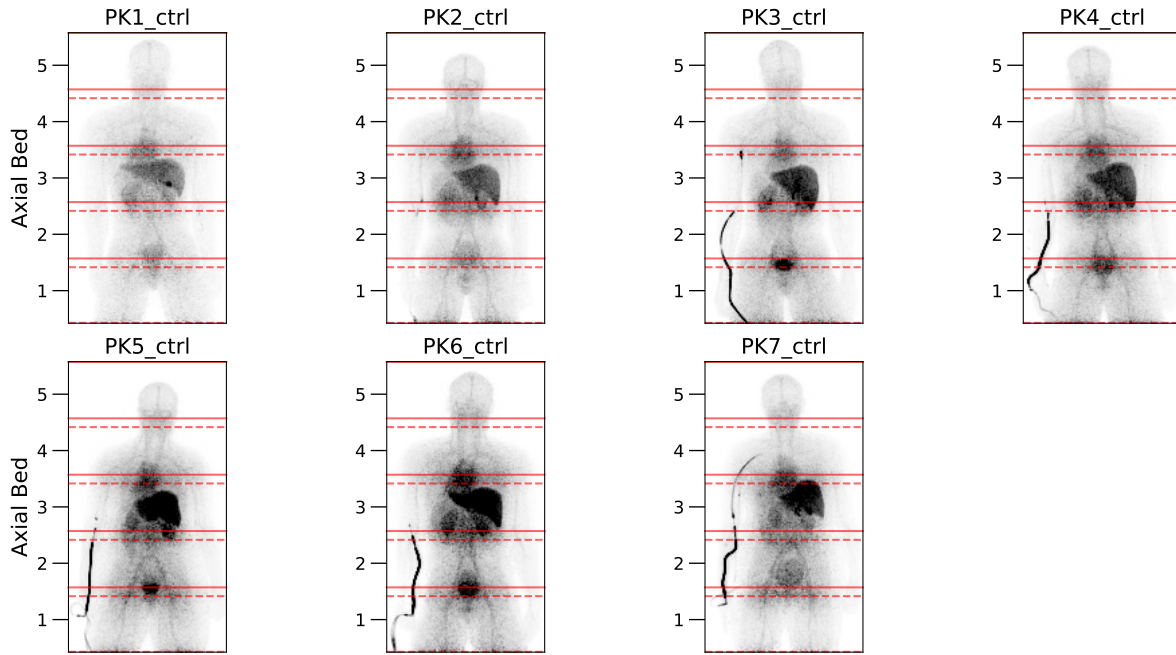
Figure 5.1: Coronal MIP projections of 7 volunteer control DWB scans with overlay of axial bed start (—) and end (-----) location.
