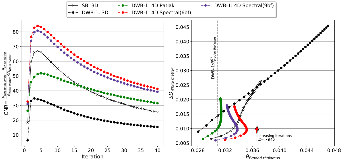
Figure 6.12: Simulation single noise realisation of DWB-1 data: Contrast to Noise ratio (left) and white matter SD vs. eroded thalamus K_i mean for 3D and 4D reconstructions.
