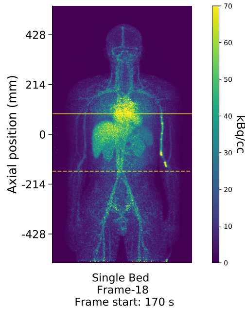
Figure 7.8: MIP image of a single frame from 4D reconstruction (15it28sub) of the CTRL scan
