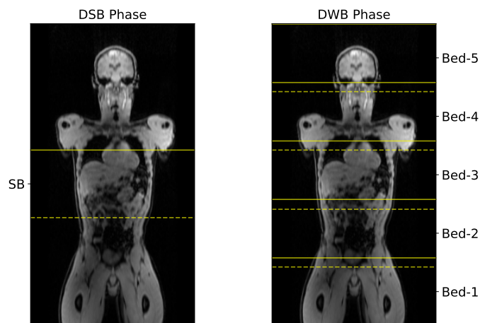
Figure 7.5: Planned DSB and DWB bed positions shown on coronal MRAC image, with bed start (——) and end (-----) positions.
