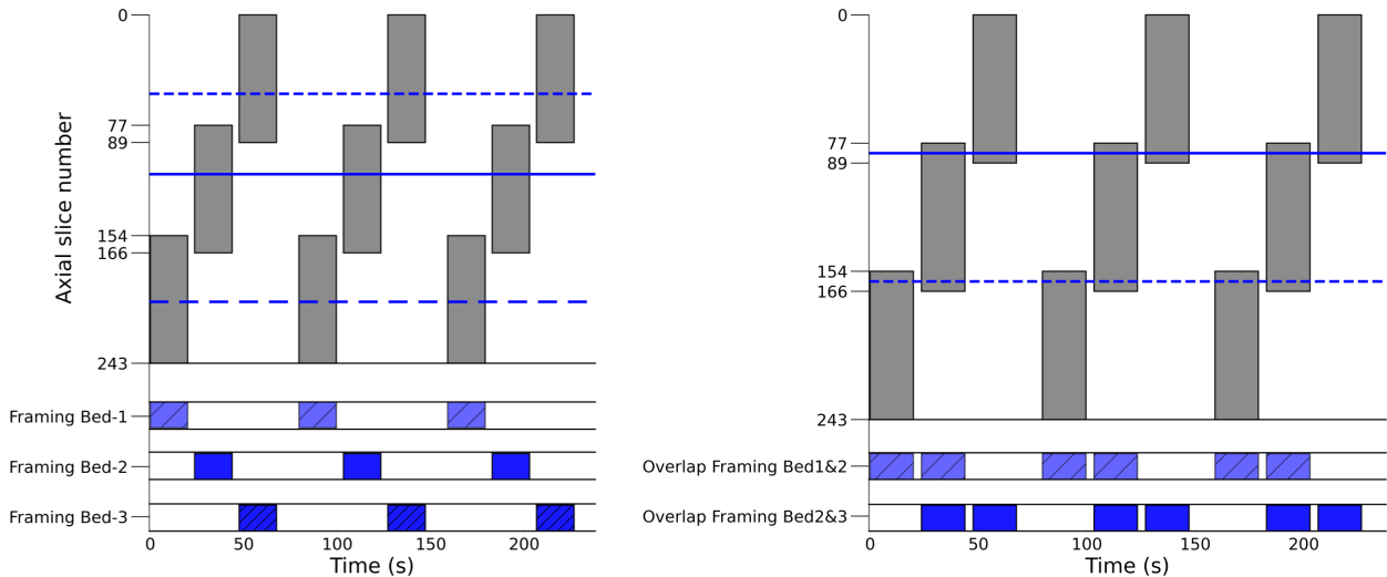
Figure 7.1: Axial slice number vs time for an example three bed positions DWB acquisition. Central axial slices (left) and slices at the overlapping regions (right) considered for the result framing.
