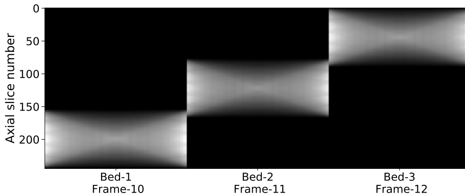
Figure 7.4: Example three frame sensitivity images from a three bed positions DWB acquisition.
