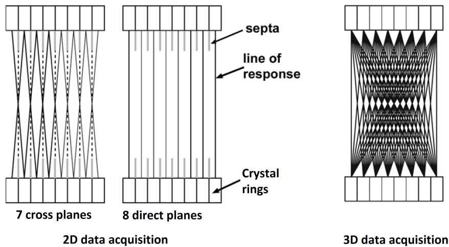
Figure 1.4: Example illustration of LORs for 2D acquisition mode using direct and cross planes (left) and 3D acquisition mode (right) for an 8 ring scanner with 15 axial slices. Adapted from Cherry S. and Magnus D. [35] (Reproduced with permission).
