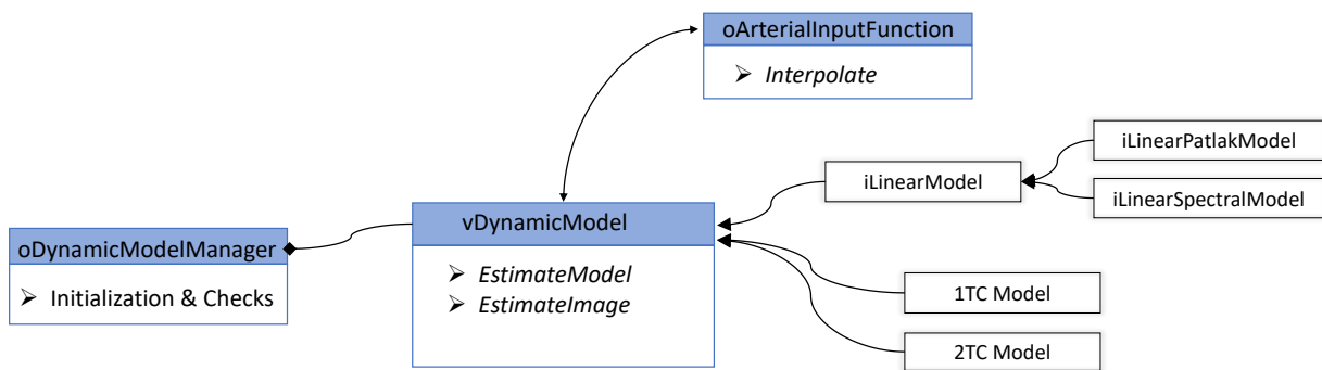
Figure 6.1: CASToR framework for dynamic reconstructions.
