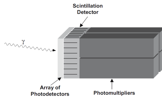
Figure 1.2: Example illustration of PMT based block detector [1] (Reproduced with permission).
