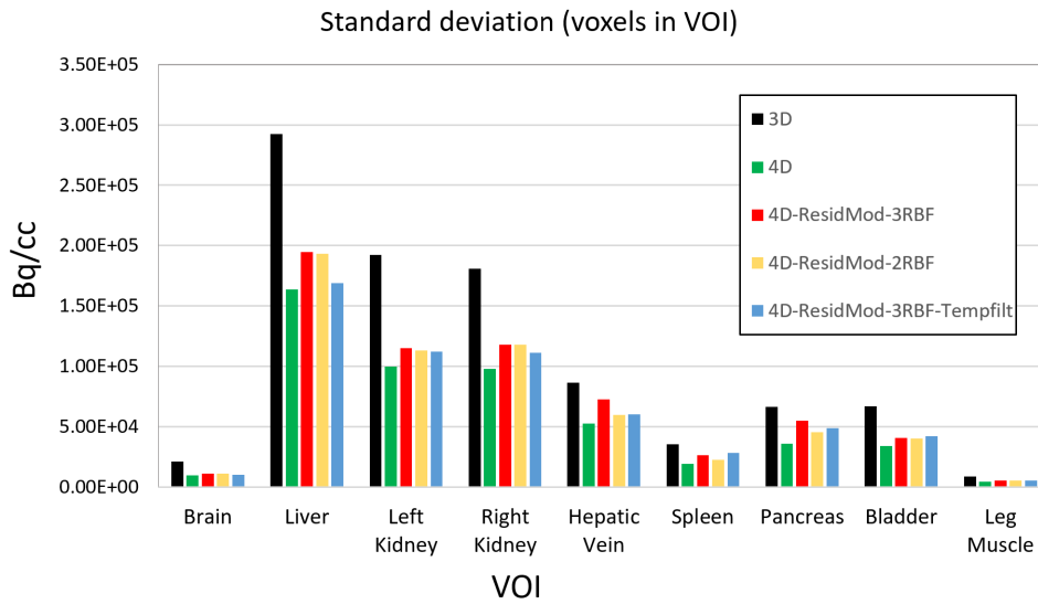
Figure 8.5: Standard deviation of VOIs for regions in the whole-body, for all evaluated reconstructions.
