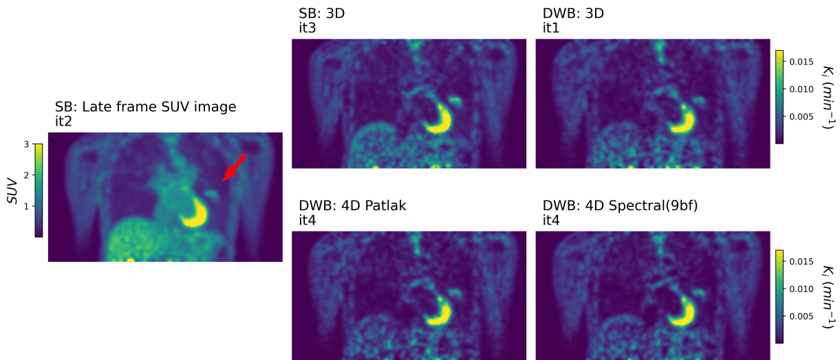
Figure 6.11: Real Data: Parametric K_i images (with 5mm Gaussian Filtering) from SB and DWB replay datasets from 3D and 4D reconstructions, using TOF information, at matched SD values over the liver.
