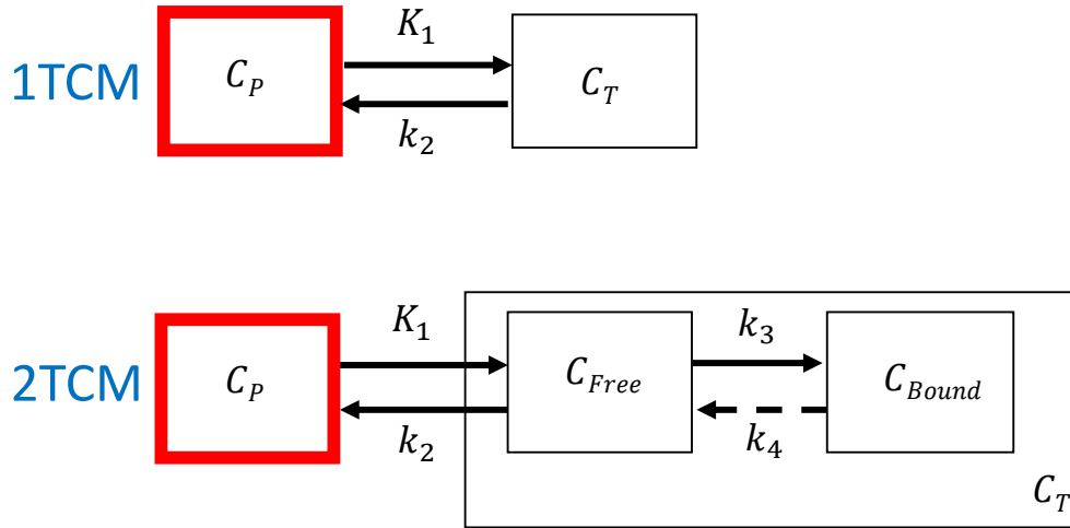
Figure 2.1: Representation of compartments and exchanges rates for 1TCM (top) and 2TCM (bottom)
