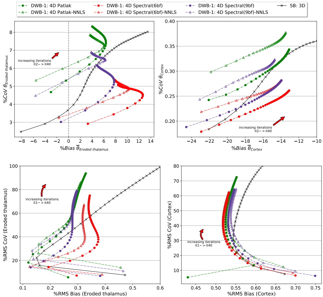
Figure 6.7: Simulation: Eroded thalamus (left) and Cortex (right) noise versus bias trade-off curves for 4D reconstructions, with MLEM and NNLS nested optimization. VOI based metrics (top row) and voxel-based metrics (bottom row).
