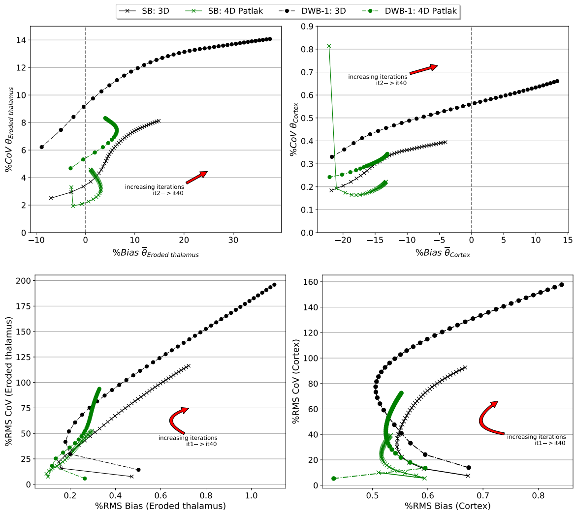
Figure 6.5: Simulation: Eroded thalamus (left) and Cortex (right) noise versus bias trade-off curves for 3D and 4D Patlak reconstructions. VOI based metrics (top row) and voxel-based metrics (bottom row).
