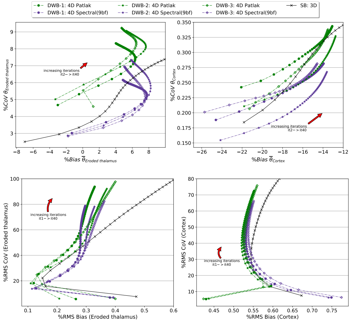
Figure 6.8: Simulation: Eroded thalamus (left) and Cortex (right) noise versus bias trade-off curves for 4D reconstructions of the simulated DWB protocol data. VOI based metrics (top row) and voxel-based metrics (bottom row).
