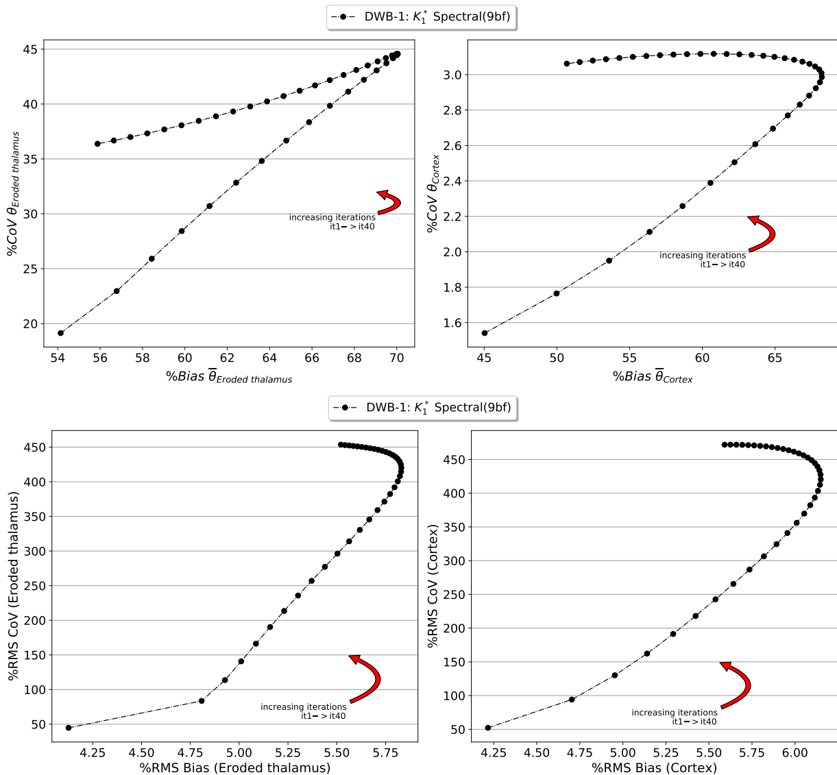
Figure 6.14: Simulation: Eroded thalamus (left) and Cortex (right) noise versus bias trade-off curves for K_1 parametric imaging from 4D spectral reconstructions of the simulated DWB-1 protocol data. VOI based metrics (top row) and voxel-based metrics (bottom row).
