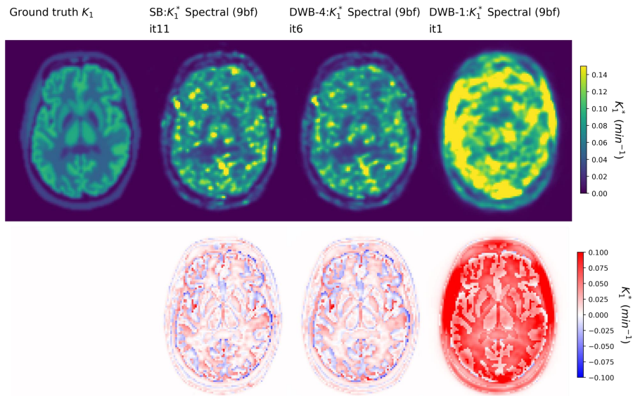
Figure 6.16: Single slice through parametric K_1^* images of one noise replicate (with 3mm Gaussian Filtering) (top) and their corresponding Bias images (over noise replicates) (bottom) from SB and DWB data, for 4D Spectral reconstructions at matched RMS CoV in the eroded thalamus.
