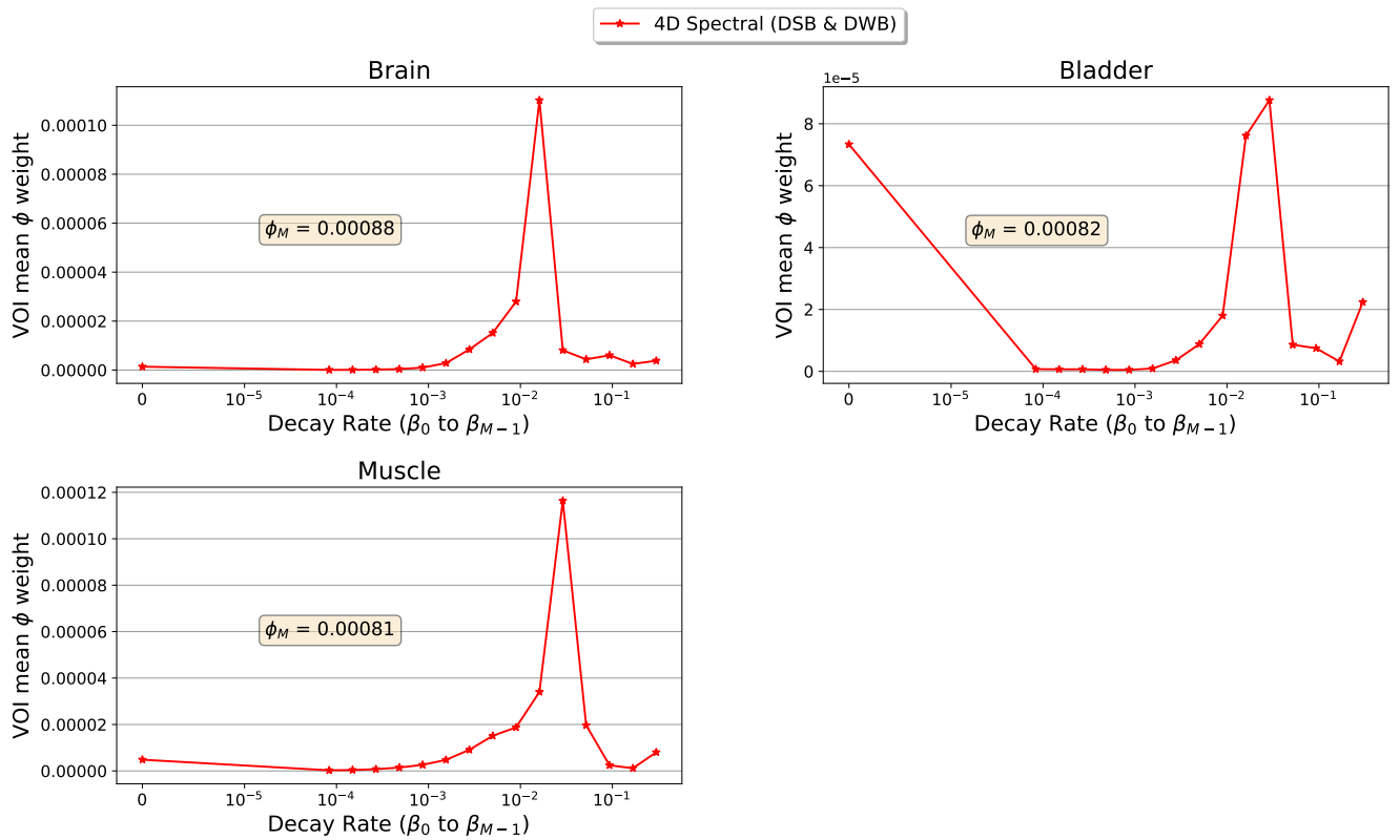
Figure C.4: Spectral model coefficients average in VOIs. VOI regions shown which are covered only by the DWB acquisition.
