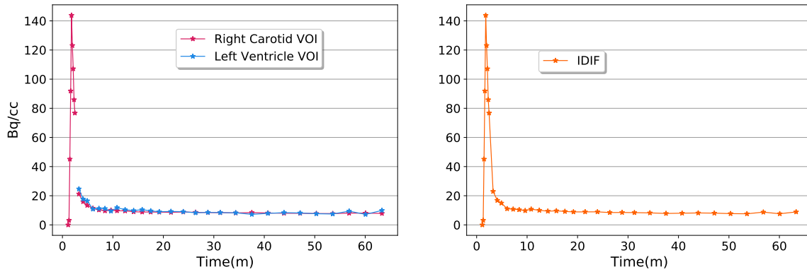
Figure 5.9: NHP study's image derived input function using information from multiple bed positions.
