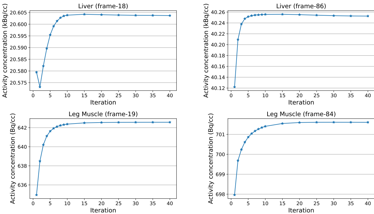
Figure C.2: Liver (top) and Muscle (bottom) VOI mean versus iteration curves for 4D spectral reconstruction. Shown for early (left) and late (right) frames of the CTRL DWB acquisition including the DSB phase.
