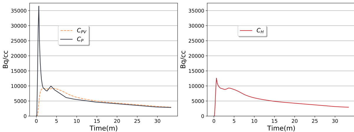
Figure 2.3: Example measured arterial input function C_P(t) and modelled PV input function (using k_g=0.5 \text{ min}^{-1} [77]) (left). Combination of arterial and PV input function to provide C_H(t) , assuming a 25/75 ratio (right).
