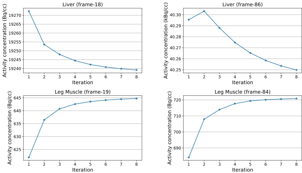
Figure C.1: Liver (top) and Muscle (bottom) VOI mean versus iteration curves for 3D reconstruction. Shown for early (left) and late (right) frames of the CTRL DWB acquisition including the DSB phase.
