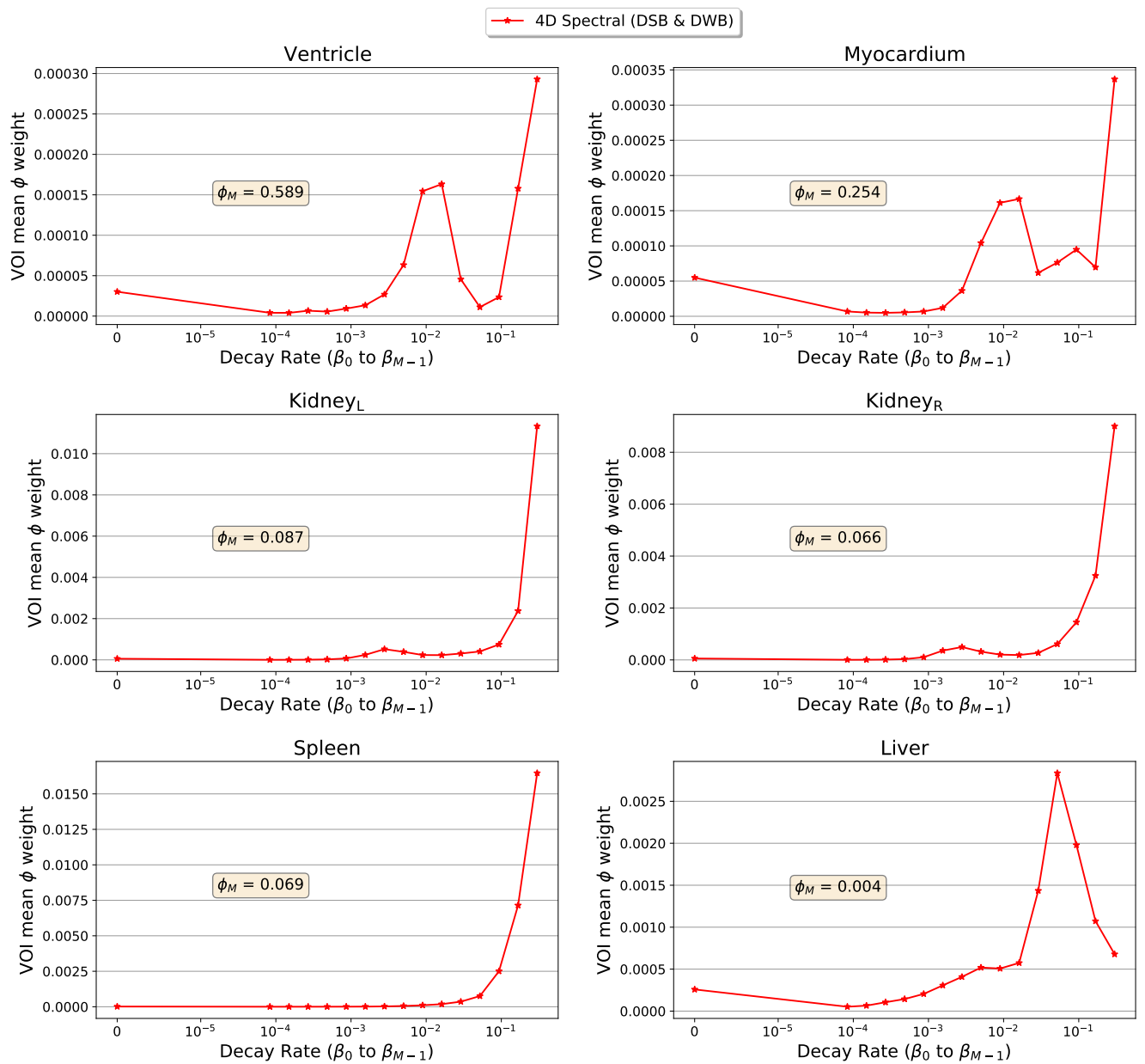
Figure C.3: Spectral model coefficients average in VOIs. VOI regions shown which are included in both DSB and DWB acquisition.
