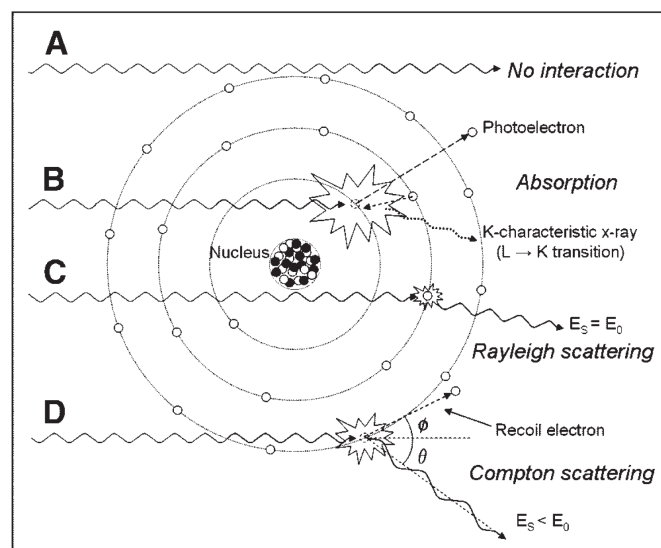
Figure 1.1: Illustration of the described interactions. (A) No interaction resulting in transmission of photon. (B) Photoelectric absorption from inner shell electron, resulting in its ejection and followed by an inner electron transition and characteristic X-Ray emission. (C) Elastic (Rayleigh) scattering conserving the energy of the photons but resulting in small angle change in direction. (D) Compton scattering with outer shell electron resulting to change of energy and direction of incident photon. Adapted from Seibert et al. [30].
