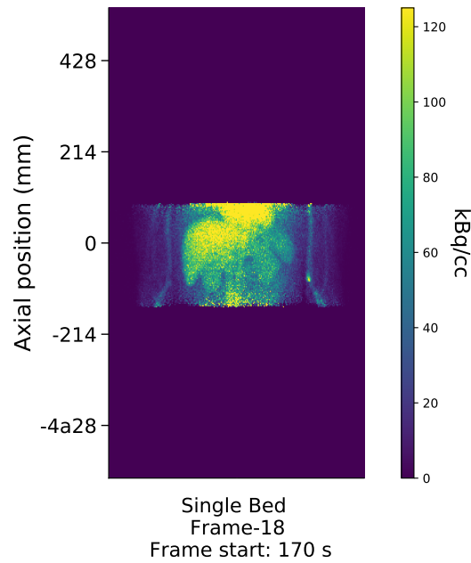
Figure 7.6: Coronal MIP image of 3D reconstruction (4it28sub) of a single frame from the DSB acquisition on the CTRL scan
