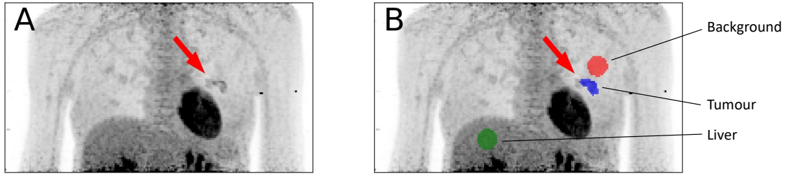
Figure 6.4: Real data MIP SUV image (A) and the drawn VOI (B).
