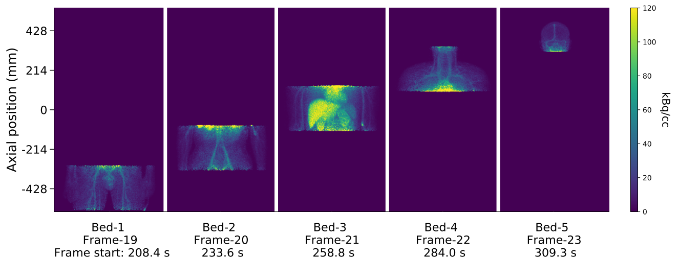
Figure 7.7: Coronal MIP images of 3D reconstructions (4it28sub) of a single frame per bed position from the first whole-body pass of the DWB acquisition on the CTRL scan.
