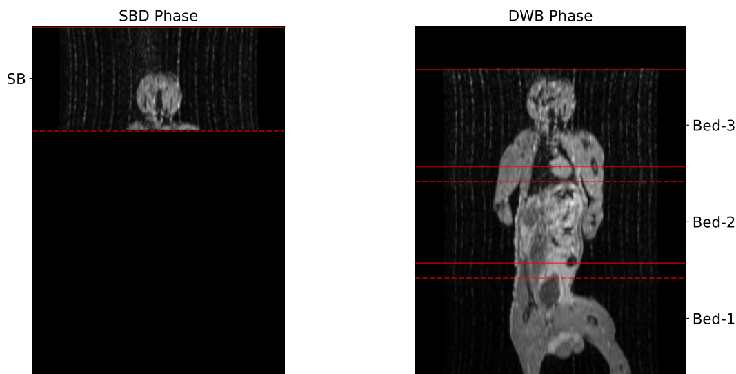
Figure 5.5: MRAC acquisitions of NHP study showing the planned bed positions of the two acquisition phases, with overlay of axial bed start (——) and end (-----) location.
