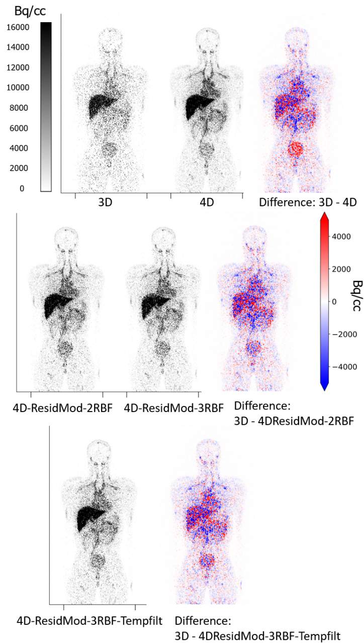
Figure 8.1: Coronal view of activity distribution from the evaluated reconstructions (frames of 41.2 to 44.1 minutes post injection). Difference images are also shown for selected cases against the 3D reconstruction.
