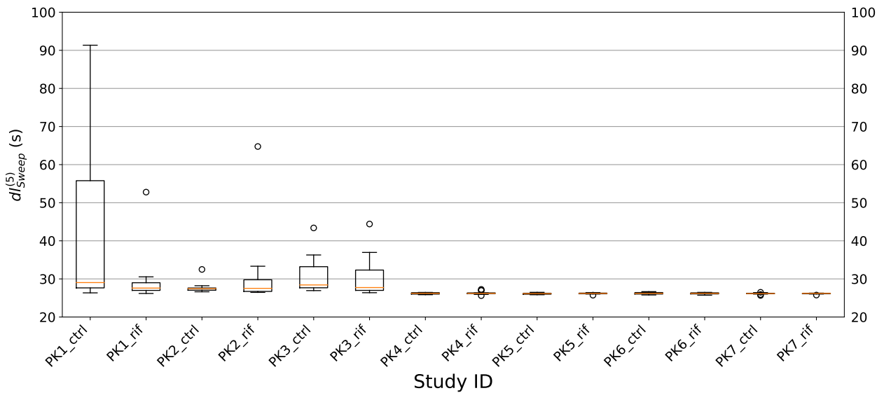
Figure 5.4: Box plots of delay between WB Sweeps dl_{Sweep} of the IsotoPK DWB protocol used in practice.
