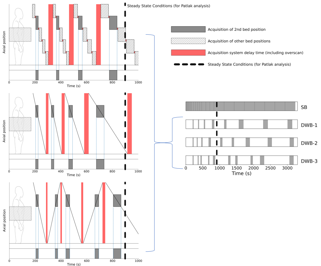
Figure 6.2: Dynamic whole-body acquisition protocols considered for simulation.
