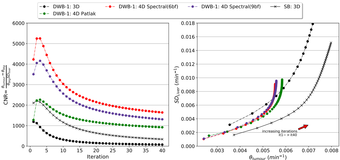
Figure 6.9: Real Data: Contrast to Noise ratio (left) and liver SD vs. VOI mean of the tumour (right) for 3D and 4D reconstructions without TOF information.
