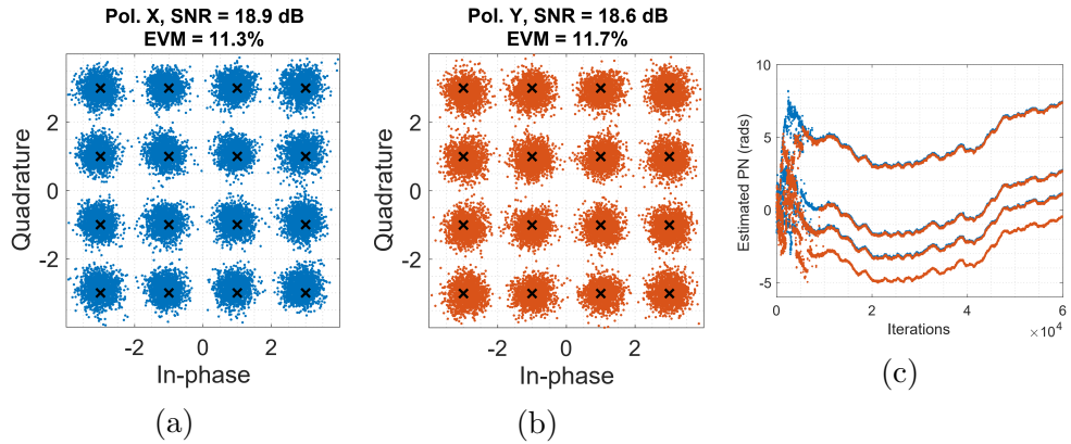
Figure 5.31 – (a) Recovered PM-16-QAM constellations using parallel BPS ( L = 4 ) at OSNR = 27.8 dB, Pol. X, (b) Pol. Y (c) Phase noise estimate.
