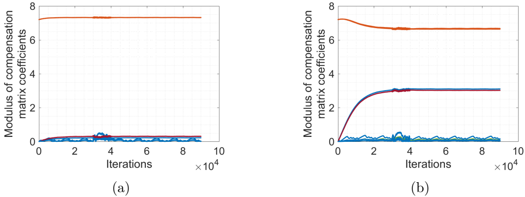
Figure 5.11 – Modulus of mixture coefficients convergence for PM-16-QAM at a 17.7 dB OSNR (a) “aligned SOPs”, (b) “arbitrary SOPs”.
