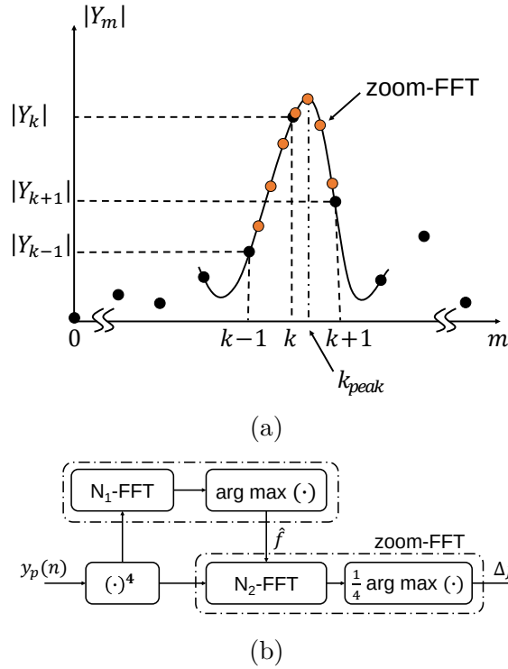
Figure 3.34 – (a) N_1 -FFT and zoom-FFT magnitude samples of a spectral tone. (b) Schematic diagram of zoom-FFT.
