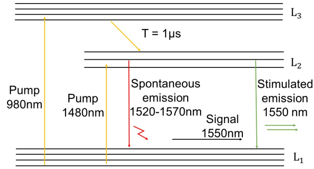
Figure 3.2 – Transitions involved in EDFA amplification.
