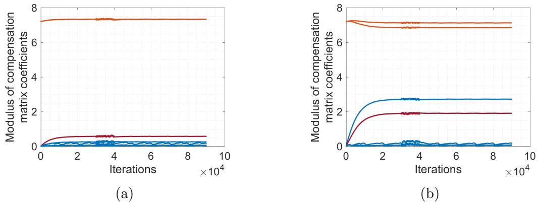
Figure 5.8 – Modulus of mixture coefficients convergence for PM-4-QAM (a) “aligned SOPs”, (b) “arbitrary SOPs”.
