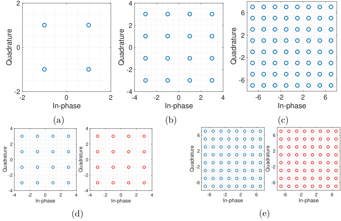
Figure 2.5 – Examples of modulation formats commonly used in coherent optical communications. (a) quadrature phase shift keying (QPSK), or alternatively, 4-ary QAM (4-QAM), 2 bit/symbol, (b) 16-QAM, 4 bit/symbol, (c) 64-QAM, 6 bit/symbol, (d) PM-16QAM, 8 bit/symbol, (e) PM-64QAM, 12 bit/symbol.
