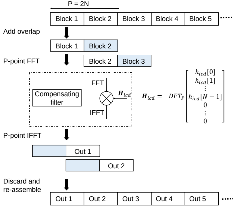
Figure 3.27 – Frequency domain CD compensation using the method overlap-save.
