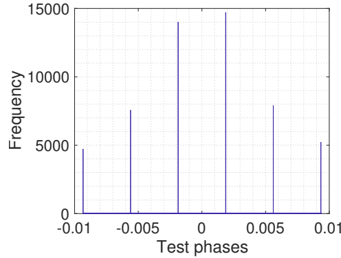
Figure 5.21 – Number of occurrence of each test phase for carrier phase compensation.
