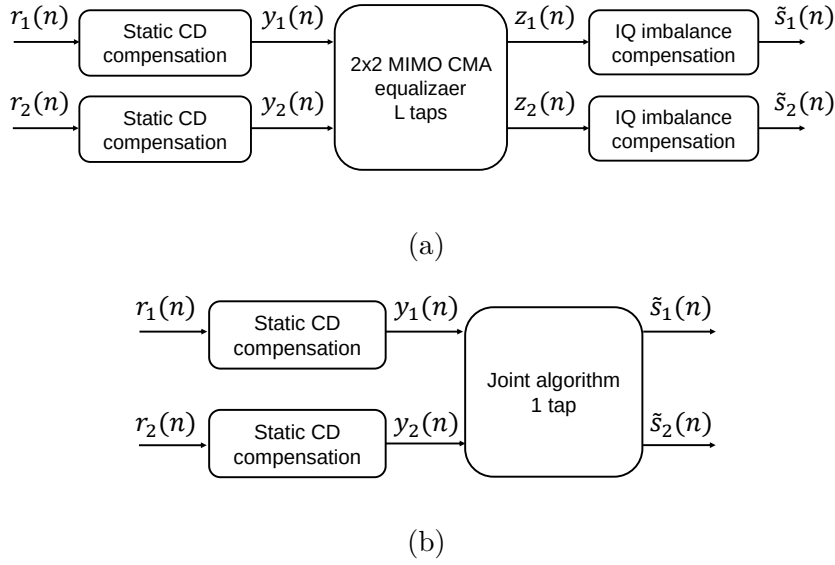
Figure 4.13 – Diagram of residual CD compensation (a) using L taps of 4 FIR filters (b) using the joint algorithm.
