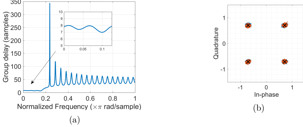
Figure 4.12 – 32 Gbaud PDM-4-QAM signals ( \text{DGD} = 30 ps, E_s/N_0 = 30 dB, \alpha = 30^\circ , \theta = 50^\circ , \epsilon_{p,Tx} = 0.1 and \varphi_{p,Tx} = 6^\circ ) (a) group delay of the resulted Wiener filter, (b) signals after cascaded Wiener filter and the joint algorithm.
