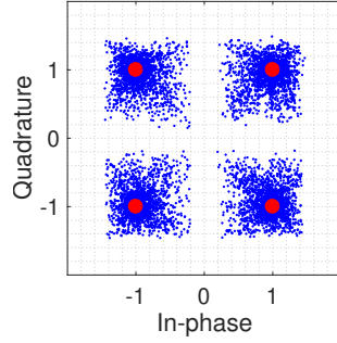
(a) QPSK corrupted with timing offset
