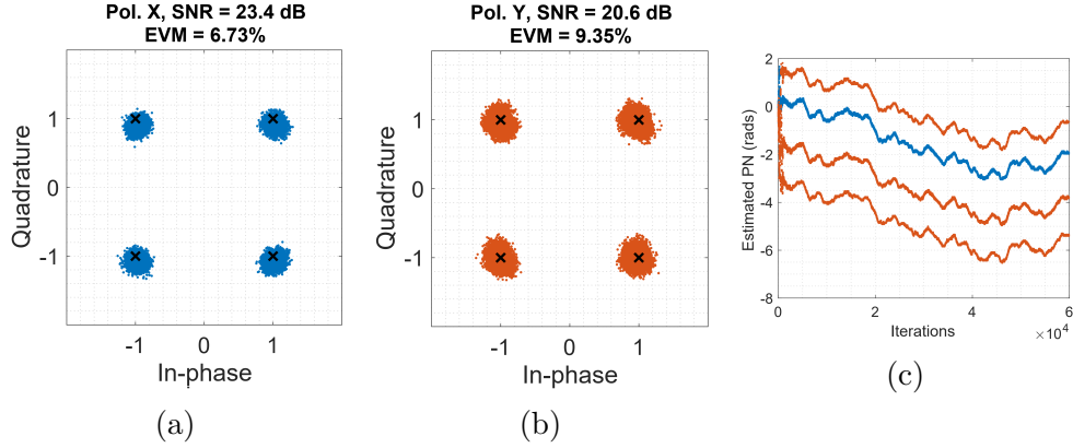
Figure 5.26 – (a) Recovered PM-4-QAM constellations using parallel BPS ( L = 4 ) at OSNR = 27.8 dB, Pol. X, (b) Pol. Y (c) Phase noise estimate.
