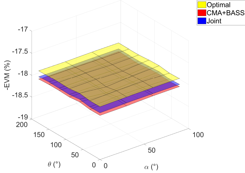
Figure 4.6 – Average -EVM surfaces as a function of the polarization rotation parameters with 16-QAM modulation ( E_s/N_0 = 15 dB, \epsilon_{p,Tx} = 0.1 , \varphi_{p,Tx} = 6^\circ ).
