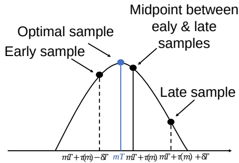
Figure 3.15 – Feedback timing recovery scheme.
