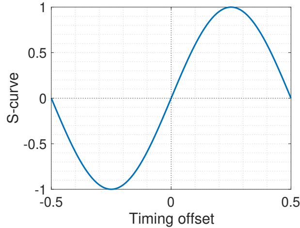
Figure 3.16 – S-curve for the non-data aided early-late timing error detector.
