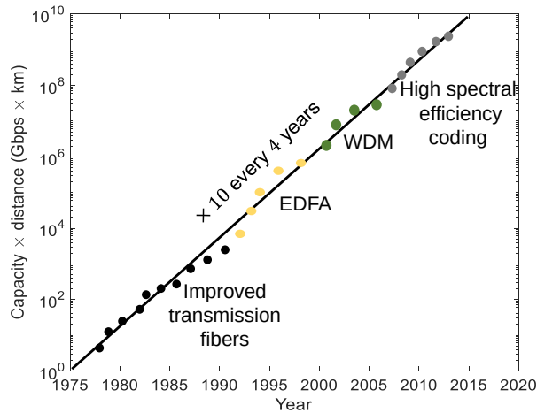
Figure 1.3 – Evolution of optical transmission systems, inspired from [15]
