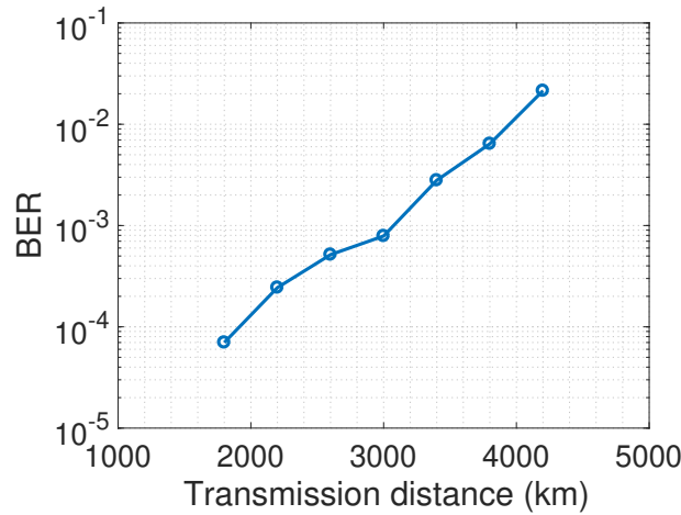
Figure 5.5 – BER vs transmission distance for 35.8 dB received OSNR.
