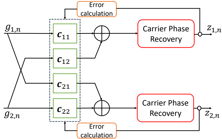
Figure 3.50 – Joint PMD compensation and carrier phase recovery.
