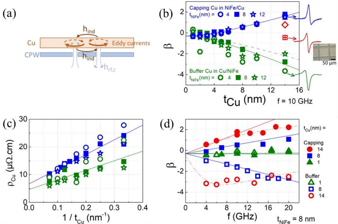
Figure 11 : (a) Illustration of a mechanism where the inhomogeneous field ( h_{\text{rf}} ) of the coplanar waveguide, with strong out-of-plane components, generates eddy currents with oppositely directed induced in-plane fields ( h_{\text{ind}} ) above and below a Cu layer. (b) Representative series of dependences of \beta on ‘capping’ and ‘buffer’ Cu-layer thickness ( t_{\text{Cu}} ) for Si/SiO 2 /Cu( t_{\text{Cu}} )/NiFe( t_{\text{NiFe}}=4;8;12 )/Al(2)O x and Si/SiO 2 /NiFe( t_{\text{NiFe}}=4;8;12 )/Cu( t_{\text{Cu}} )/Al(2)O x (nm) stacks. Data were recorded at 10 GHz. The square crossed symbol corresponds to data recorded after patterning (inset) the Cu(14)/Al(2)O x bilayer in a Si/SiO 2 /NiFe(8)/Cu(14)/Al(2)O x (nm) stack. The open square symbol corresponds to data for the same stack on which the whole etching process was performed, as these samples were protected by a resist they remained unpatterned. (c) Corresponding dependences of Cu-layer resistivity ( \rho_{\text{Cu}} ) on t_{\text{Cu}} , obtained separately using standard 4-point electrical measurements. The lines were obtained using linear fits. (d) Representative series of dependences of on frequency ( f ) for Si/SiO 2 /Cu( t_{\text{Cu}}=1;8;14 )/NiFe(8)/Al(2)O x and Si/SiO 2 /NiFe(8)/Cu( t_{\text{Cu}}=1;8;14 )/Al(2)O x (nm) stacks. The straight lines in (b) and (d) were obtained using Eq. 1-19. The dashed and dash-dotted lines are visual guides.
